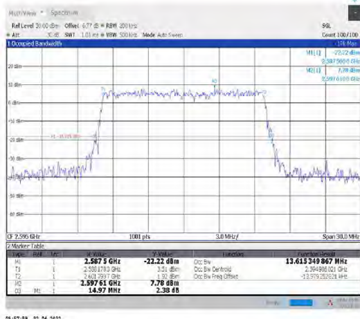
1-N38--30-15-M-9-CP-256QAM-Outer_Full-38@0- Ant1-13.615-14.970-≤15-PASS
