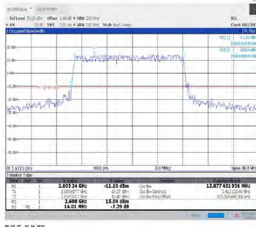
1-N38--30-15-H-1-DFT-QPSK-Outer_Full-36@0- Ant1-12.877-14.010-≤15-PASS
