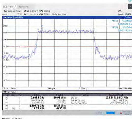
1-N38--30-15-H-2-DFT-PI2BPSK-Outer_Full-36@0- Ant1-12.834-14.130-≤15-PASS
