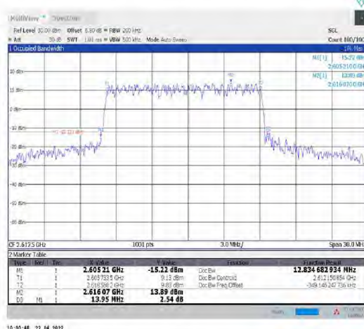
1-N38--30-15-H-3-DFT-16QAM-Outer_Full-36@0- Ant1-12.835-13.950≤15-PASS
