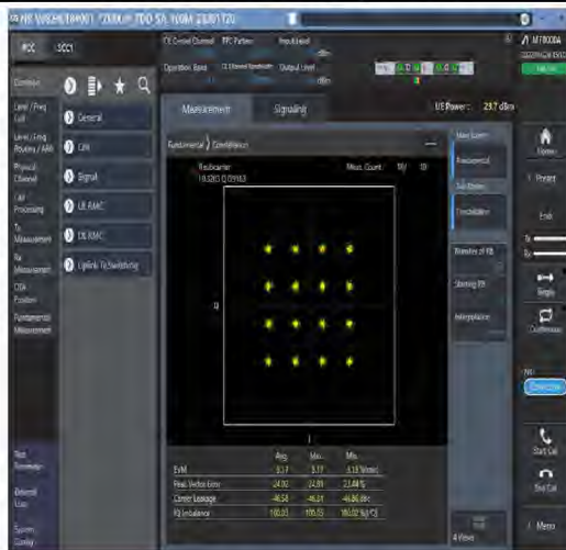
1-N41--30-100-M-7-CP-16QAM-Outer_Full-273@0-Ant1-see graph-PASS
