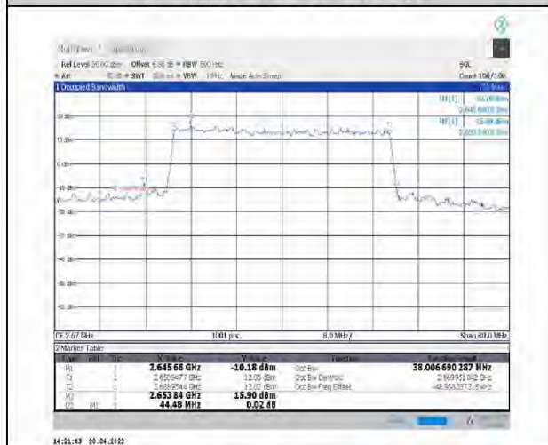
1-N41--30-40-H-7-CP-16QAM-Outer_Full-106@0- Ant1-38.007-44.480-≤40-PASS
