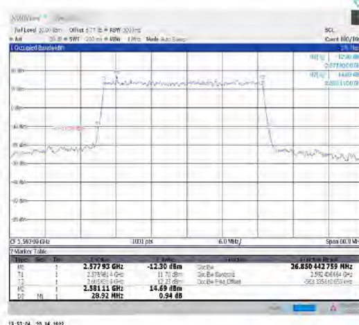
1-N41--30-30-M-4-DFT-64QAM-Outer_Full-75@0- Ant1-26.85-28.920-≤30-PASS
