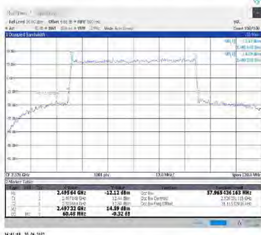
1-N41--30-60-L-3-DFT-16QAM-Outer_Full-162@0- Ant1-57.965-60.480-≤60-PASS
