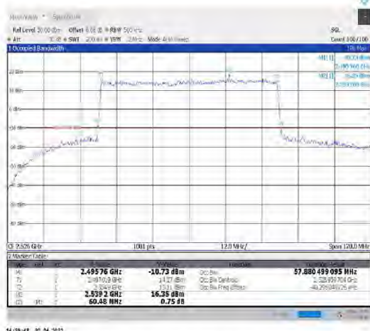
1-N41--30-60-L-1-DFT-QPSK-Outer_Full-162@0- Ant1-57.88-60.480-≤60-PASS
