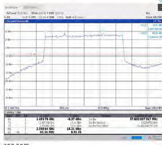
1-N41--30-60-L-2-DFT-PI2BPSK-Outer_Full-162@0- Ant1-57.853-60.360-≤60-PASS
