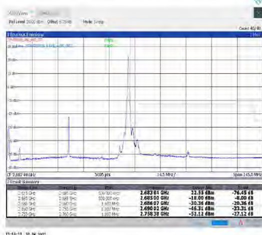
1-N41--30-70-H-5-CP-QPSK-Edge_1RB_Right- 1@188-Ant1-PASS-see graph
