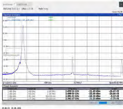
1-N41-PC2-30-70-L-4-CP-QPSK-Edge_1RB_Left- 1@0-Ant2-PASS-see graph
