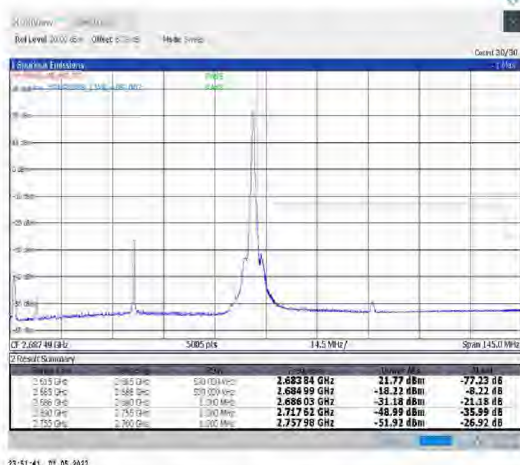
1-N41-PC2-30-70-H-5-CP-QPSK-Edge_1RB_Right- 1@188-Ant2-PASS-see graph
