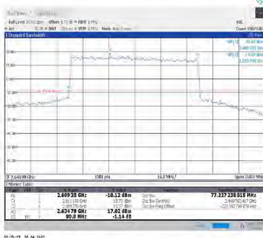
1-N41--30-80-H-3-DFT-16QAM-Outer_Full-216@0- Ant1-77.227-80.800-≤80-PASS
