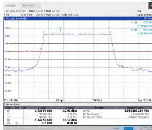
1-N66-PC3-15-10-M-2-DFT-PI2BPSK-Outer_Full- 50@0-Ant1-8.956-9.700-≤10-PASS
