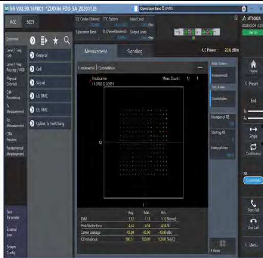
1-N2-PC3-15-20-M-5-DFT-256QAM-Outer_Full-100@0-Ant1-see graph-PASS
