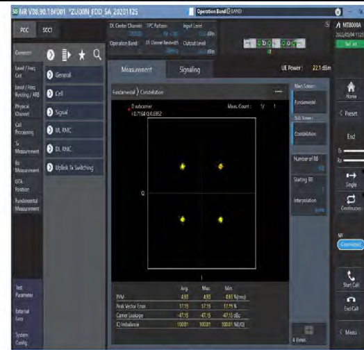
1-N2-PC3-15-20-M-6-CP-QPSK-Outer_Full-106@0-Ant1-see graph-PASS
