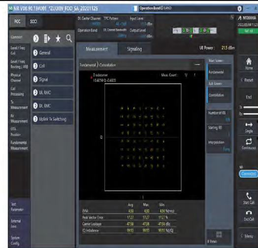
1-N2-PC3-15-20-M-8-CP-64QAM-Outer_Full-106@0-Ant1-see graph-PASS
