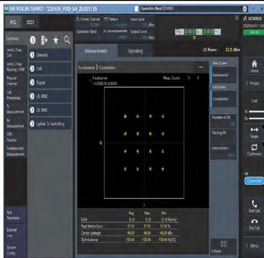
1-N2-PC3-15-20-M-7-CP-16QAM-Outer_Full-106@0-Ant1-see graph-PASS
