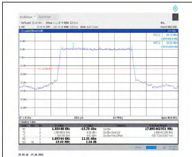
1-N2--15-20-H-2-DFT-PI2BPSK-Outer_Full-100@0- Ant1-17.895-19.080-≤20-PASS
