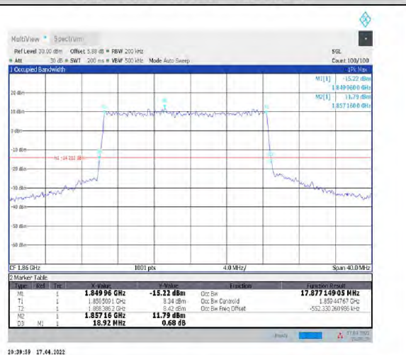
1-N2--15-20-L-3-DFT-16QAM-Outer_Full-100@0- Ant1-17.877-18.920-≤20-PASS
