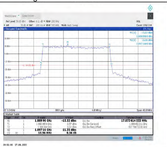
1-N2--15-20-H-3-DFT-16QAM-Outer_Full-100@0- Ant1-17.874-18.960-≤20-PASS
