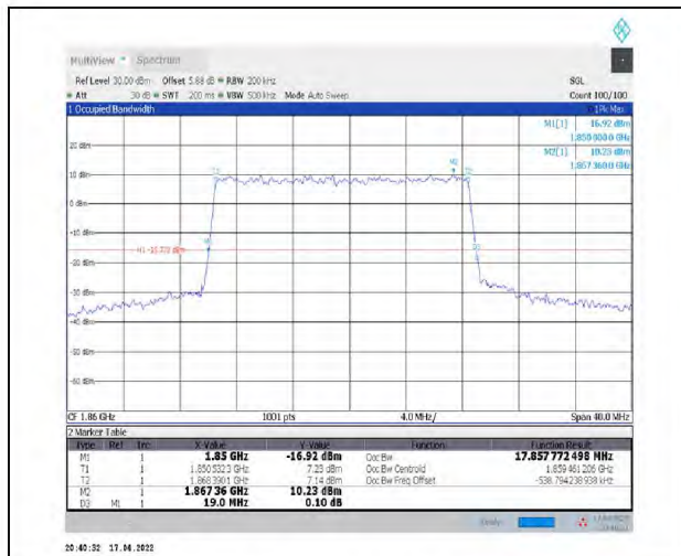
1-N2--15-20-L-4-DFT-64QAM-Outer_Full-100@0-Ant1-17.858-19.000-≤20-PASS
