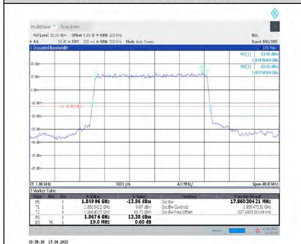
1-N2--15-20-L-2-DFT-PI2BPSK-Outer_Full-100@0- Ant1-17.86-19.000-≤20-PASS
