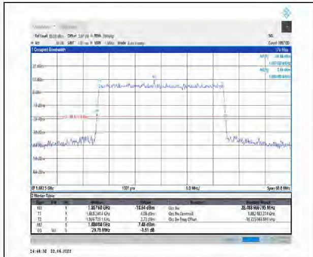
1-N25--15-30-M-9-CP-256QAM-Outer_Full-160@0- Ant1-28.484-29.760-≤30-PASS
