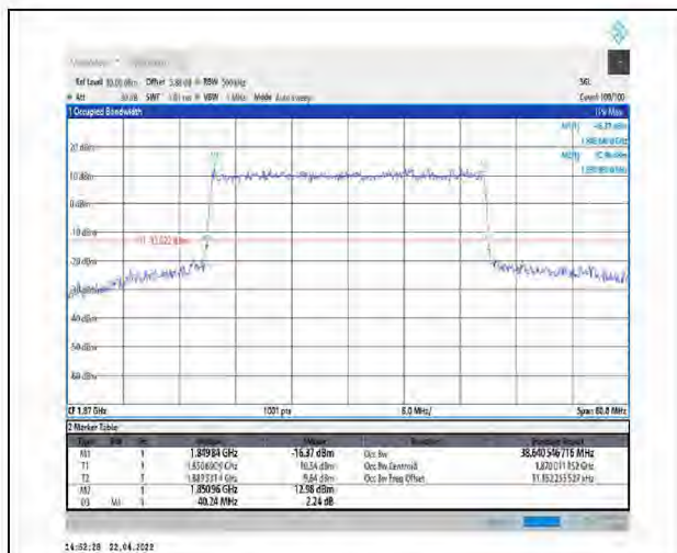
1-N25--15-40-L-3-DFT-16QAM-Outer_Full-216@0- Ant1-38.641-40.240-≤40-PASS
