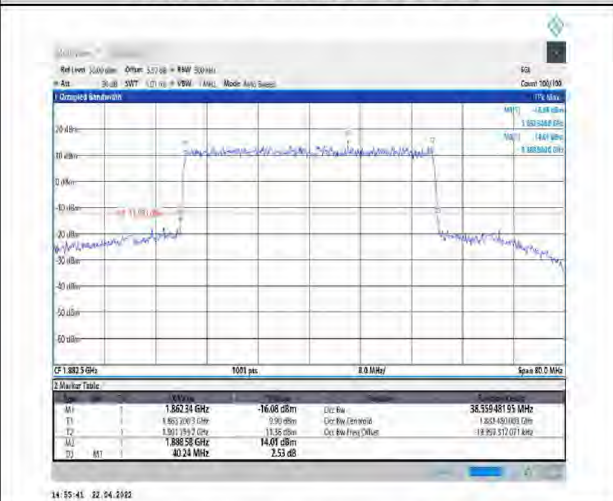
1-N25--15-40-M-1-DFT-QPSK-Outer_Full-216@0- Ant1-38.559-40.240-<40-PASS
