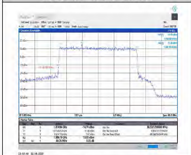
1-N25--15-40-H-3-DFT-16QAM-Outer_Full-216@0- Ant1-38.532-40.240-≤40-PASS
