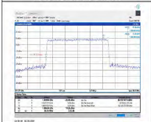
1-N25--15-40-L-5-DFT-256QAM-Outer_Full-216@0- Ant1-38.553-40.240-≤40-PASS
