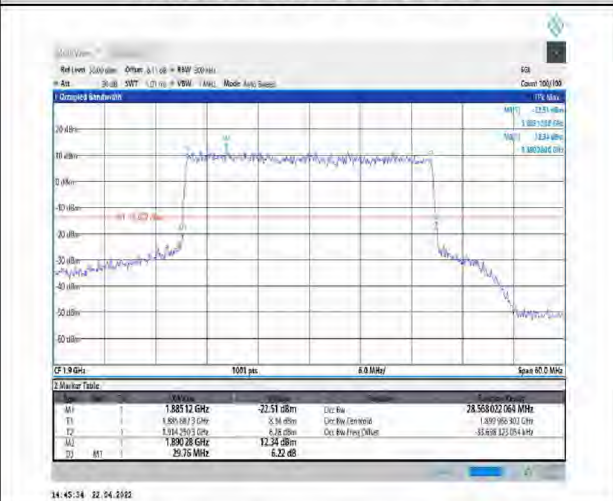
1-N25--15-30-H-3-DFT-16QAM-Outer_Full-160@0- Ant1-28.568-29.760-≤30-PASS
