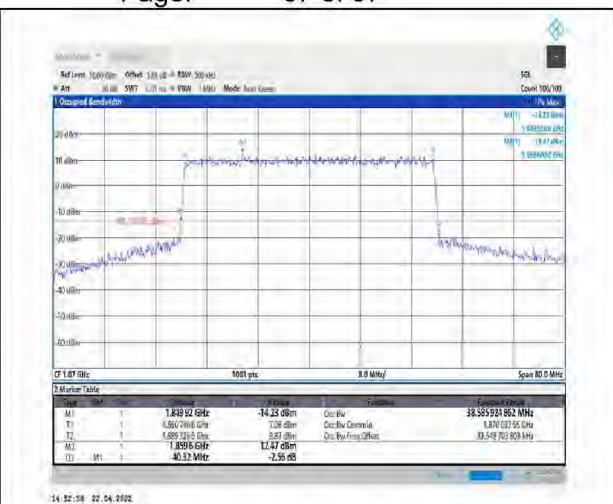
1-N25--15-40-L-4-DFT-64QAM-Outer_Full-216@0- Ant1-38.586-40.320-≤40-PASS
