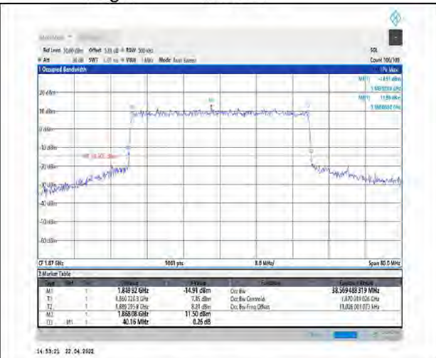
1-N25--15-40-L-8-CP-64QAM-Outer_Full-216@0- Ant1-38.569-40.160-<40-PASS
