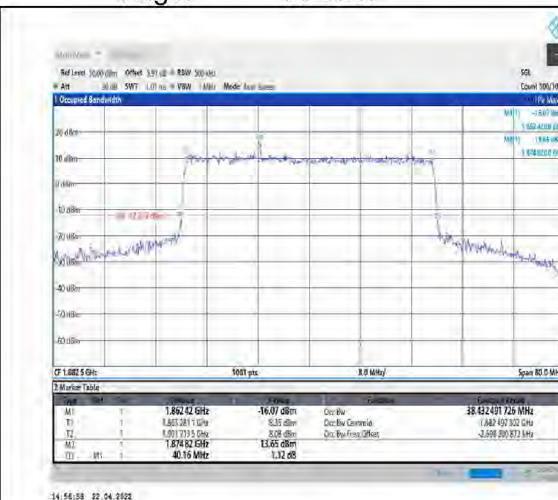
1-N25--15-40-M-7-CP-16QAM-Outer_Full-216@0- Ant1-38.432-40.160-≤40-PASS
