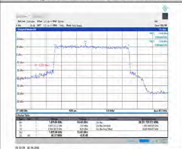
1-N25--15-40-H-4-DFT-64QAM-Outer_Full-216@0- Ant1-38.552-40.320-≤40-PASS
