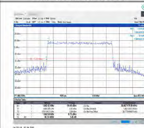
1-N25--15-40-M-9-CP-256QAM-Outer_Full-216@0- Ant1-38.607-40.160-≤40-PASS
