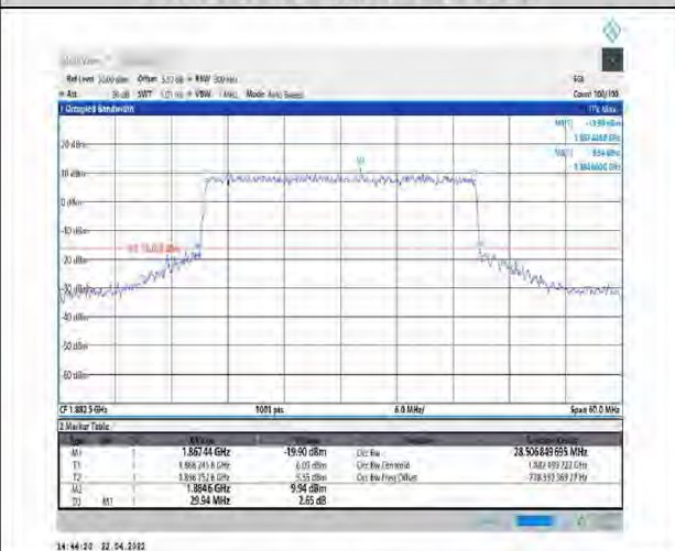
1-N25--15-30-M-8-CP-64QAM-Outer_Full-160@0-Ant1-28.507-29.940-≤30-PASS
