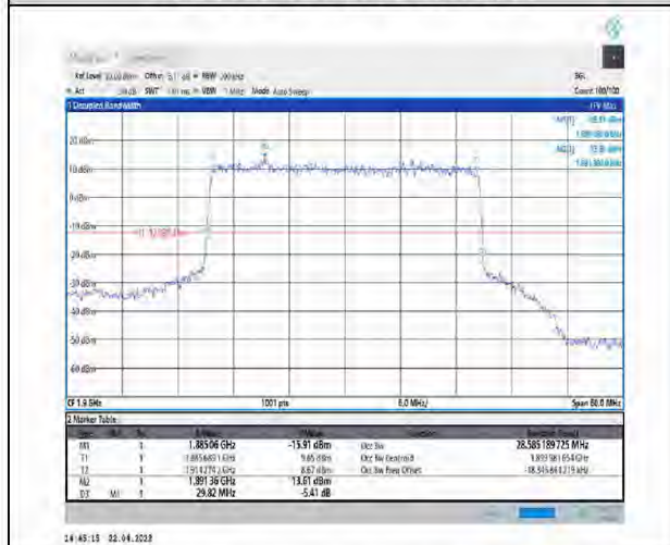
1-N25--15-30-H-2-DFT-PI2BPSK-Outer_Full- 160@0-Ant1-28.585-29.820-≤30-PASS
