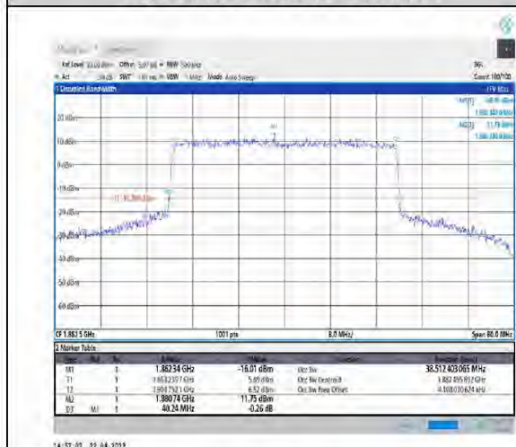
1-N25--15-40-M-8-CP-64QAM-Outer_Full-216@0- Ant1-38.512-40.240-≤40-PASS
