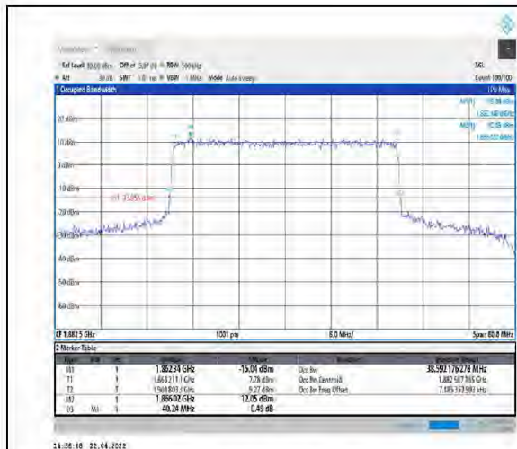
1-N25--15-40-M-6-CP-QPSK-Outer_Full-216@0- Ant1-38.592-40.240-≤40-PASS
