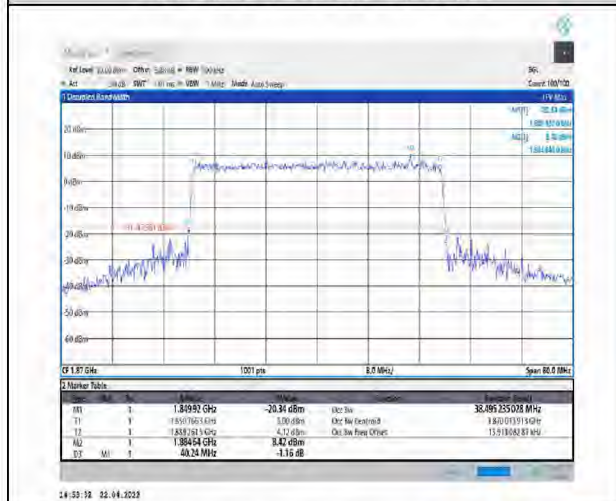
1-N25--15-40-L-9-CP-256QAM-Outer_Full-216@0- Ant1-38.495-40.240-<40-PASS
