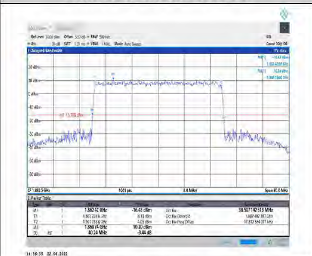
1-N25--15-40-M-5-DFT-256QAM-Outer_Full-216@0- Ant1-38.507-40.240-≤40-PASS
