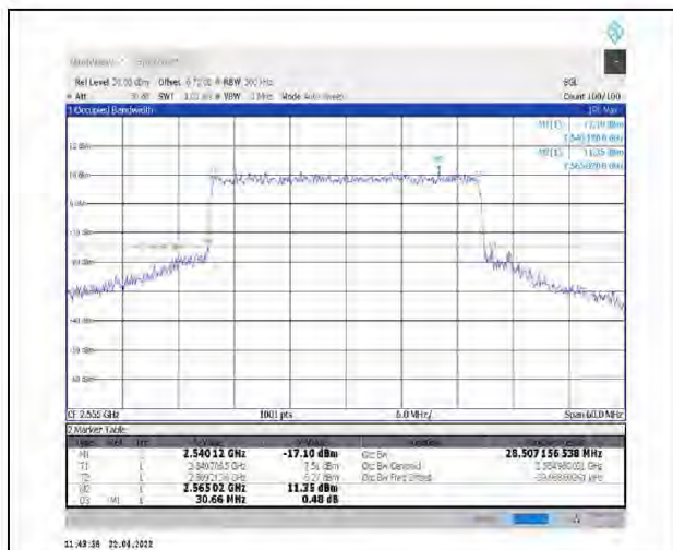
1-N7--15-30-H-8-CP-64QAM-Outer_Full-160@0- Ant1-28.509-30.660-≤30-PASS
