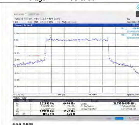
1-N7--15-40-H-6-CP-QPSK-Outet_Full-216@0-Ant1- 38.55-40.160-≤40-PASS
