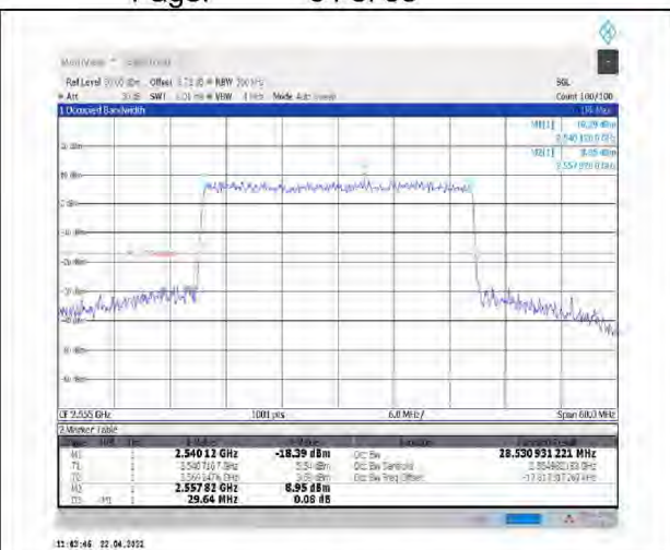
1-N7--15-30-H-9-CP-256QAM-Outer_Full-160@0- Ant1-28.533-29.640-≤30-PASS
