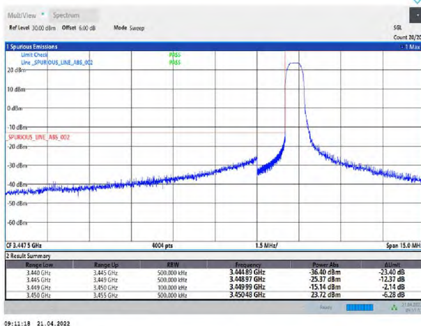
Band42-5MHz-QPSK-42115-25RB#0
