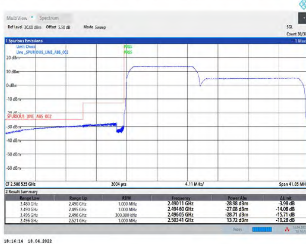
41-41-10MHz-15MHz-QPSK-QPSK-39703-39823-50RB#0-75RB#0
