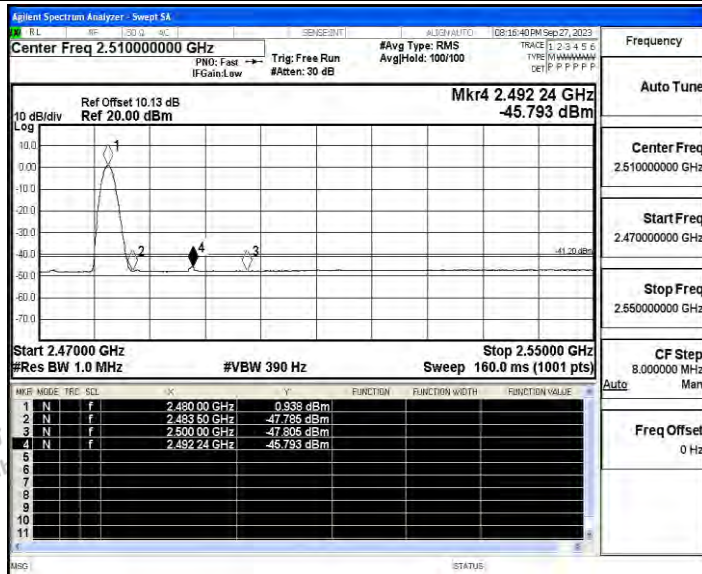
DH5_Ant_High_2480_Peak
