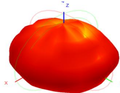
2500.0MHz H+V, Eff. 46.66%
