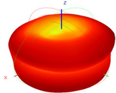
2450.0MHz H+V, Eff. 50.41%
