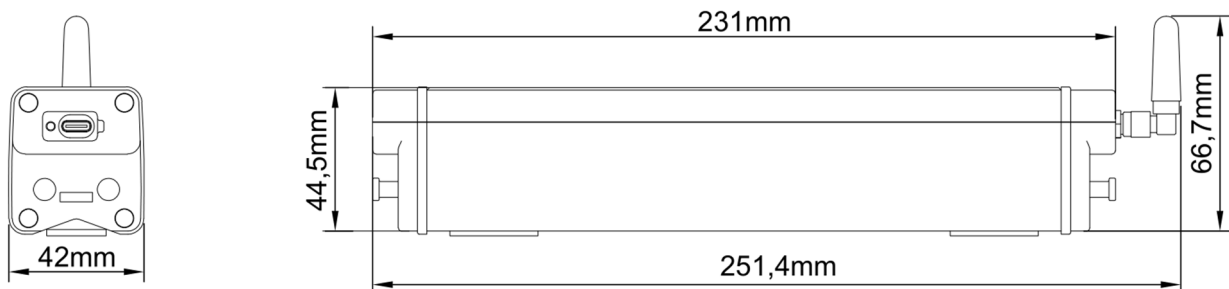
Dimension Diagram
