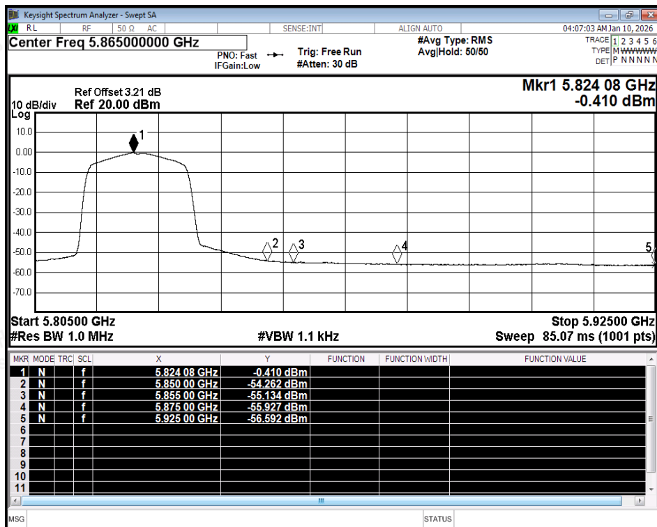
Restrict Band NVNT ax20 5825MHz Ant1 Average
