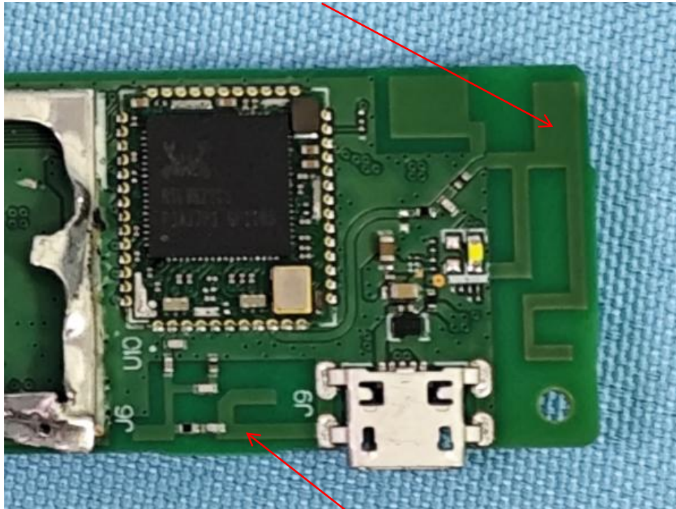
Module2(TV Stick)-BT&WiFi ANT1
