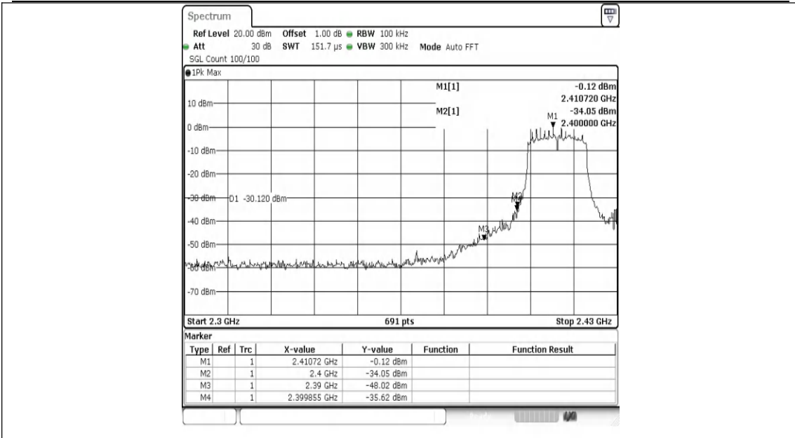
11N20MIMO-Ant0-2412-PASS
