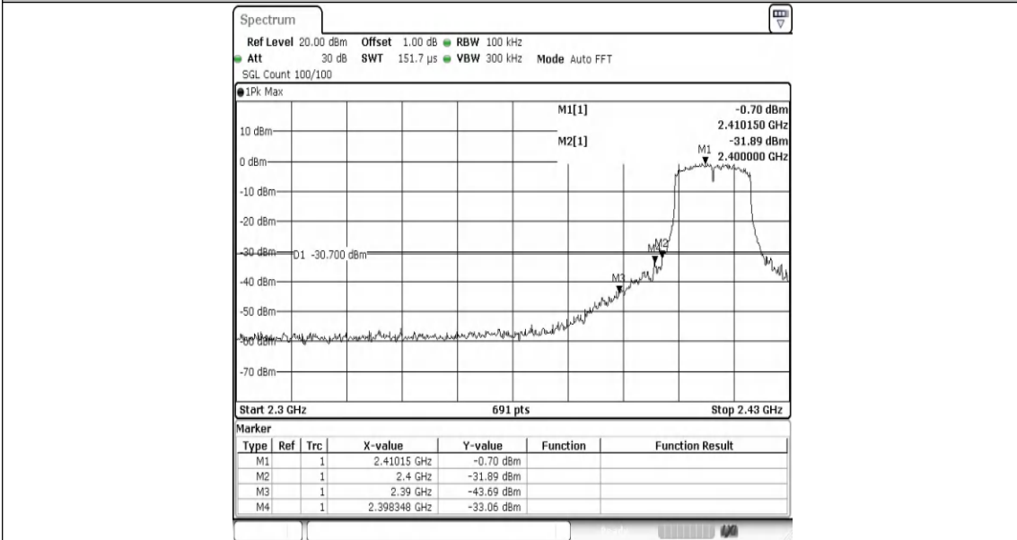
11N20MIMO-Ant1-2412-PASS
