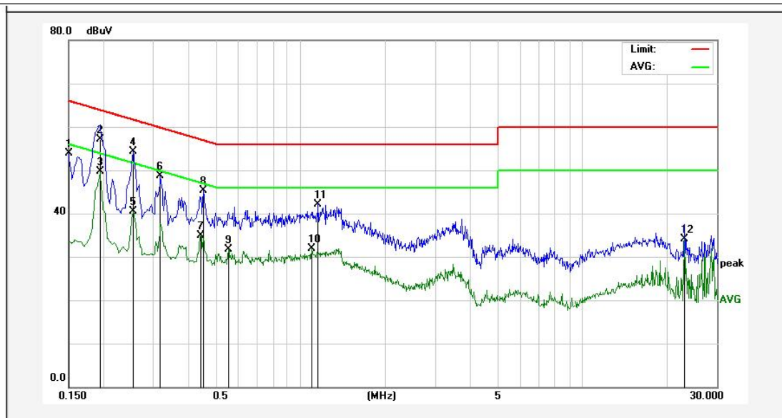
TM1 / Line: Neutral / Band: 2400-2483.5 MHz / BW: 1 / CH: M
