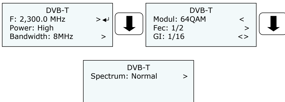
Figure 4.35: DVB-T Menu
