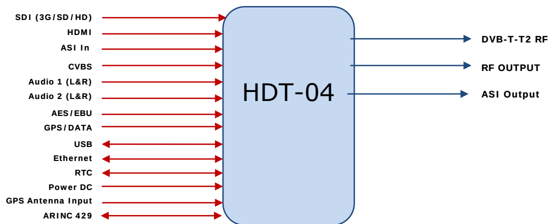
Figure 9.1: HDT-04 Connections
