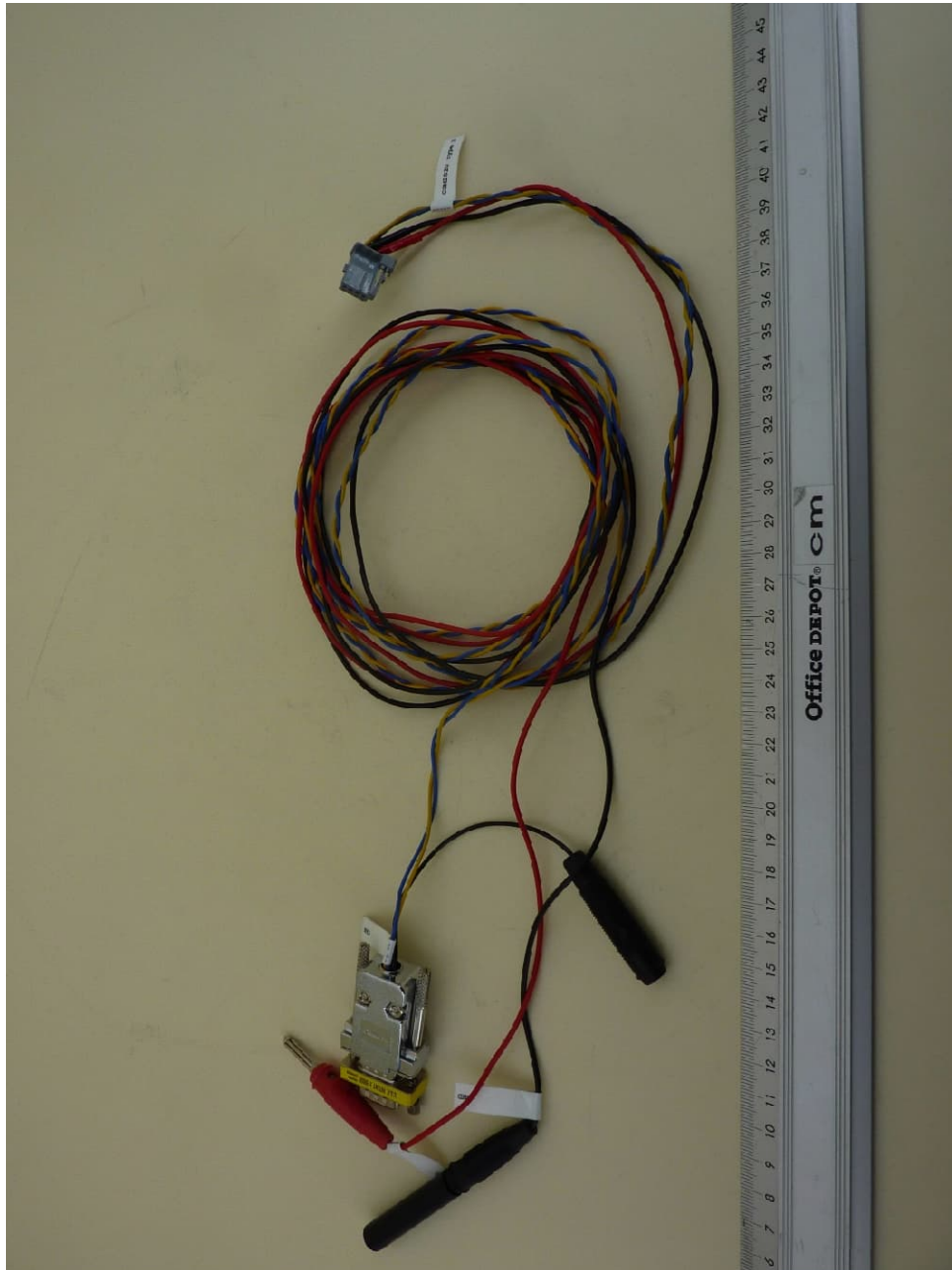
Wire harness
