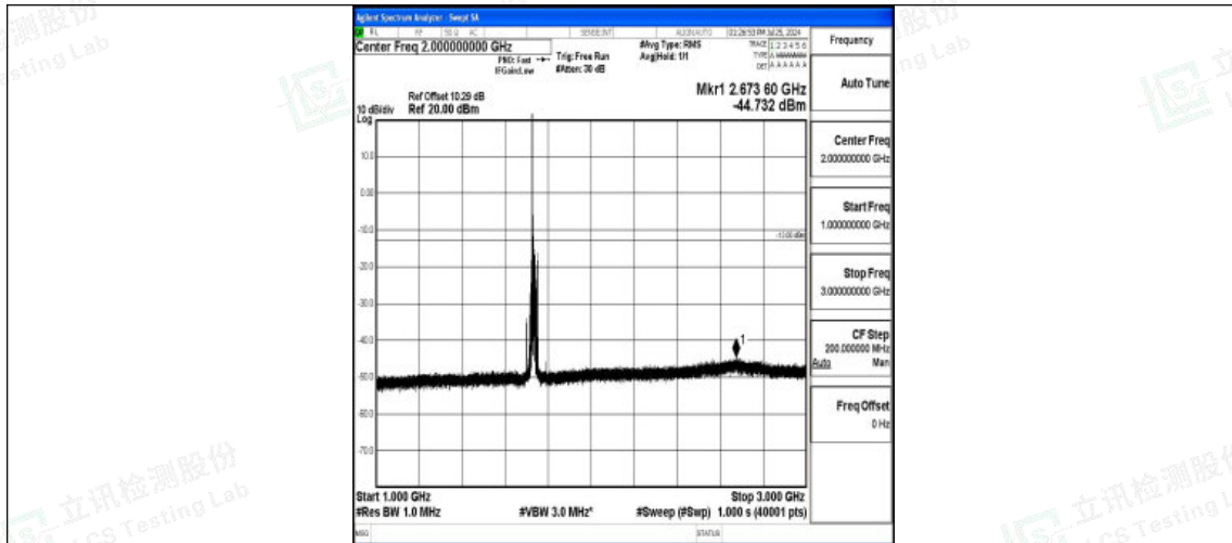
Band4-15MHz-16QAM-20175-1RB#0-1000~3000-PASS
