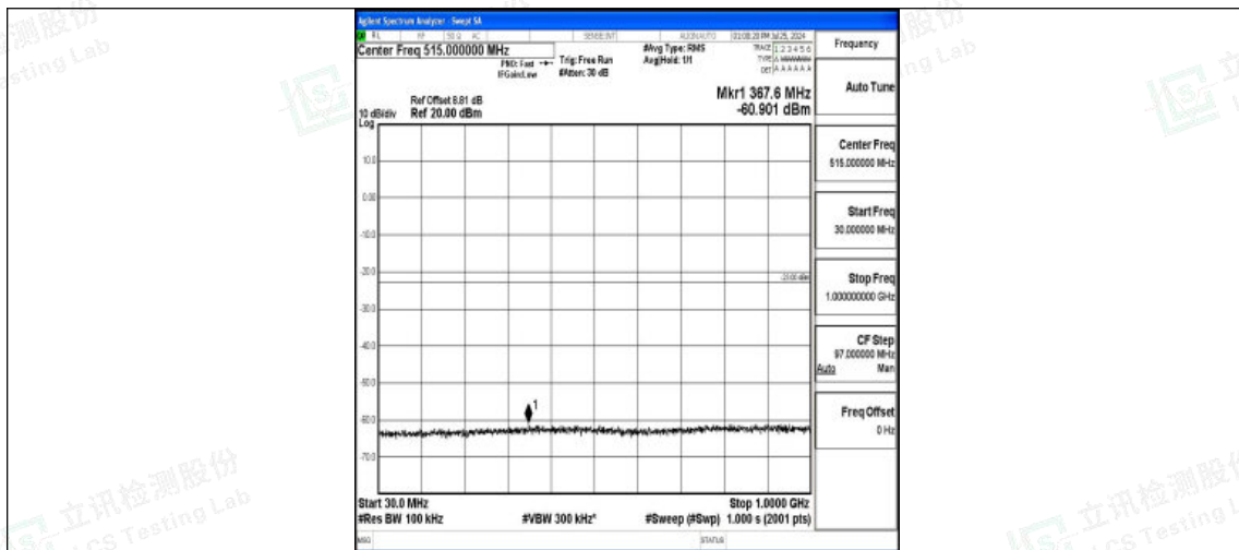
Band4-10MHz-QPSK-20175-1RB#0-30~1000-PASS
