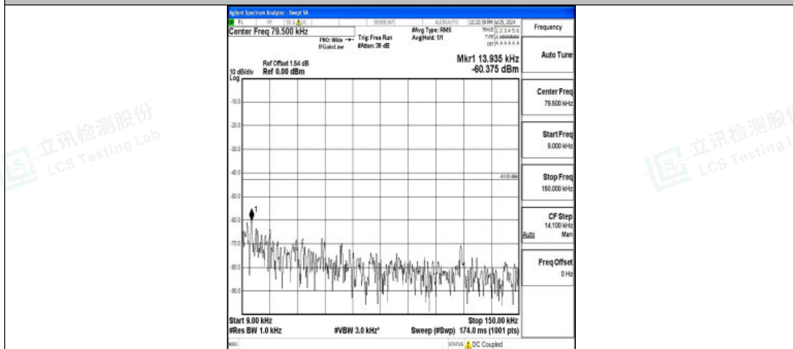
Band4-3MHz-QPSK-20385-1RB#0-0.009~0.15-PASS
