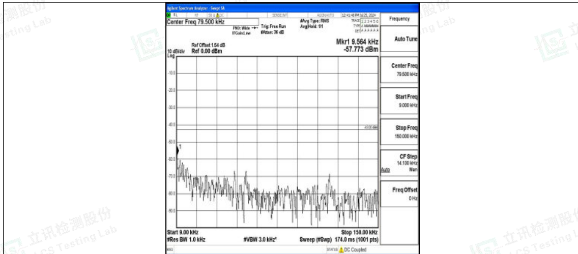
Band4-5MHz-16QAM-20175-1RB#0-0.009~0.15-PASS
