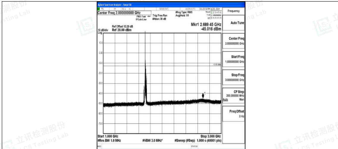
Band4-15MHz-QPSK-20025-1RB#0-1000~3000-PASS
