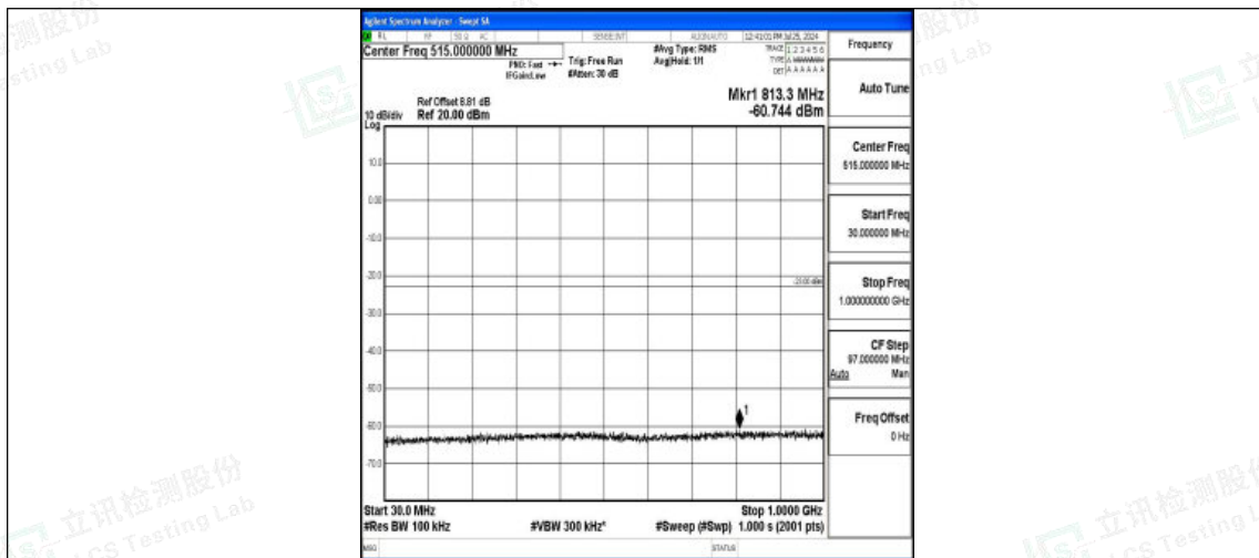
Band4-5MHz-QPSK-20175-1RB#0-30~1000-PASS
