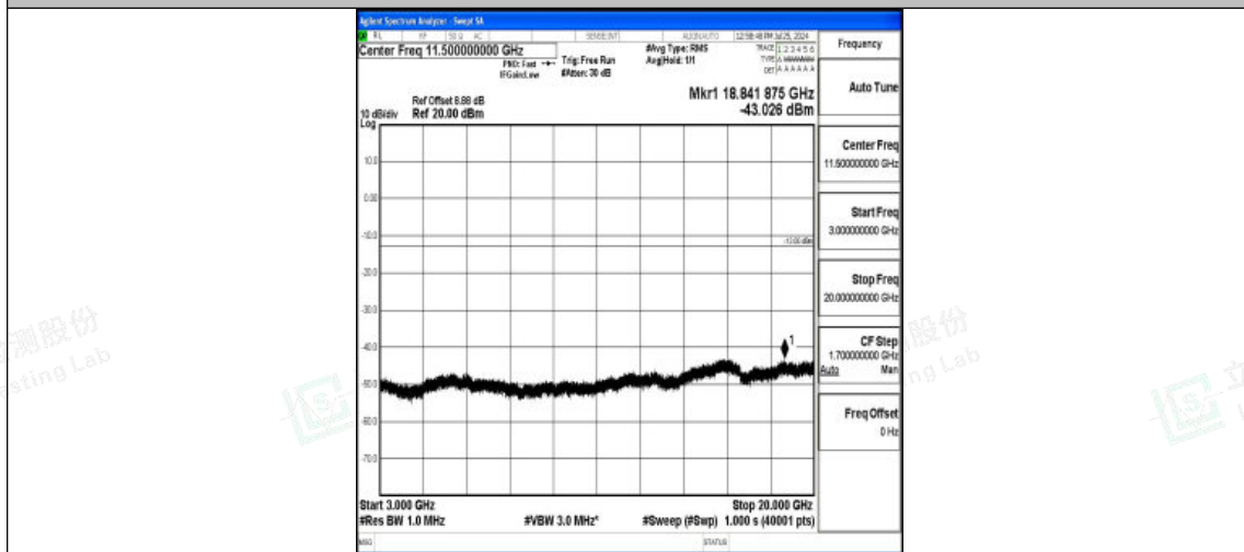
Band4-10MHz-QPSK-20000-1RB#0-3000~20000-PASS
