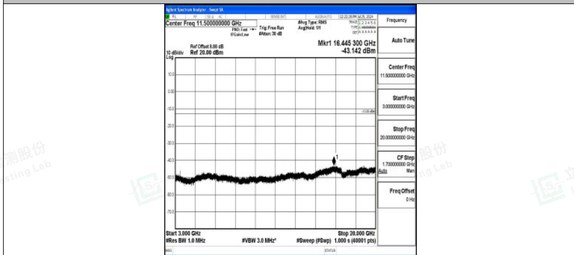
Band4-3MHz-16QAM-20175-1RB#0-3000~20000-PASS
