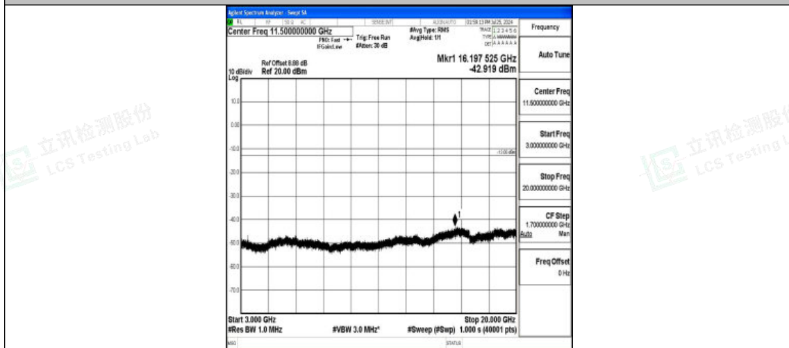
Band4-20MHz-QPSK-20175-1RB#0-3000~20000-PASS
