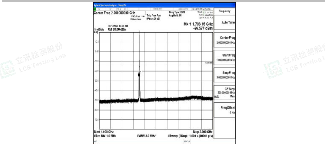
Band4-3MHz-16QAM-19965-1RB#0-1000~3000-PASS
