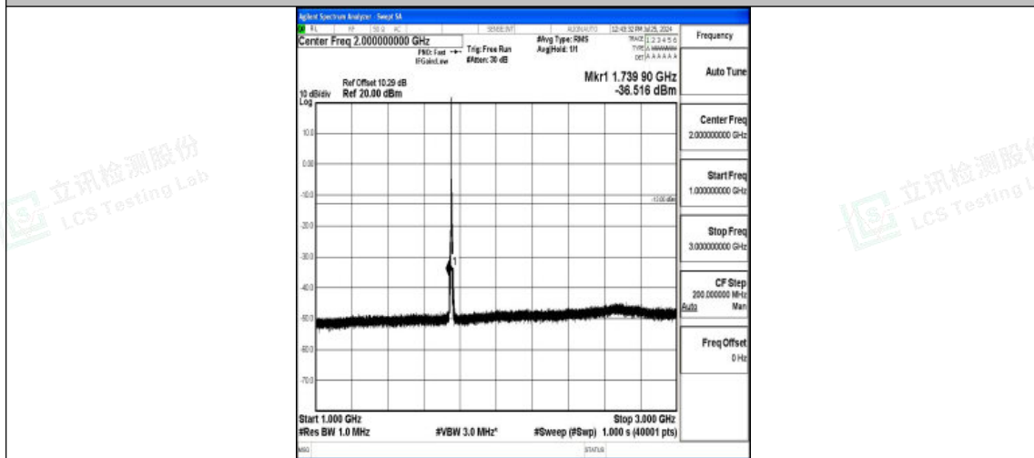
Band4-5MHz-QPSK-20375-1RB#0-1000~3000-PASS
