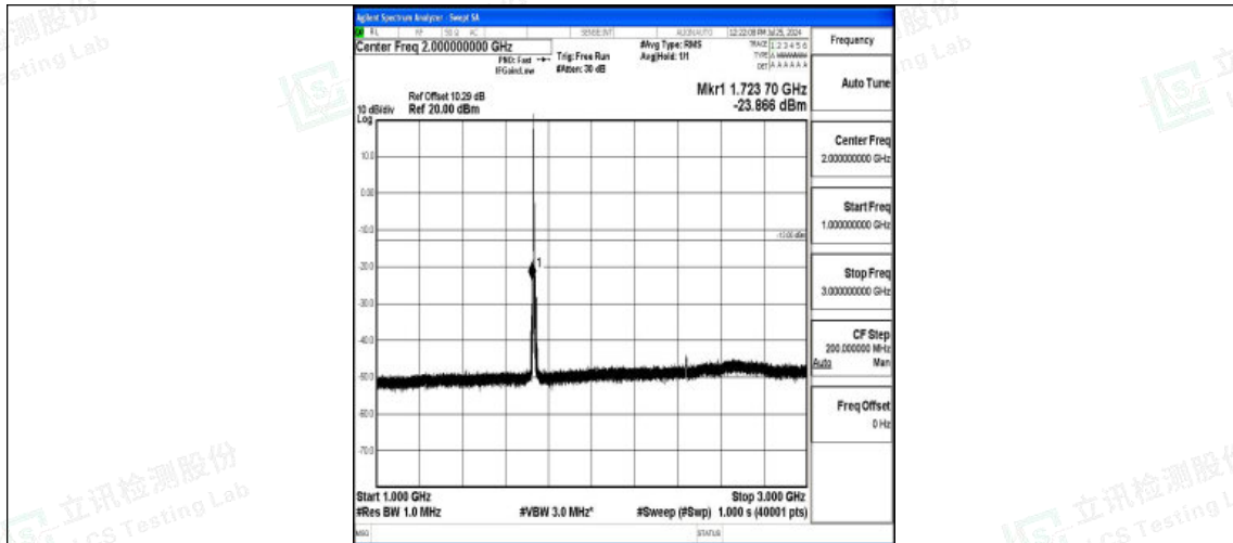
Band4-3MHz-16QAM-20175-1RB#0-1000~3000-PASS
