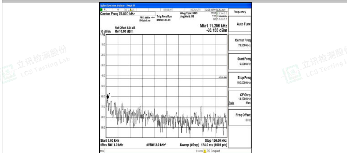
Band4-20MHz-QPSK-20300-1RB#0-0.009~0.15-PASS
