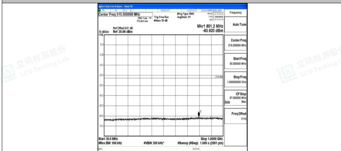
Band4-3MHz-16QAM-20175-1RB#0-30~1000-PASS
