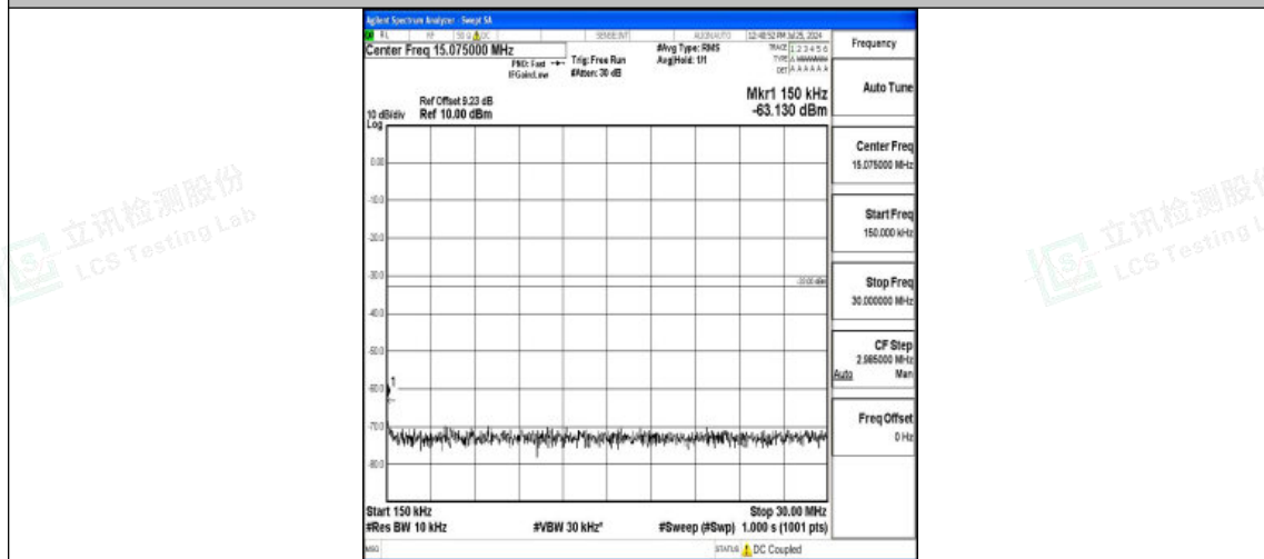
Band4-5MHz-QPSK-20175-1RB#0-0.15~30-PASS
