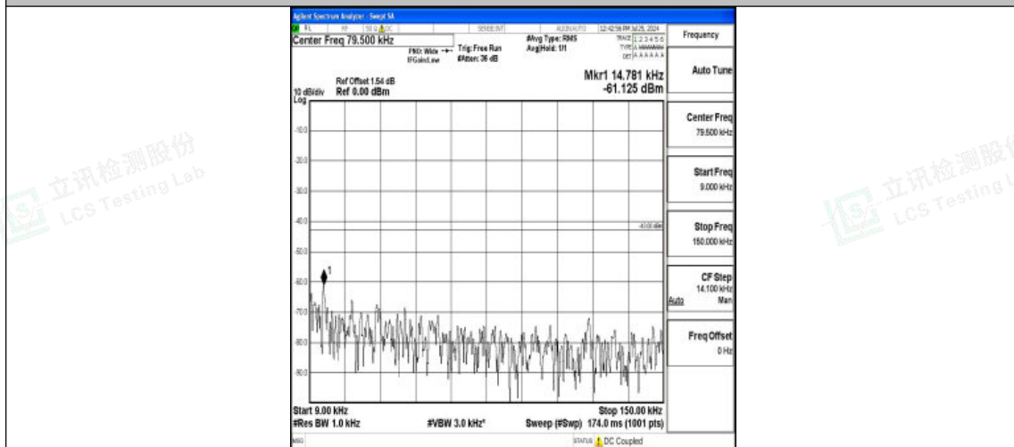
Band4-5MHz-QPSK-20375-1RB#0-0.009~0.15-PASS
