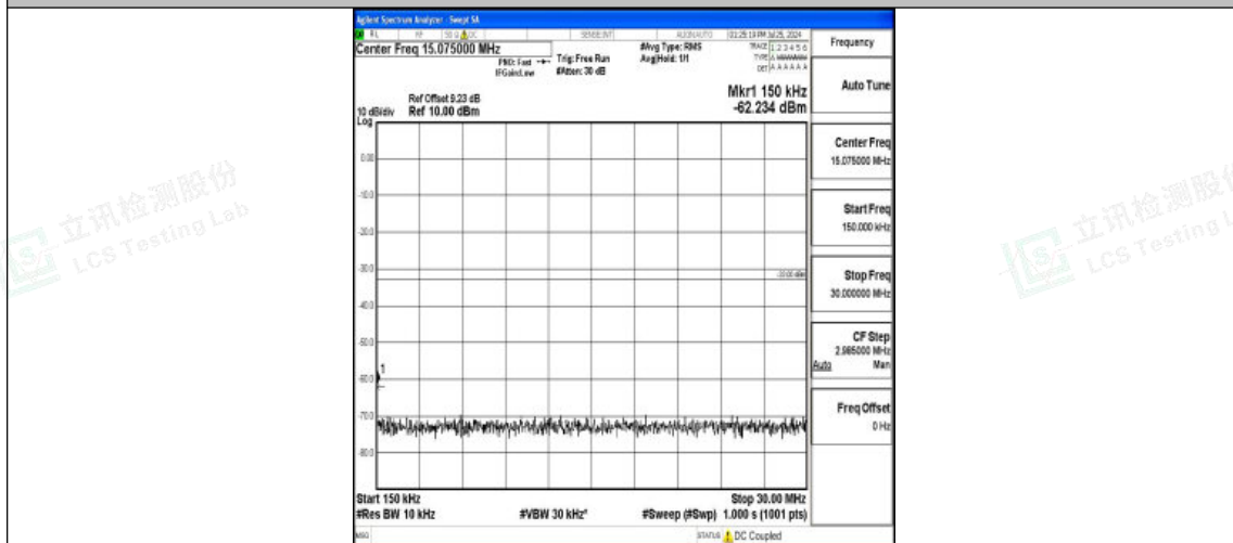
Band4-15MHz-QPSK-20175-1RB#0-0.15~30-PASS
