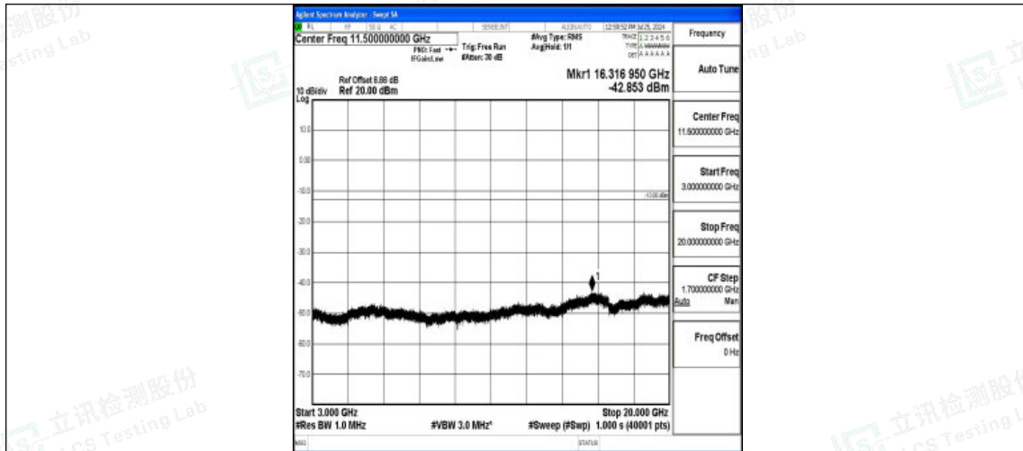
Band4-10MHz-16QAM-20000-1RB#0-3000~20000-PASS
