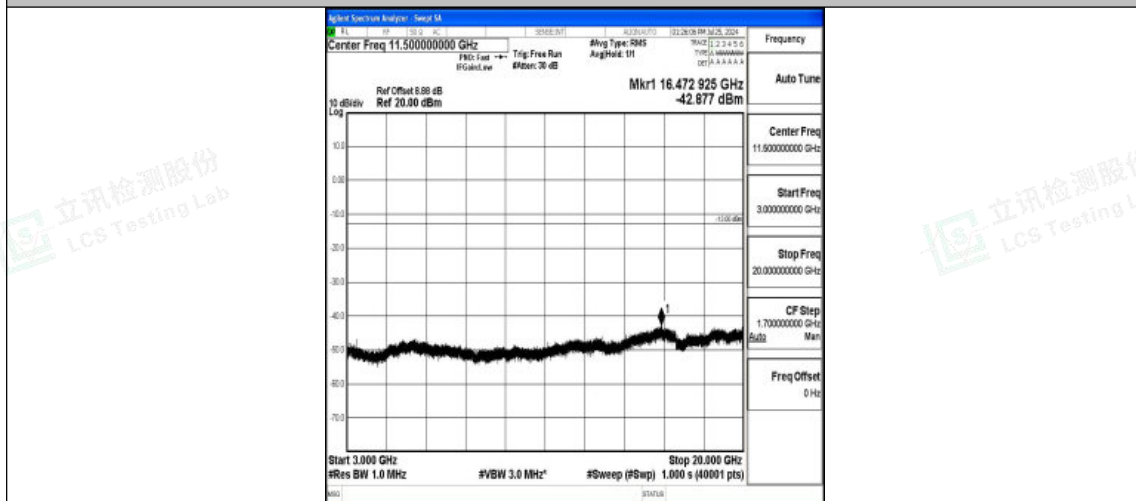
Band4-15MHz-QPSK-20175-1RB#0-3000~20000-PASS
