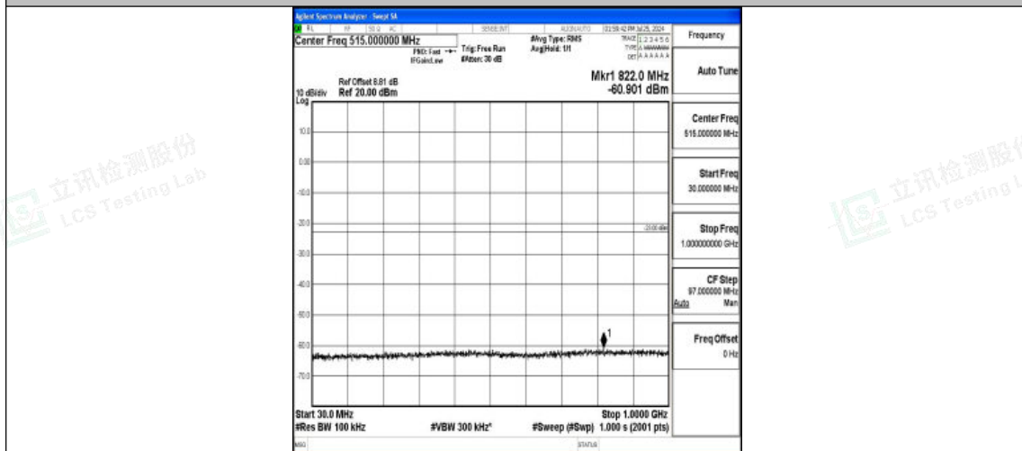
Band4-20MHz-16QAM-20175-1RB#0-30~1000-PASS
