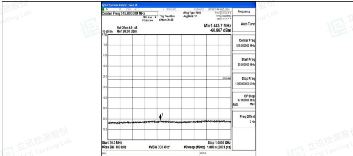
Band4-20MHz-QPSK-20175-1RB#0-30~1000-PASS
