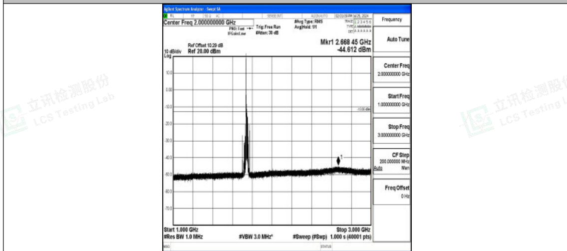
Band4-20MHz-QPSK-20300-1RB#0-1000~3000-PASS
