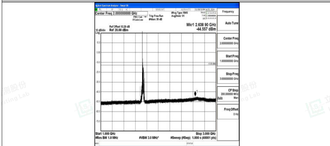
Band4-20MHz-QPSK-20175-1RB#0-1000~3000-PASS
