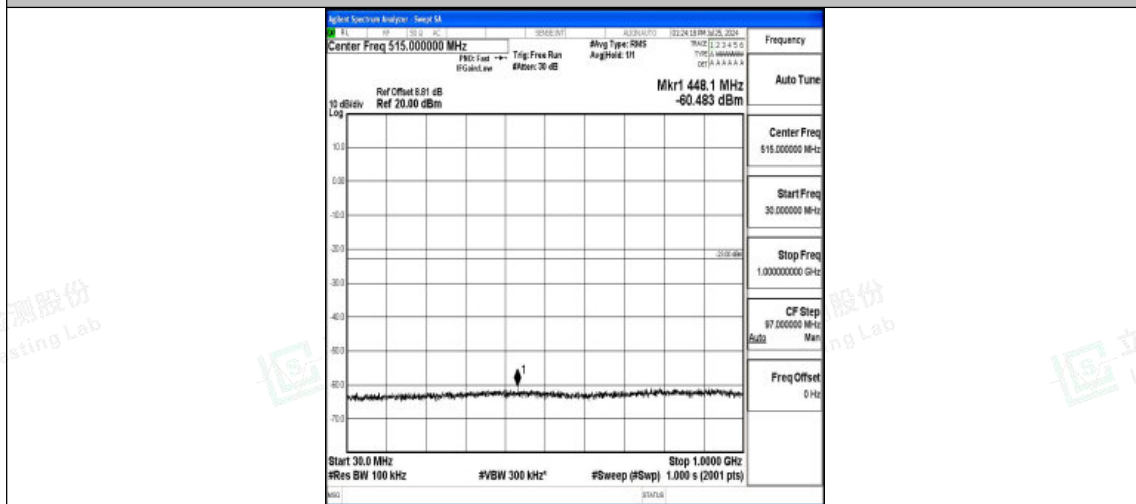
Band4-15MHz-16QAM-20025-1RB#0-30~1000-PASS
