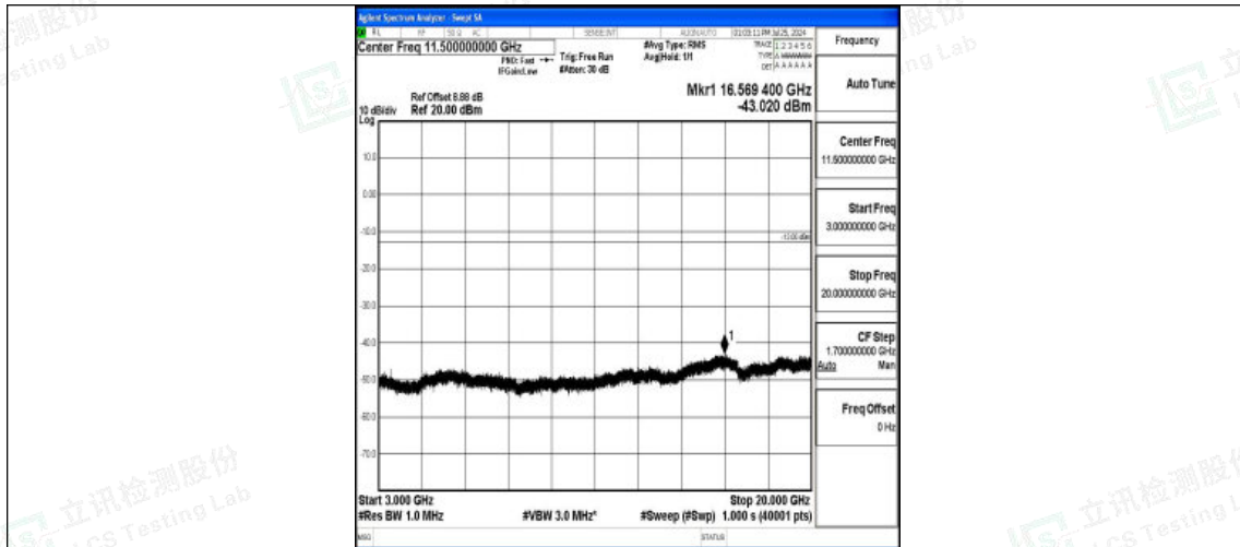
Band4-10MHz-QPSK-20350-1RB#0-3000~20000-PASS
