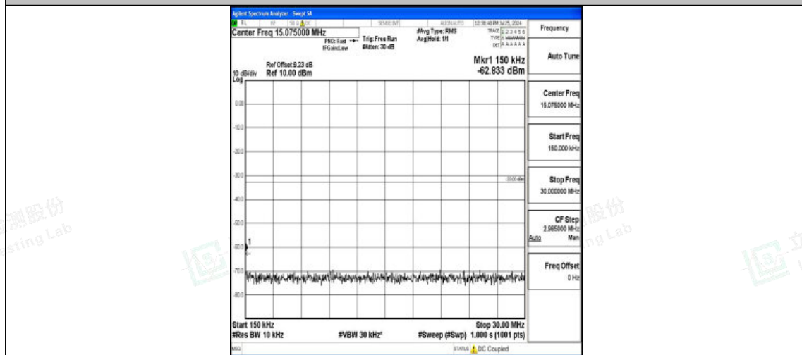
Band4-5MHz-QPSK-19975-1RB#0-0.15~30-PASS
