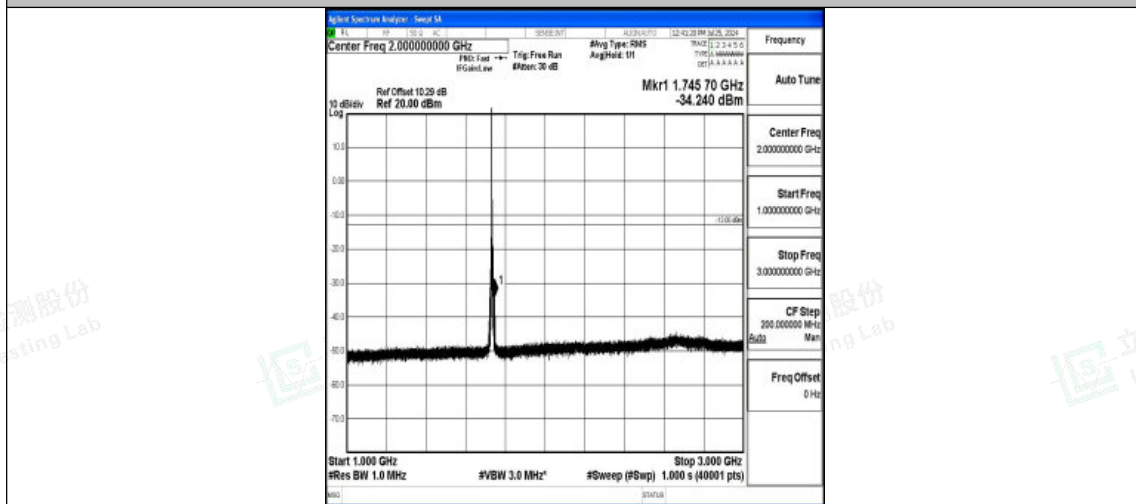
Band4-5MHz-QPSK-20175-1RB#0-1000~3000-PASS
