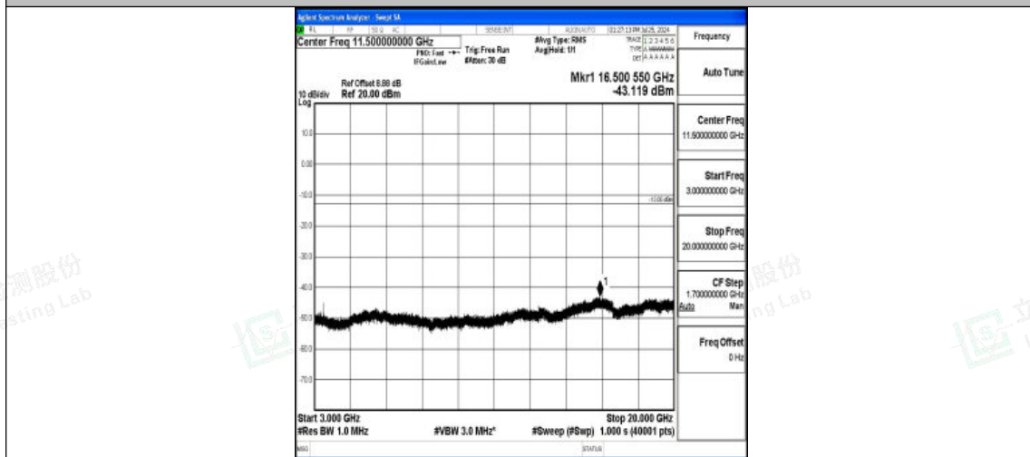
Band4-15MHz-16QAM-20175-1RB#0-3000~20000-PASS
