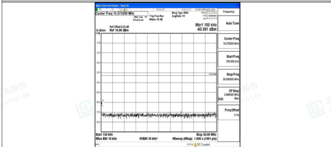
Band4-20MHz-16QAM-20175-1RB#0-0.15~30-PASS
