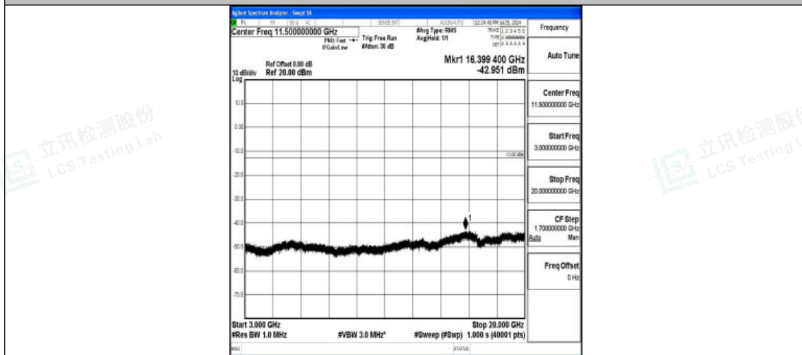
Band4-3MHz-16QAM-20385-1RB#0-3000~20000-PASS
