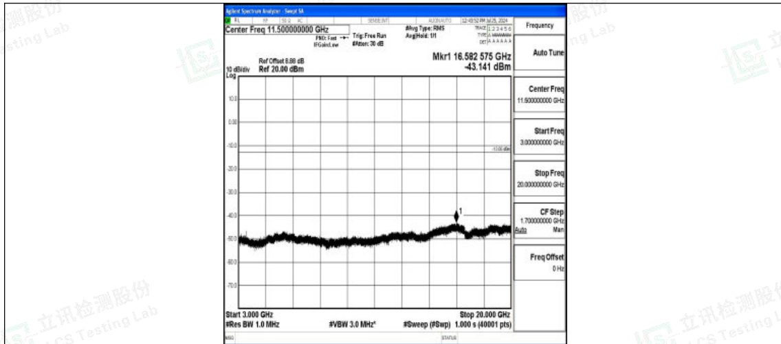
Band4-5MHz-QPSK-20375-1RB#0-3000~20000-PASS
