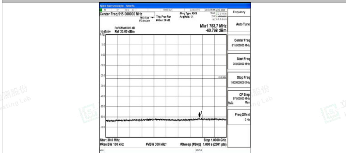
Band4-3MHz-16QAM-19965-1RB#0-30~1000-PASS
