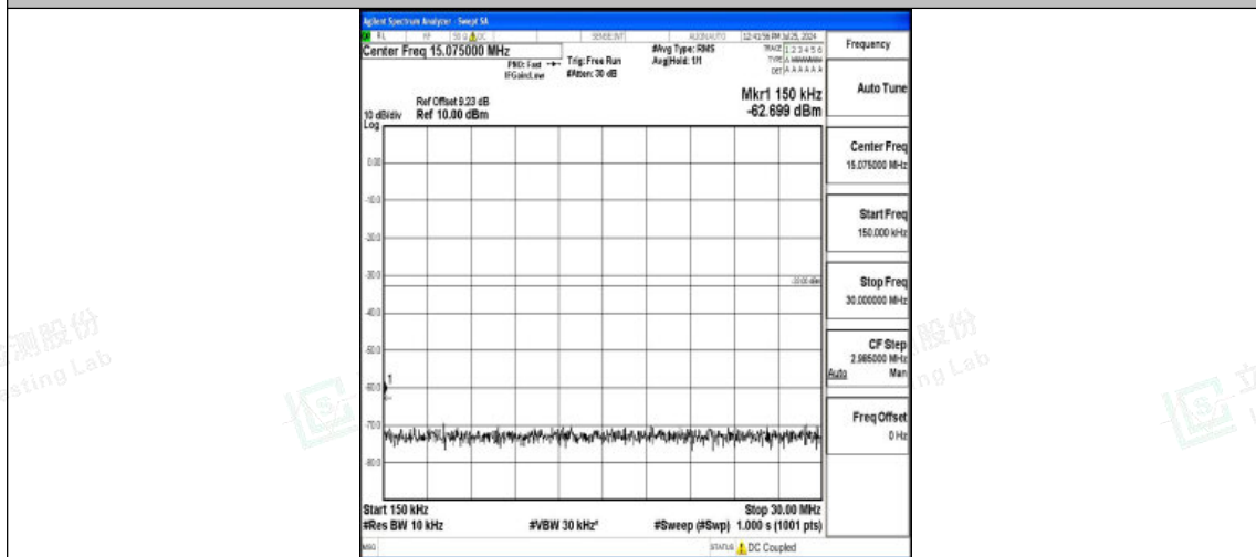
Band4-5MHz-16QAM-20175-1RB#0-0.15~30-PASS
