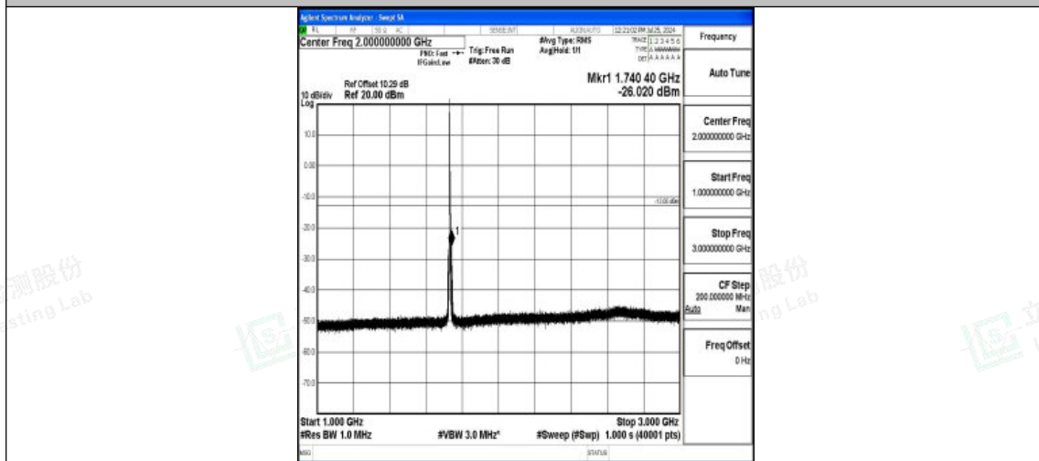
Band4-3MHz-QPSK-20175-1RB#0-1000~3000-PASS
