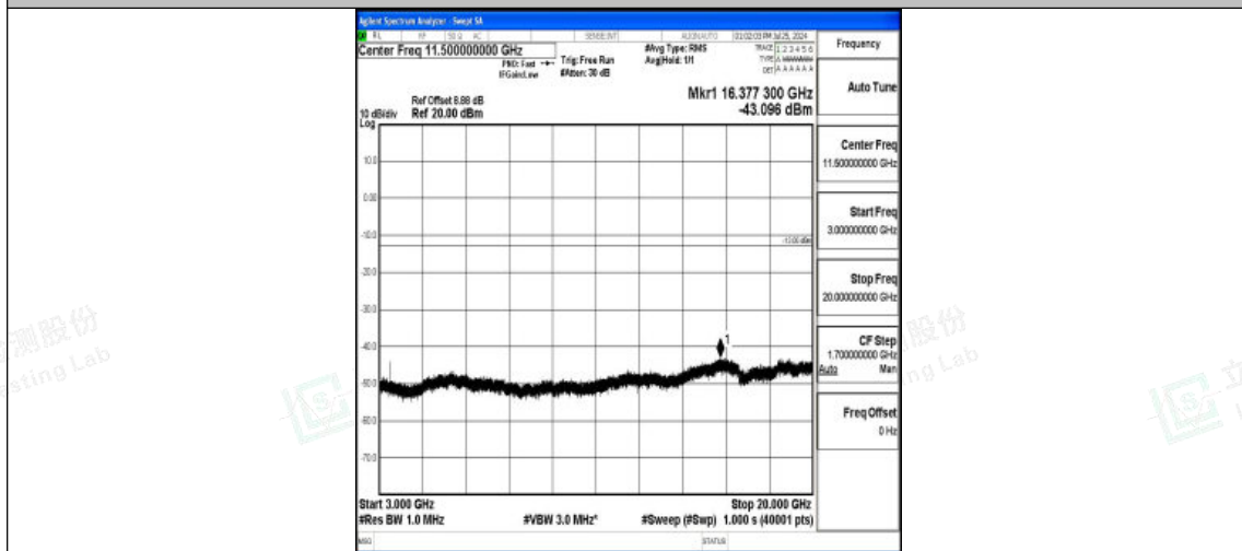
Band4-10MHz-16QAM-20175-1RB#0-3000~20000-PASS
