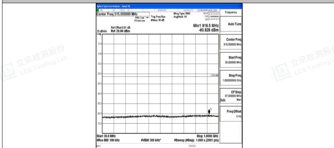
Band4-10MHz-QPSK-20000-1RB#0-30~1000-PASS
