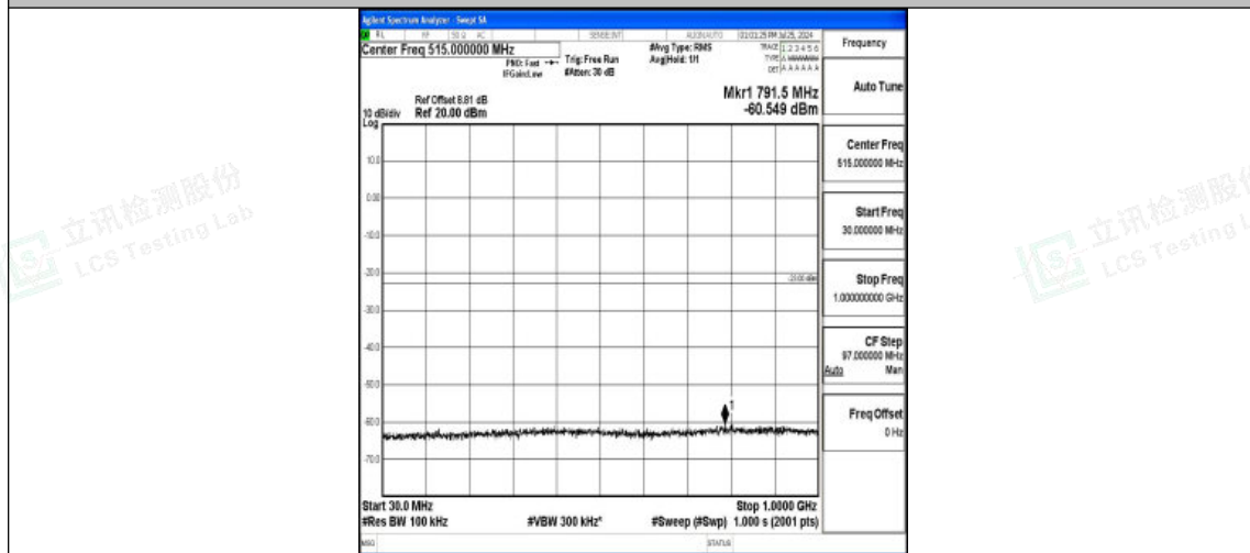
Band4-10MHz-16QAM-20175-1RB#0-30~1000-PASS
