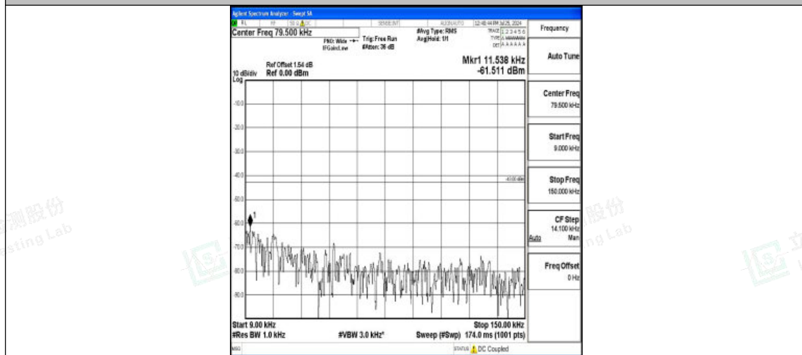
Band4-5MHz-QPSK-20175-1RB#0-0.009~0.15-PASS
