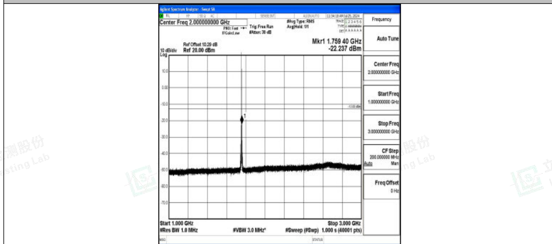
Band4-1.4MHz-16QAM-20393-1RB#0-1000~3000-PASS
