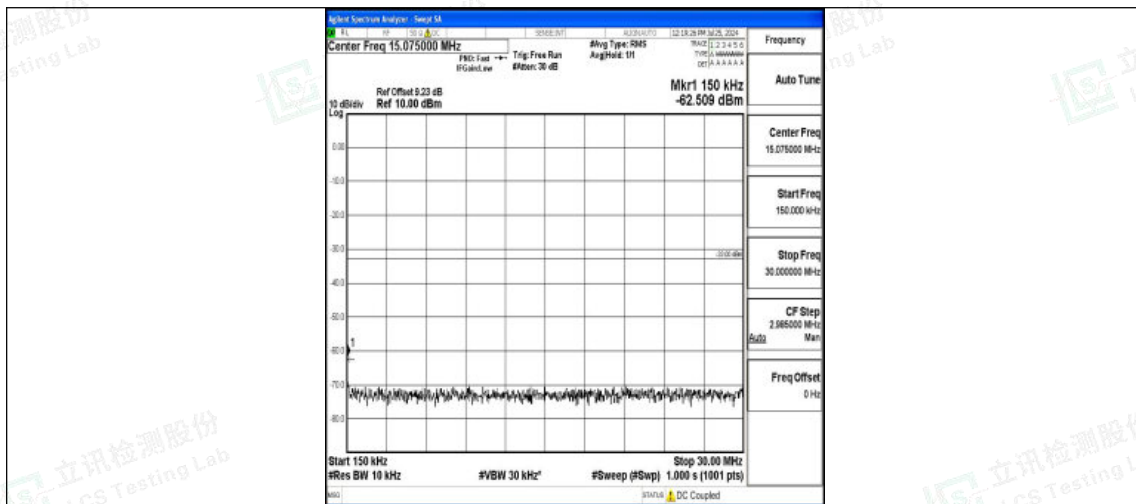
Band4-3MHz-16QAM-19965-1RB#0-0.15~30-PASS
