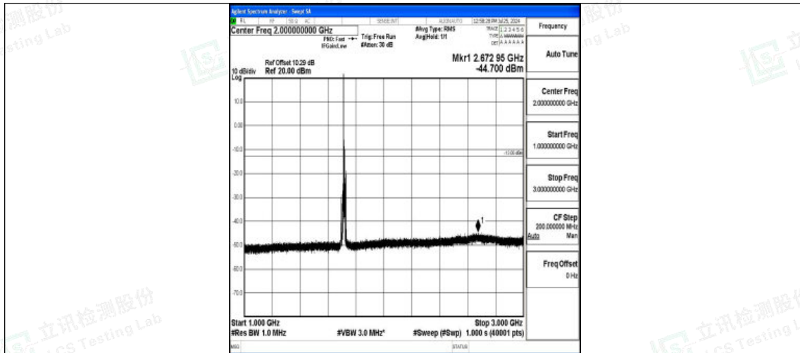
Band4-10MHz-QPSK-20000-1RB#0-1000~3000-PASS
