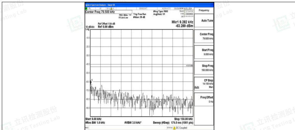
Band4-10MHz-16QAM-20175-1RB#0-0.009~0.15-PASS
