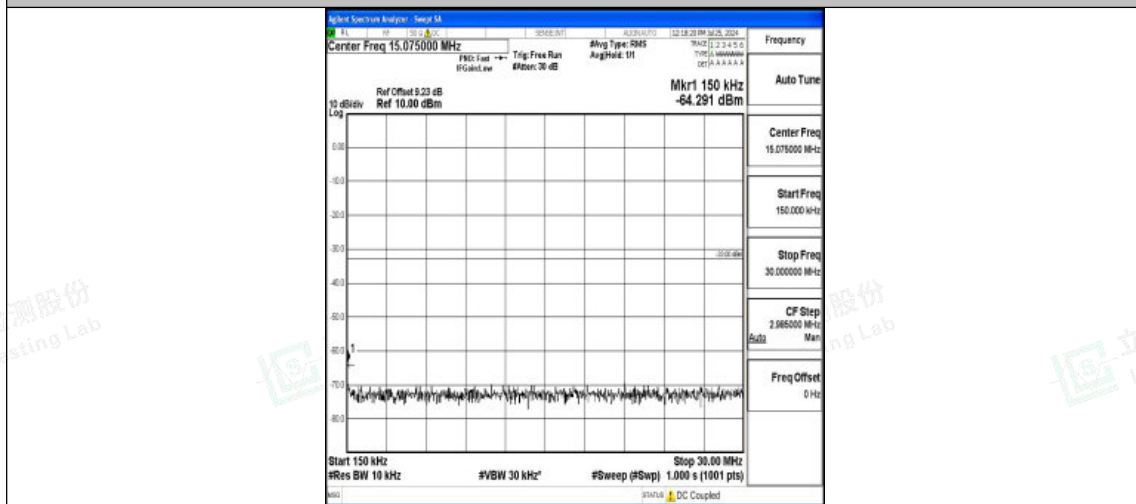
Band4-3MHz-QPSK-19965-1RB#0-0.15~30-PASS
