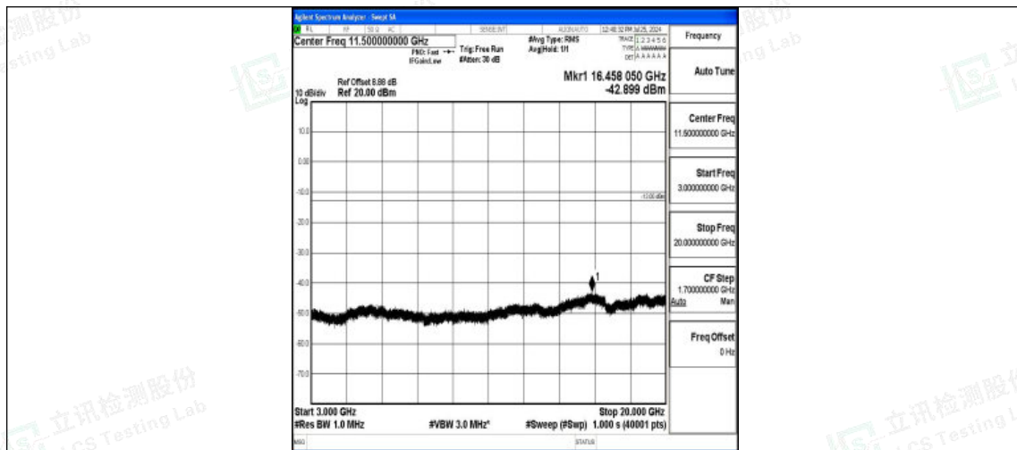
Band4-5MHz-16QAM-19975-1RB#0-3000~20000-PASS
