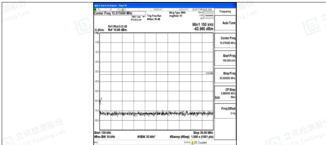
Band4-20MHz-16QAM-20050-1RB#0-0.15~30-PASS
