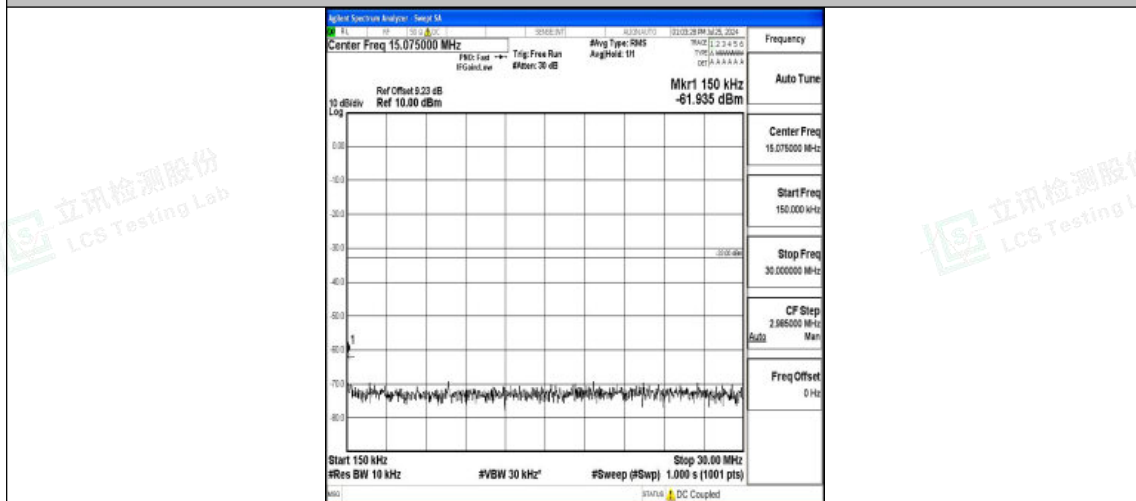
Band4-10MHz-16QAM-20350-1RB#0-0.15~30-PASS
