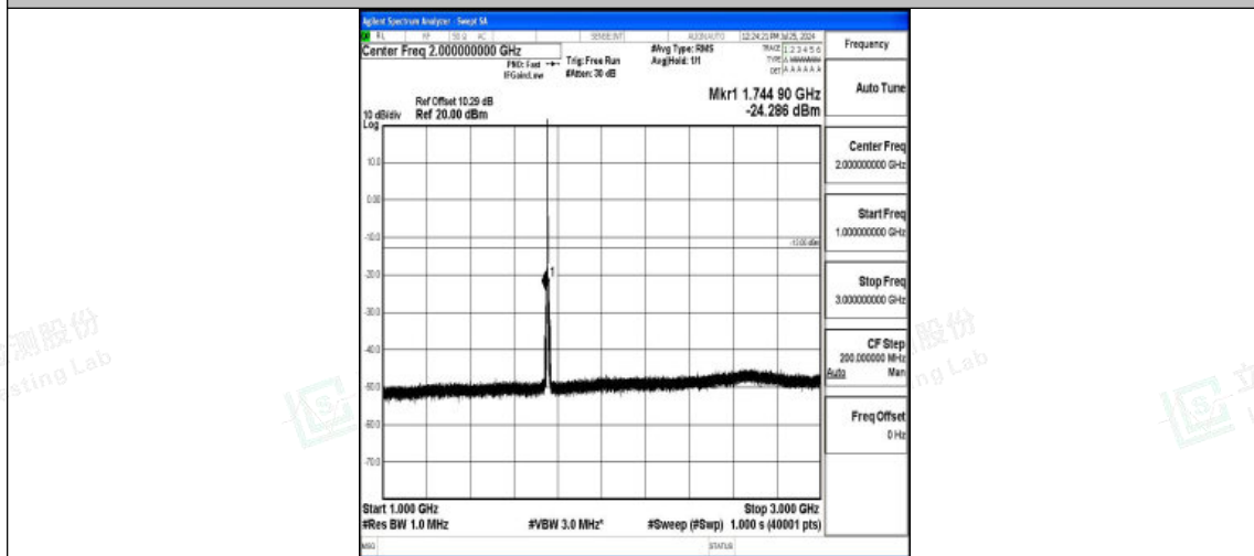
Band4-3MHz-16QAM-20385-1RB#0-1000~3000-PASS
