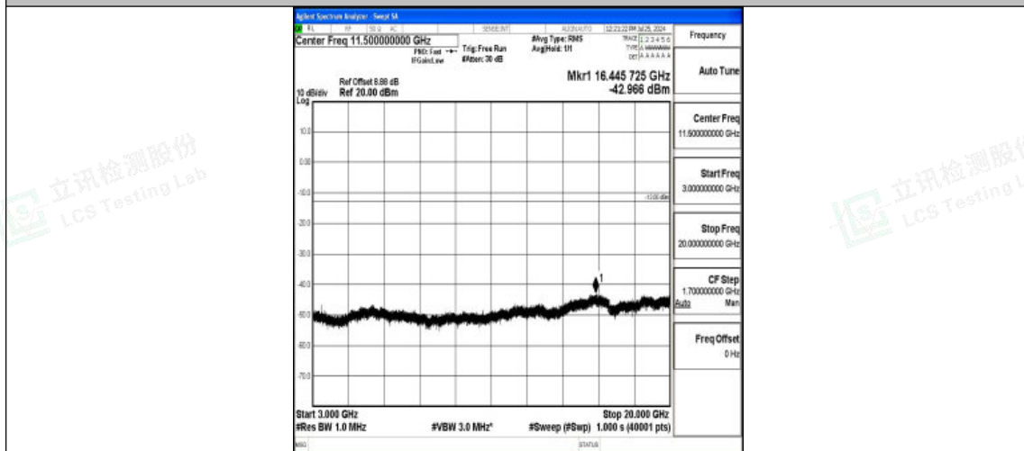
Band4-3MHz-QPSK-20175-1RB#0-3000~20000-PASS
