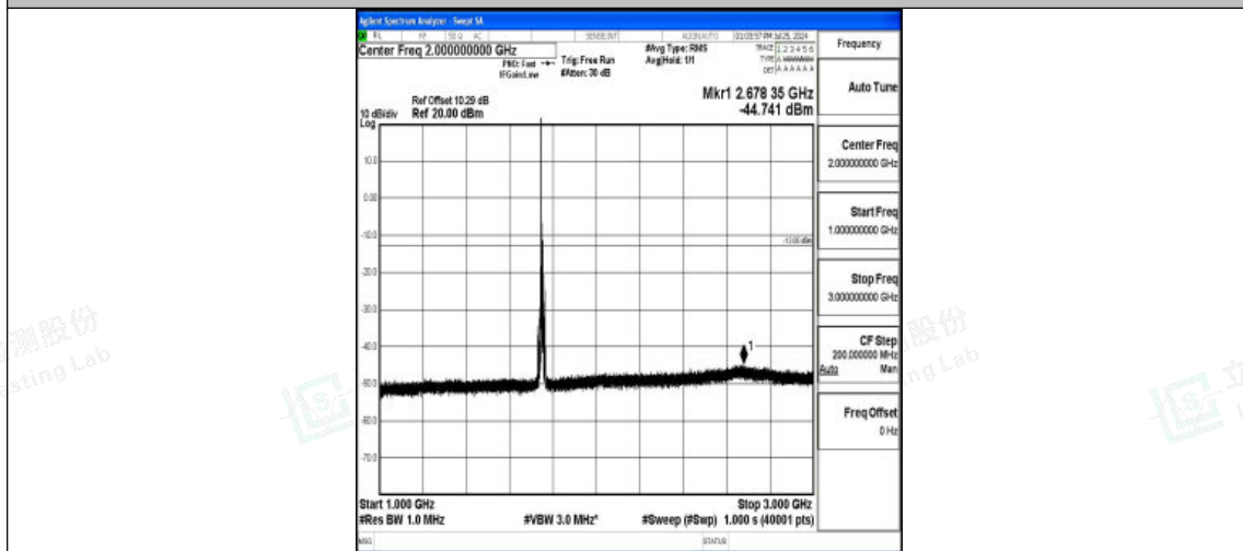
Band4-10MHz-16QAM-20350-1RB#0-1000~3000-PASS
