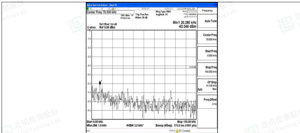
Band4-3MHz-16QAM-20175-1RB#0-0.009~0.15-PASS
