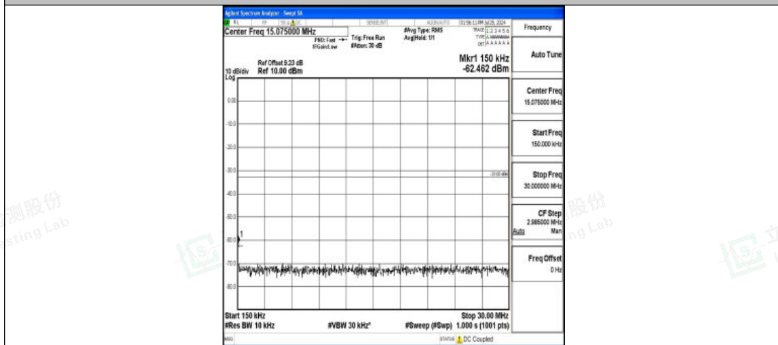
Band4-20MHz-QPSK-20050-1RB#0-0.15~30-PASS
