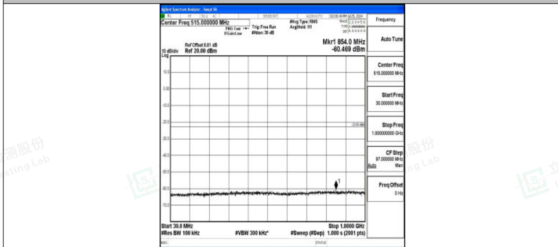
Band4-20MHz-QPSK-20300-1RB#0-30~1000-PASS
