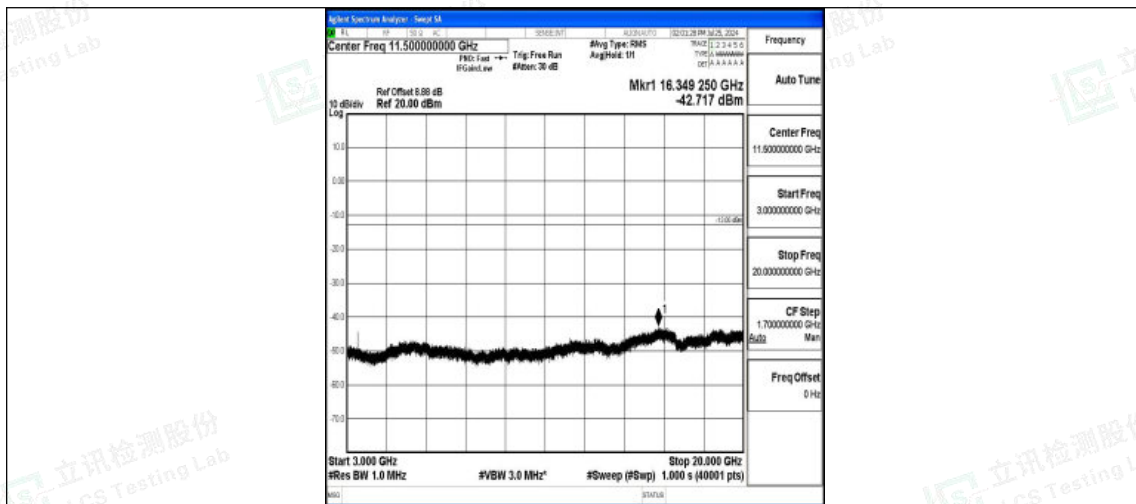
Band4-20MHz-QPSK-20300-1RB#0-3000~20000-PASS
