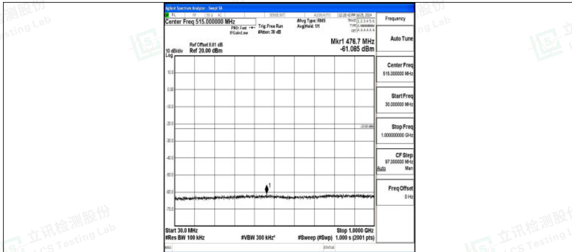
Band4-3MHz-QPSK-20175-1RB#0-30~1000-PASS
