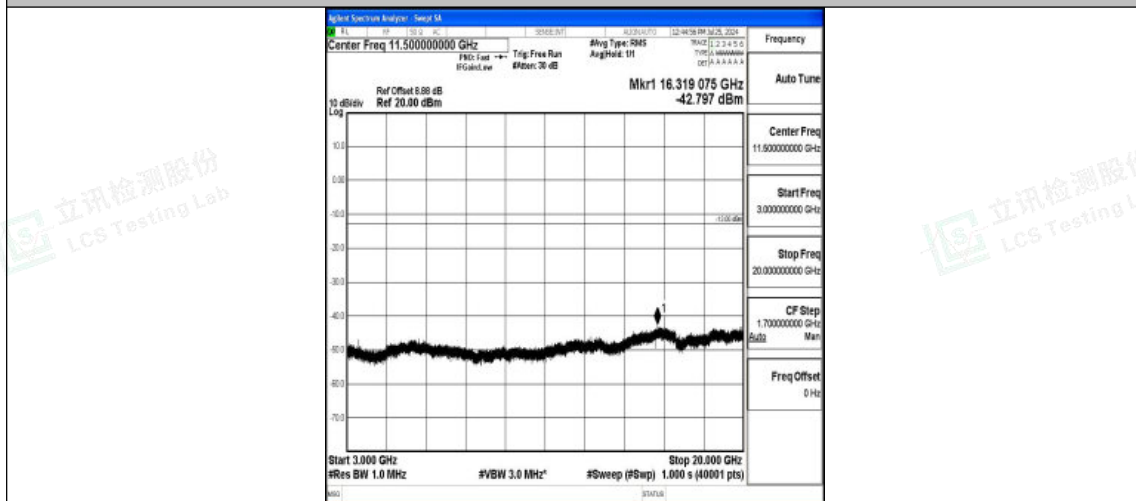
Band4-5MHz-16QAM-20375-1RB#0-3000~20000-PASS
