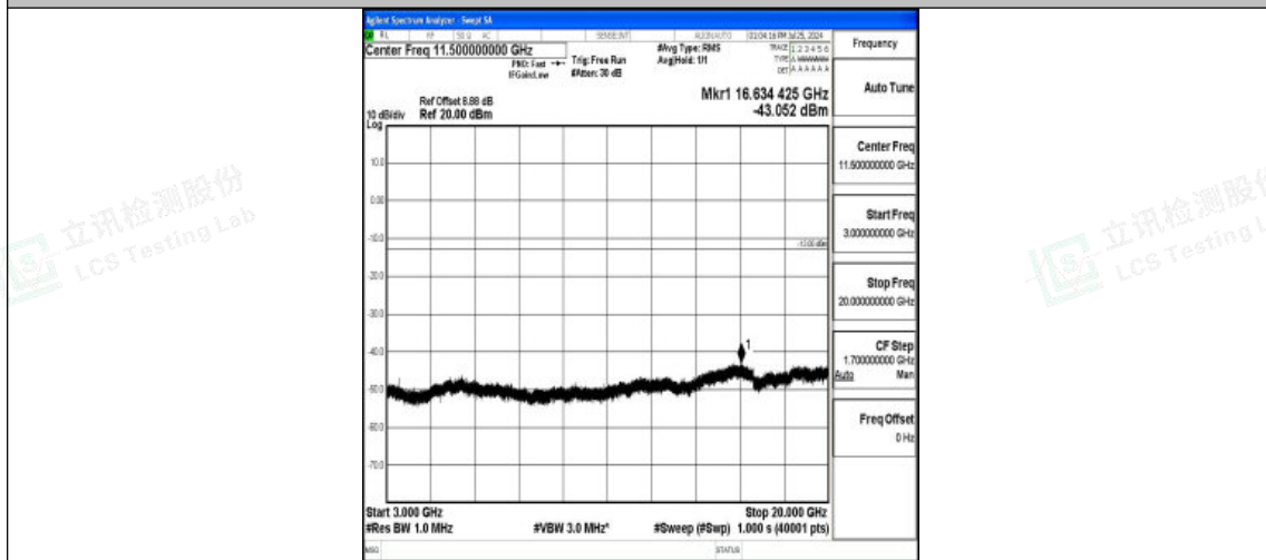
Band4-10MHz-16QAM-20350-1RB#0-3000~20000-PASS
