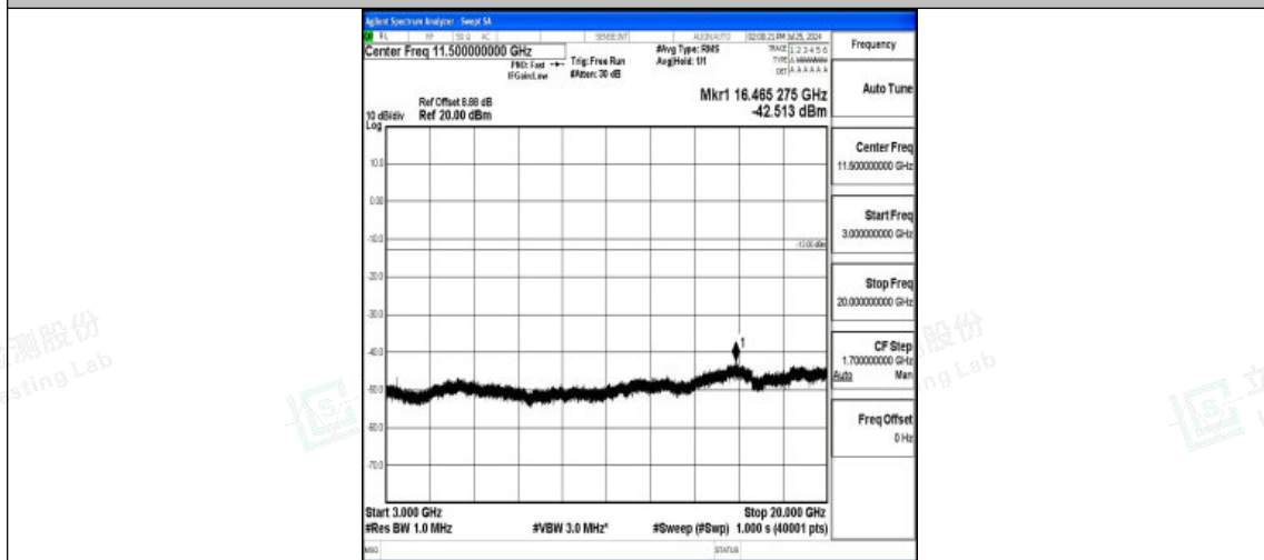
Band4-20MHz-16QAM-20175-1RB#0-3000~20000-PASS
