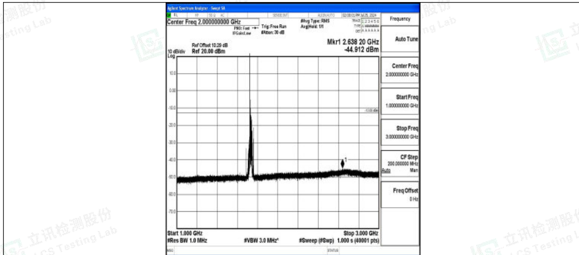
Band4-20MHz-16QAM-20175-1RB#0-1000~3000-PASS
