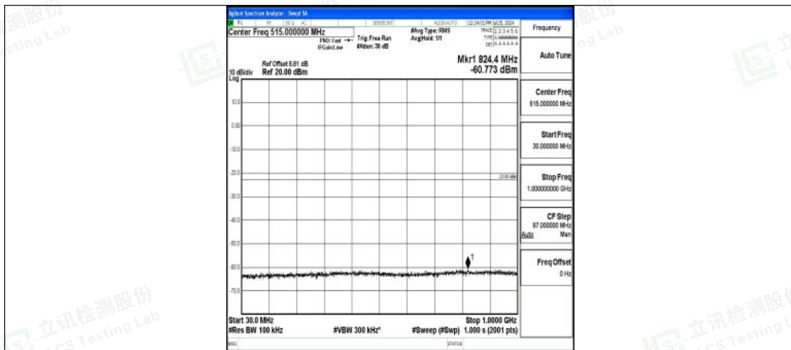
Band4-3MHz-16QAM-20385-1RB#0-30~1000-PASS
