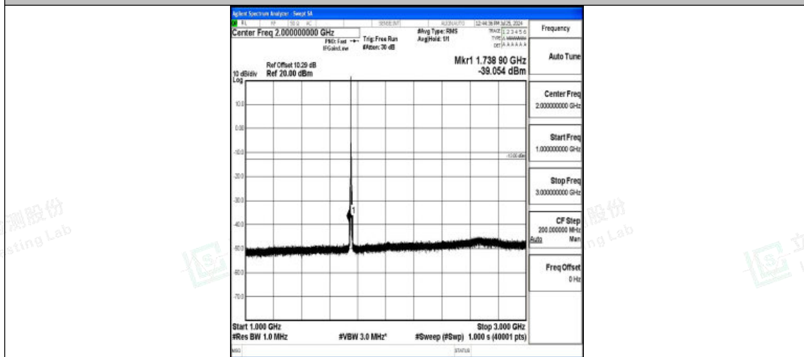
Band4-5MHz-16QAM-20375-1RB#0-1000~3000-PASS
