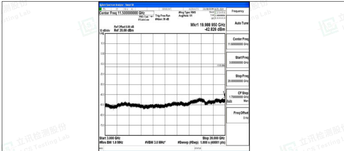
Band4-20MHz-16QAM-20050-1RB#0-3000~20000-PASS
