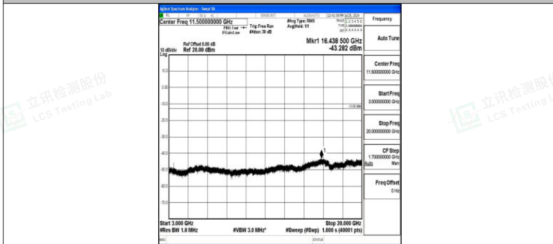
Band4-5MHz-QPSK-20175-1RB#0-3000~20000-PASS
