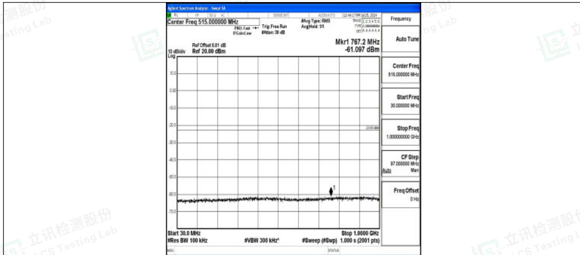
Band4-5MHz-16QAM-20375-1RB#0-30~1000-PASS
