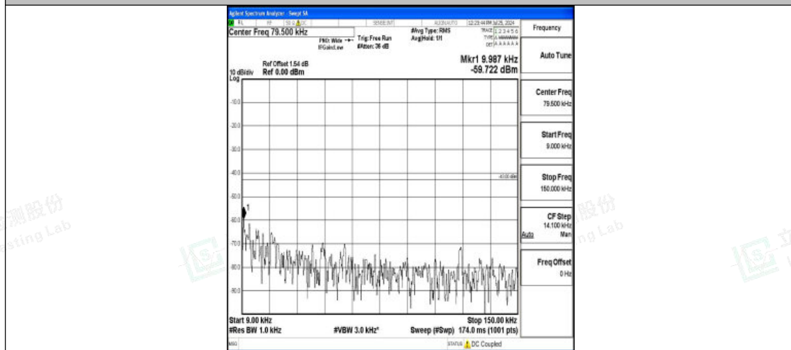
Band4-3MHz-16QAM-20385-1RB#0-0.009~0.15-PASS
