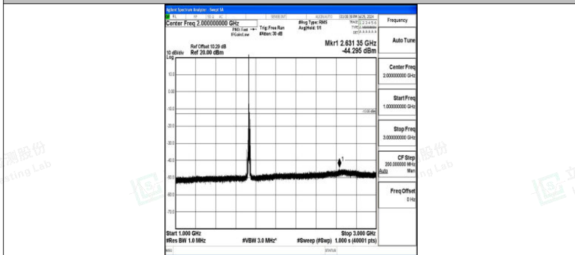
Band4-10MHz-QPSK-20175-1RB#0-1000~3000-PASS
