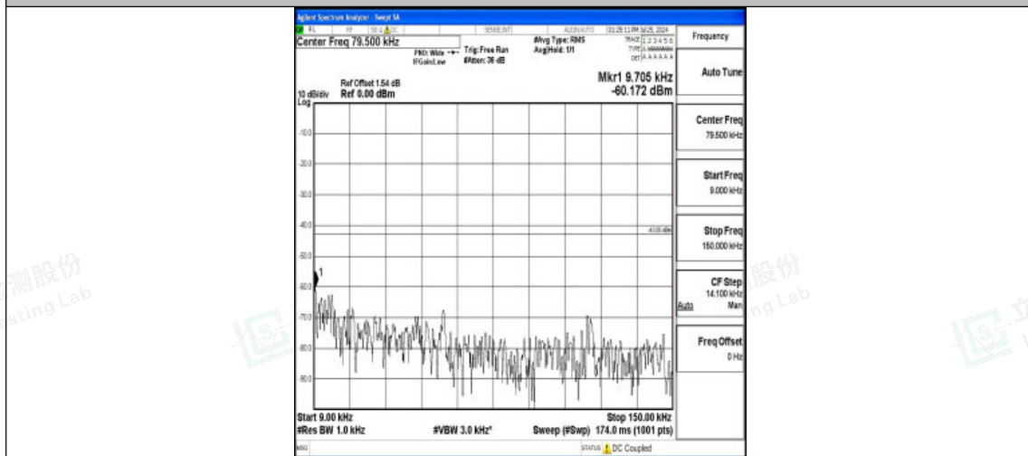
Band4-15MHz-QPSK-20175-1RB#0-0.009~0.15-PASS
