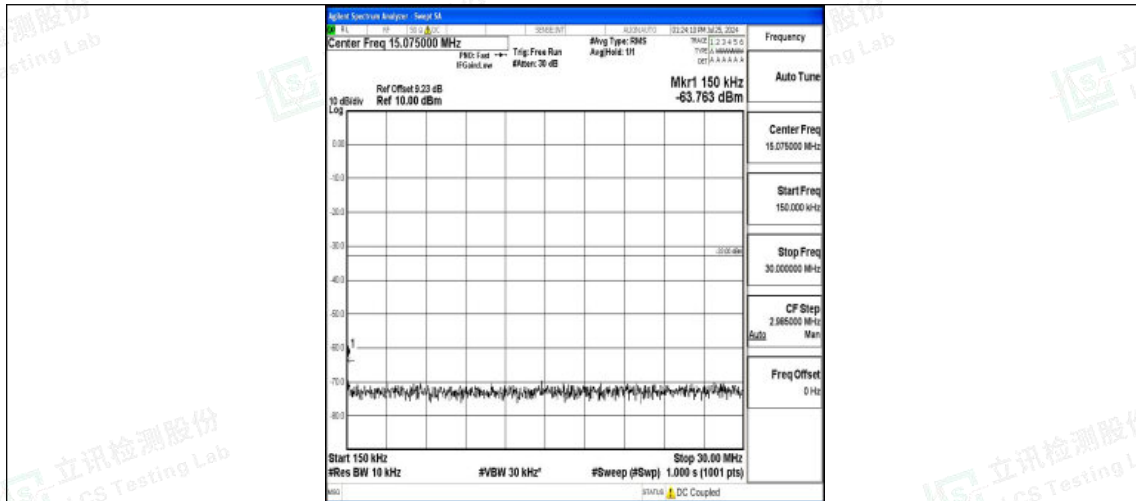
Band4-15MHz-16QAM-20025-1RB#0-0.15~30-PASS
