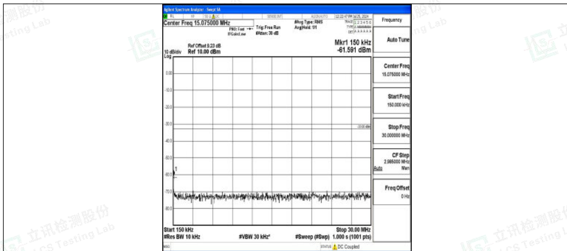
Band4-3MHz-QPSK-20385-1RB#0-0.15~30-PASS
