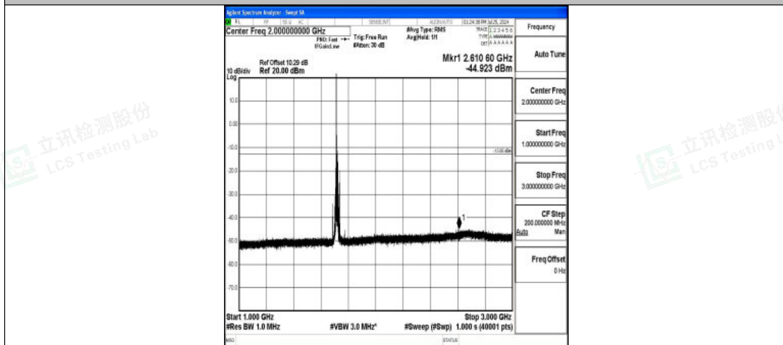
Band4-15MHz-16QAM-20025-1RB#0-1000~3000-PASS
