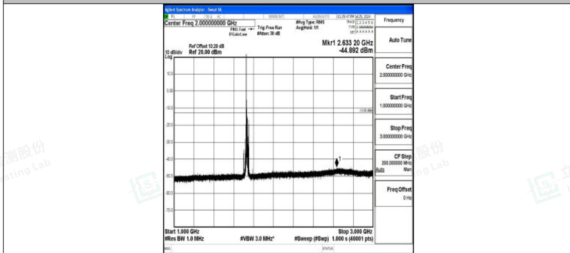
Band4-15MHz-QPSK-20175-1RB#0-1000~3000-PASS
