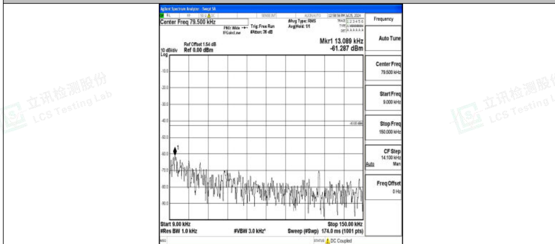
Band4-10MHz-16QAM-20000-1RB#0-0.009~0.15-PASS
