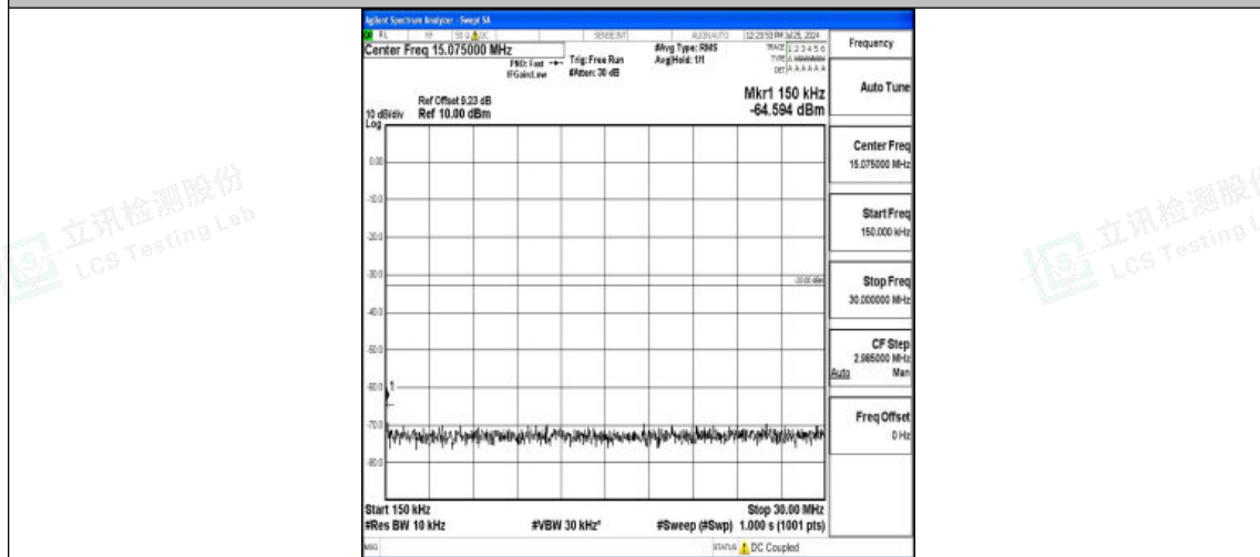
Band4-3MHz-16QAM-20385-1RB#0-0.15~30-PASS
