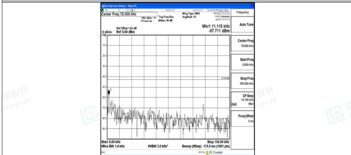
Band4-1.4MHz-16QAM-20393-1RB#0-0.009~0.15-PASS
