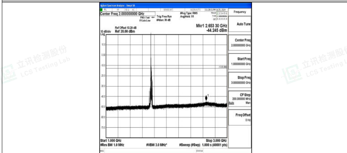
Band4-15MHz-QPSK-20325-1RB#0-1000~3000-PASS
