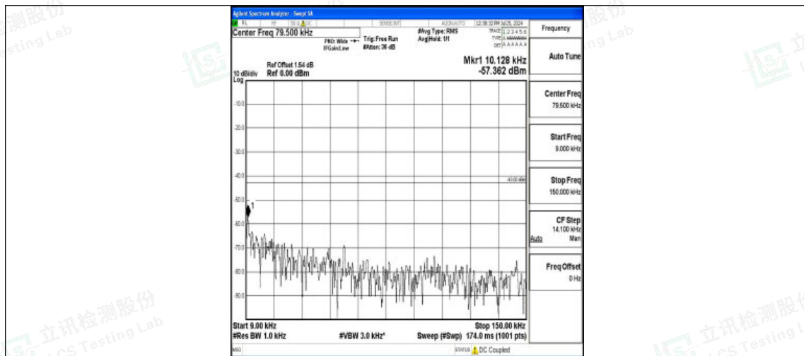
Band4-5MHz-QPSK-19975-1RB#0-0.009~0.15-PASS
