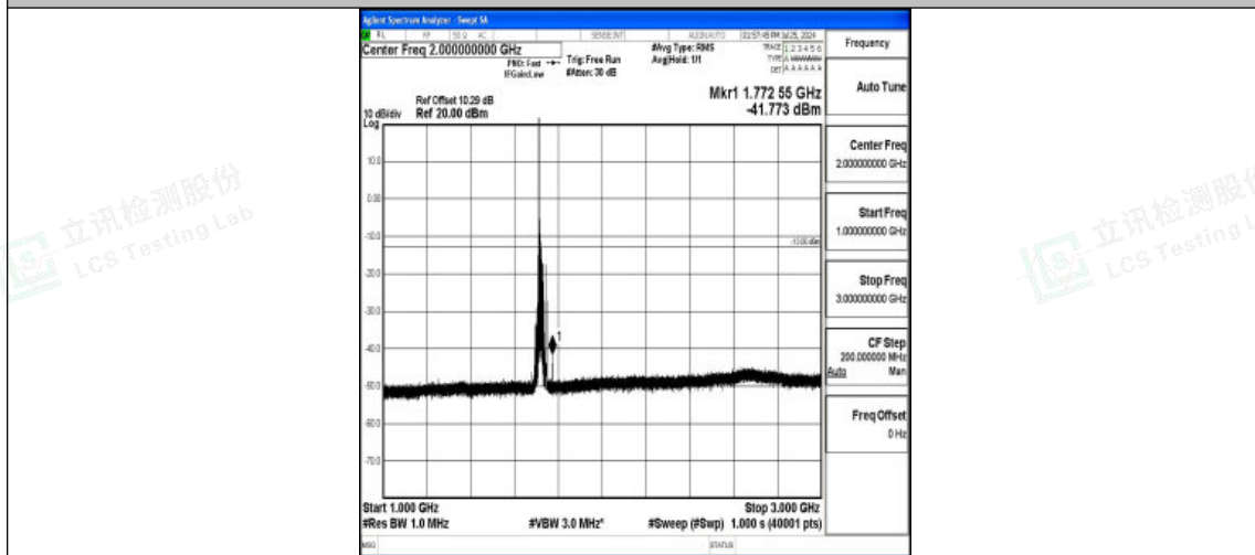
Band4-20MHz-16QAM-20050-1RB#0-1000~3000-PASS
