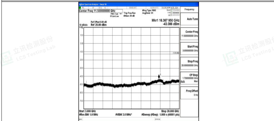
Band4-15MHz-16QAM-20325-1RB#0-3000~20000-PASS
