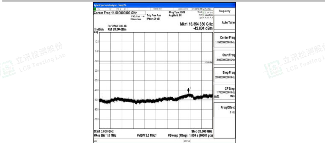
Band4-10MHz-QPSK-20175-1RB#0-3000~20000-PASS
