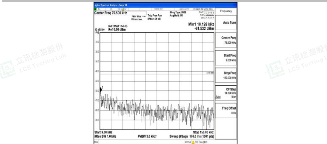
Band4-15MHz-16QAM-20025-1RB#0-0.009~0.15-PASS
