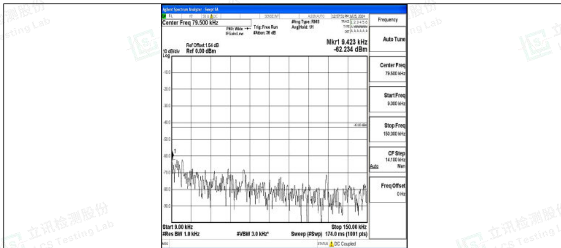
Band4-10MHz-QPSK-20000-1RB#0-0.009~0.15-PASS
