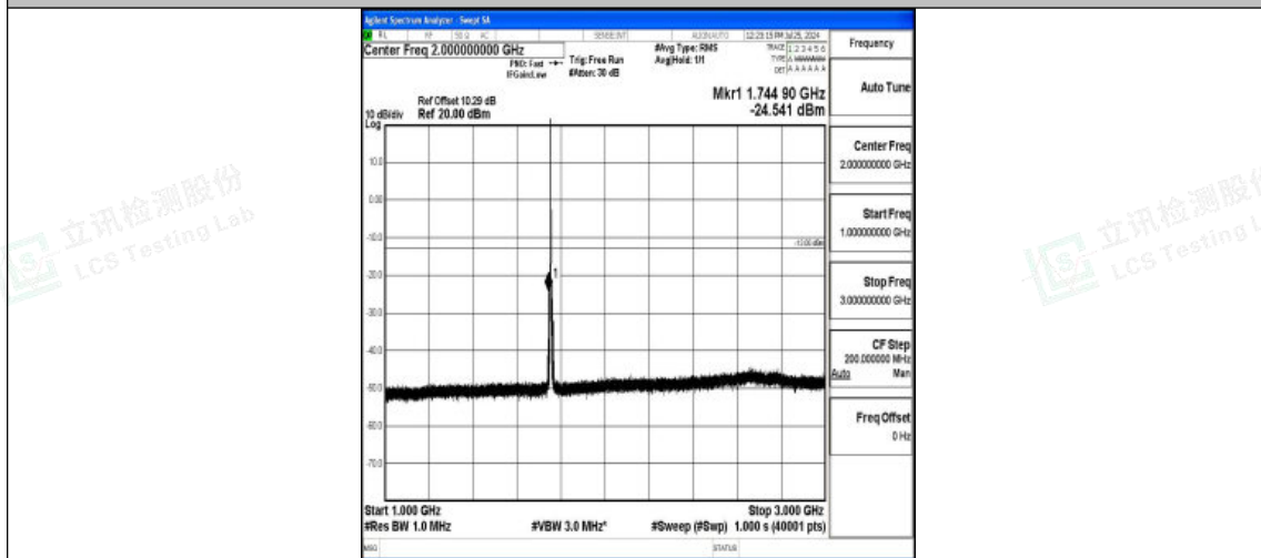
Band4-3MHz-QPSK-20385-1RB#0-1000~3000-PASS
