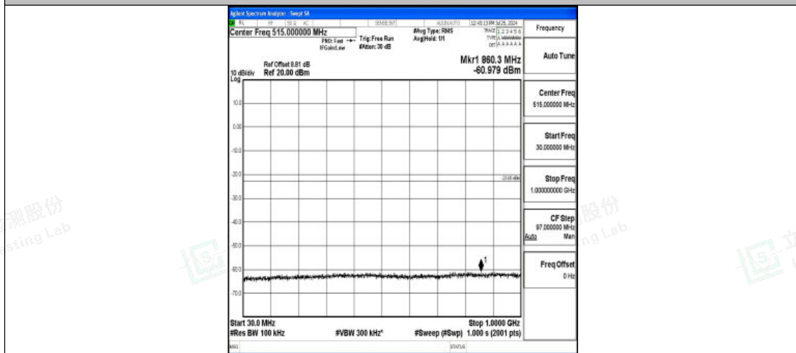
Band4-5MHz-QPSK-20375-1RB#0-30~1000-PASS
