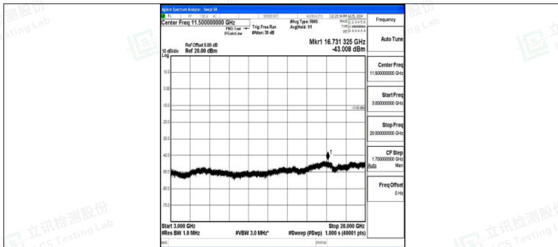
Band4-3MHz-QPSK-20385-1RB#0-3000~20000-PASS
