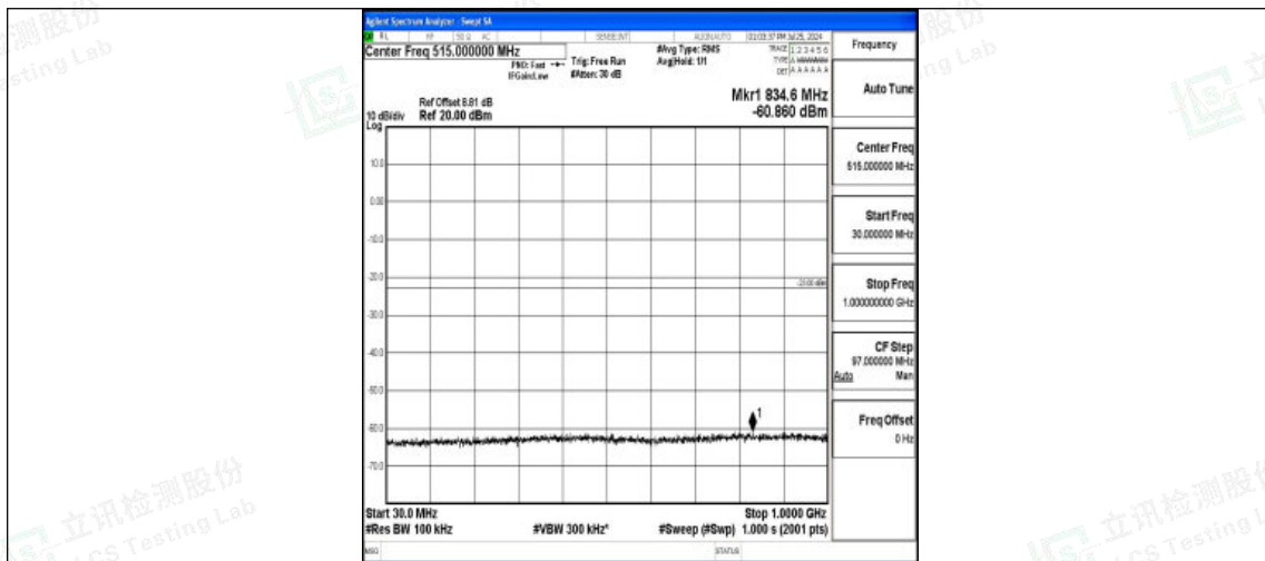
Band4-10MHz-16QAM-20350-1RB#0-30~1000-PASS
