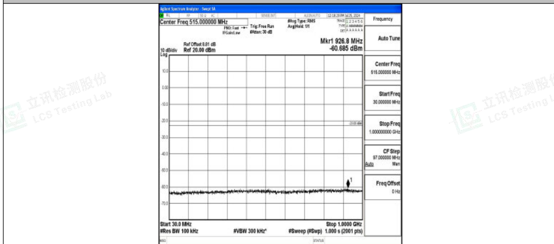
Band4-3MHz-QPSK-19965-1RB#0-30~1000-PASS
