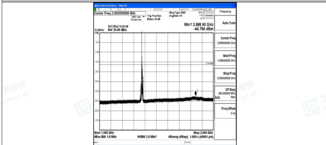
Band4-15MHz-16QAM-20325-1RB#0-1000~3000-PASS
