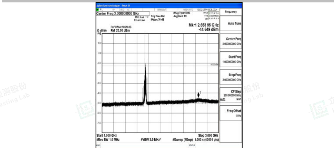
Band4-20MHz-16QAM-20300-1RB#0-1000~3000-PASS
