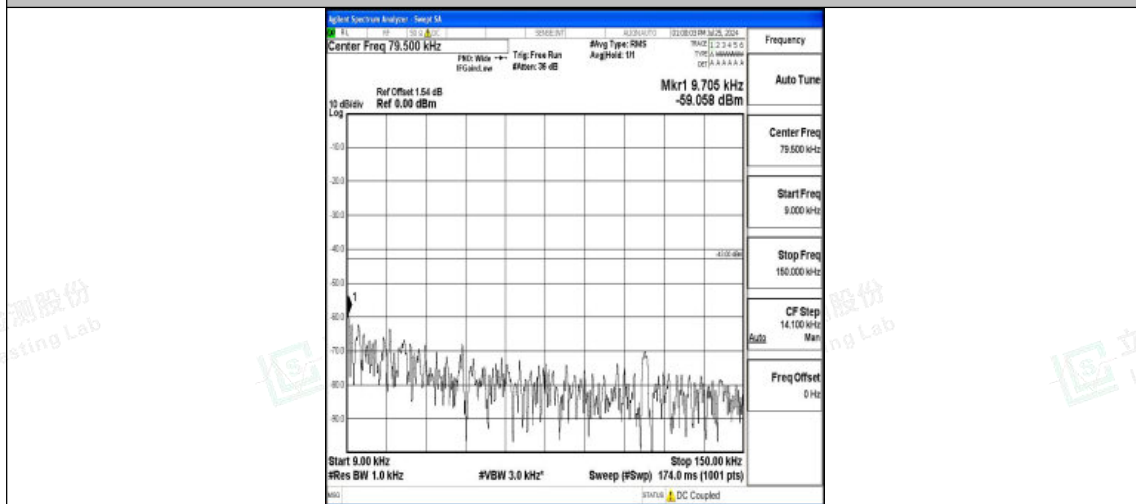
Band4-10MHz-QPSK-20175-1RB#0-0.009~0.15-PASS
