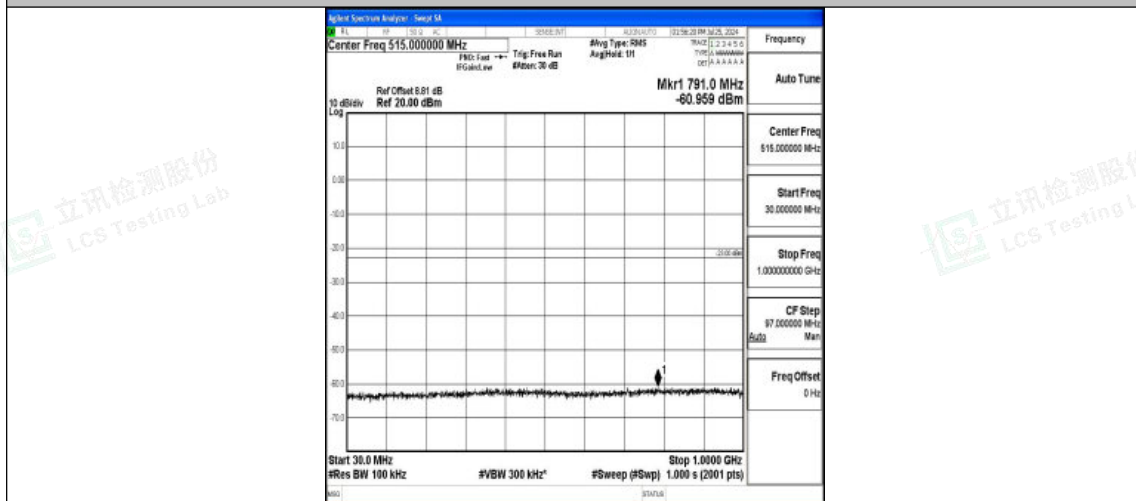
Band4-20MHz-QPSK-20050-1RB#0-30~1000-PASS
