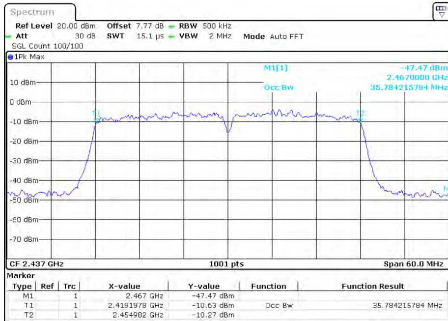
OBW NVNT n40 2437MHz Ant1
