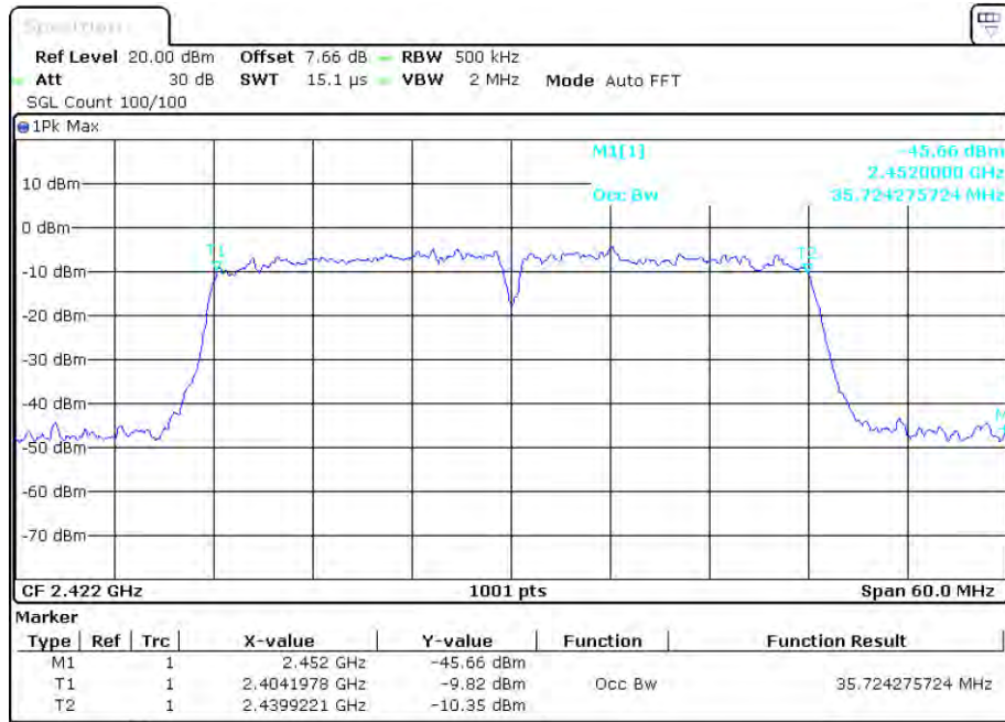
OBW NVNT n40 2422MHz Ant1
