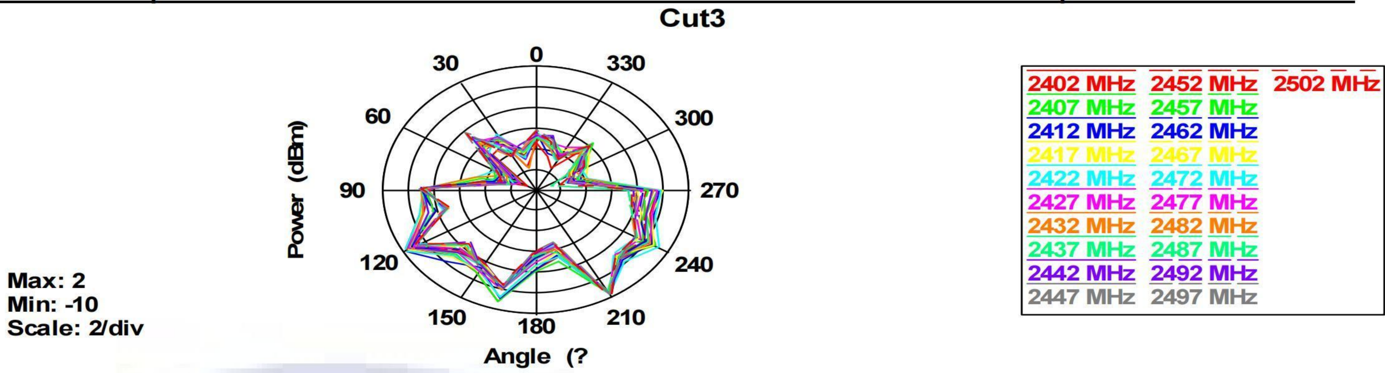
2402MHz ~2502 MHz Wi-Fi 2.4G 3D Gain
