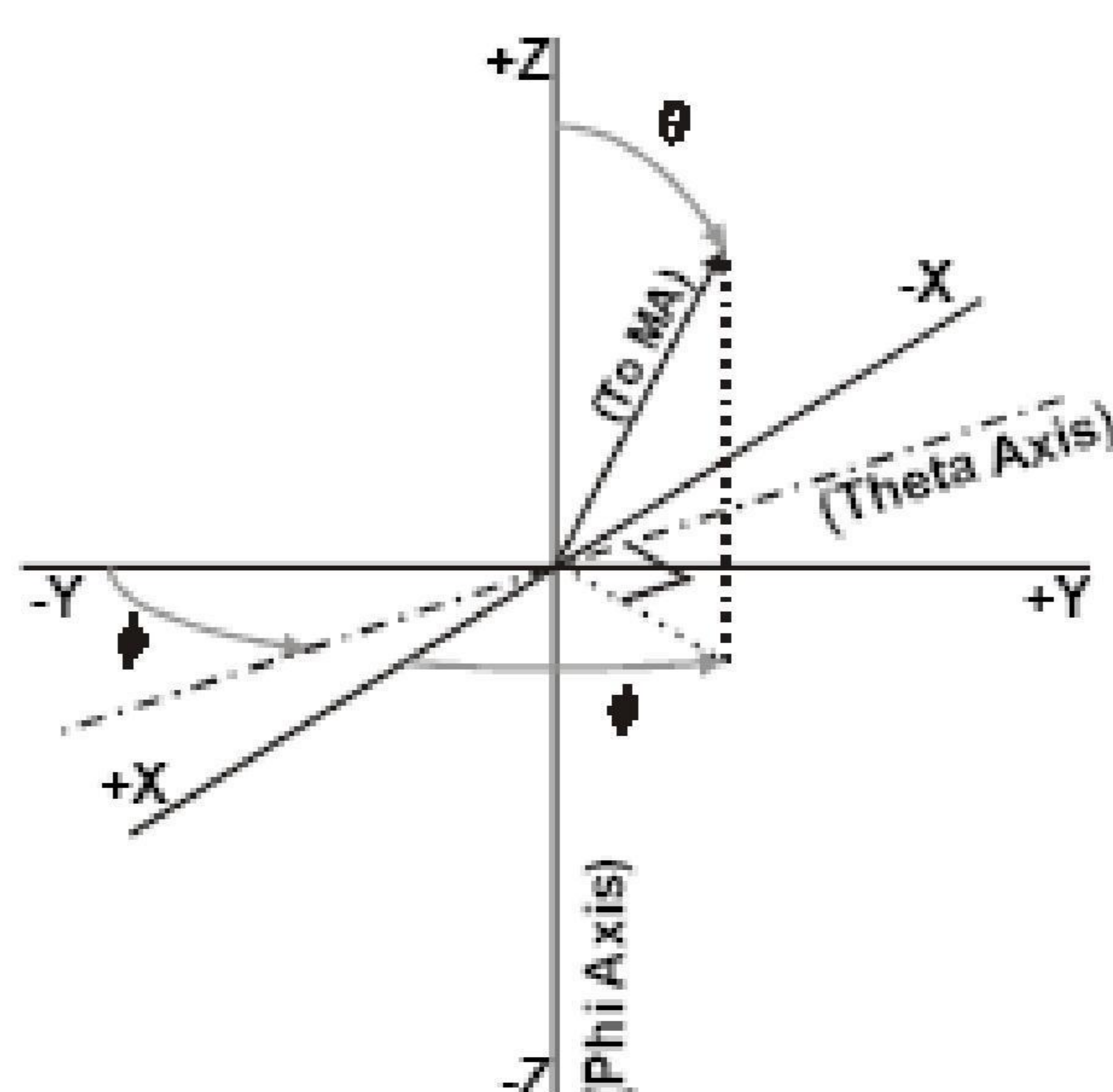
Figure 1 Test coordinate system
