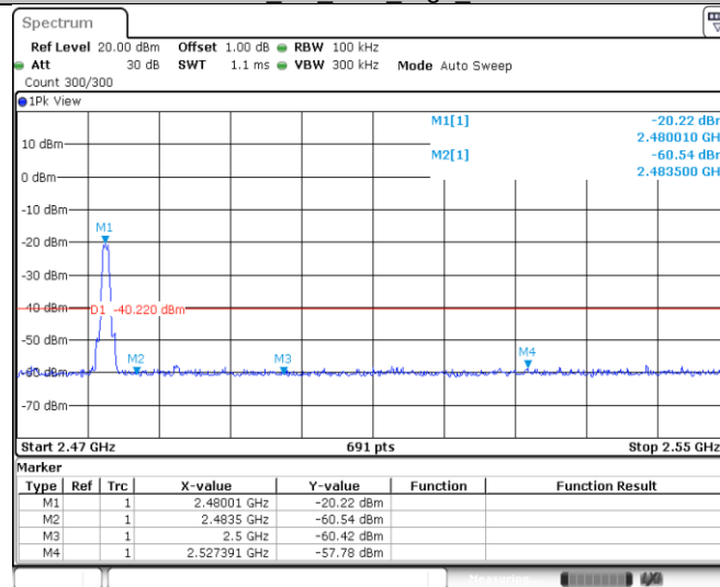
BLE_1M_Ant1_High_2480
