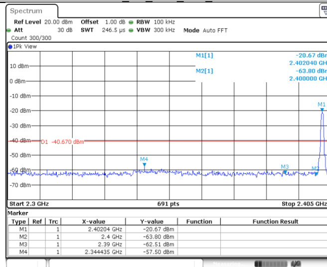
BLE_1M_Ant1_Low_2402
