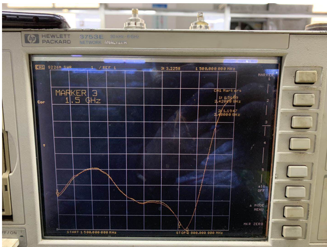
Standing wave ratio diagram of BT antenna
