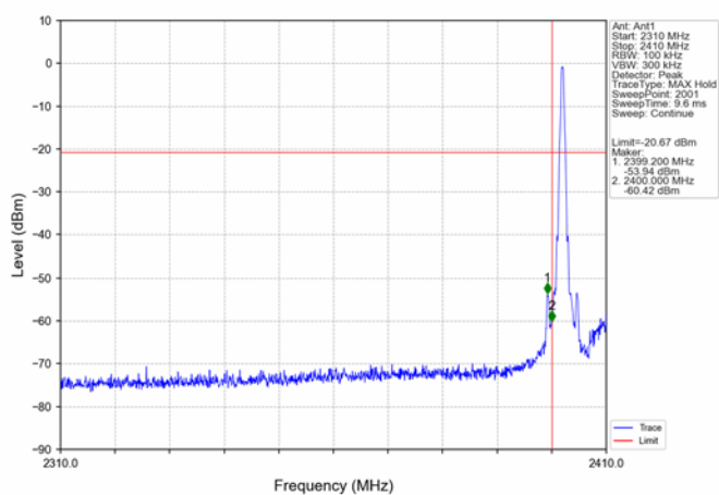
GFSK_DH5_LCH_2402MHz_Ant1_NTNV
