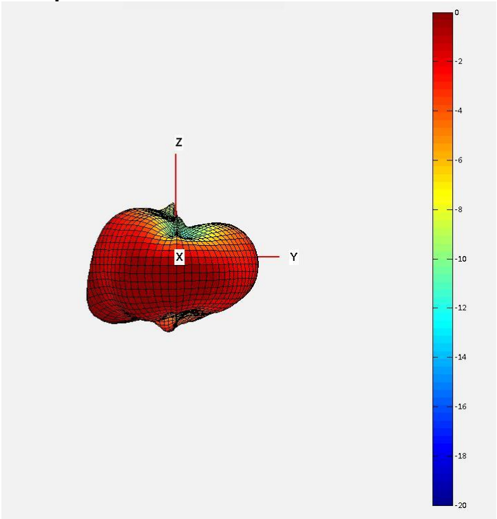
2450MHz Y-Z plane
