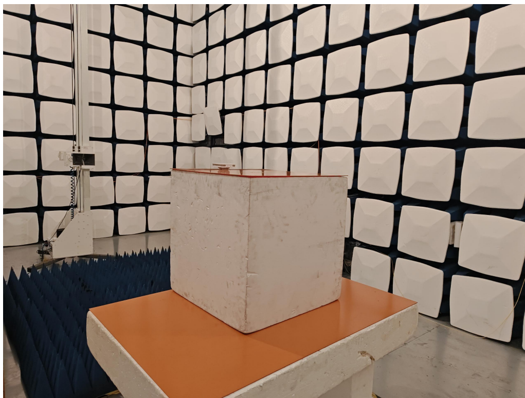
Test Setup Photo(s) of 20dB Bandwidth & 99% Occupied Bandwidth
