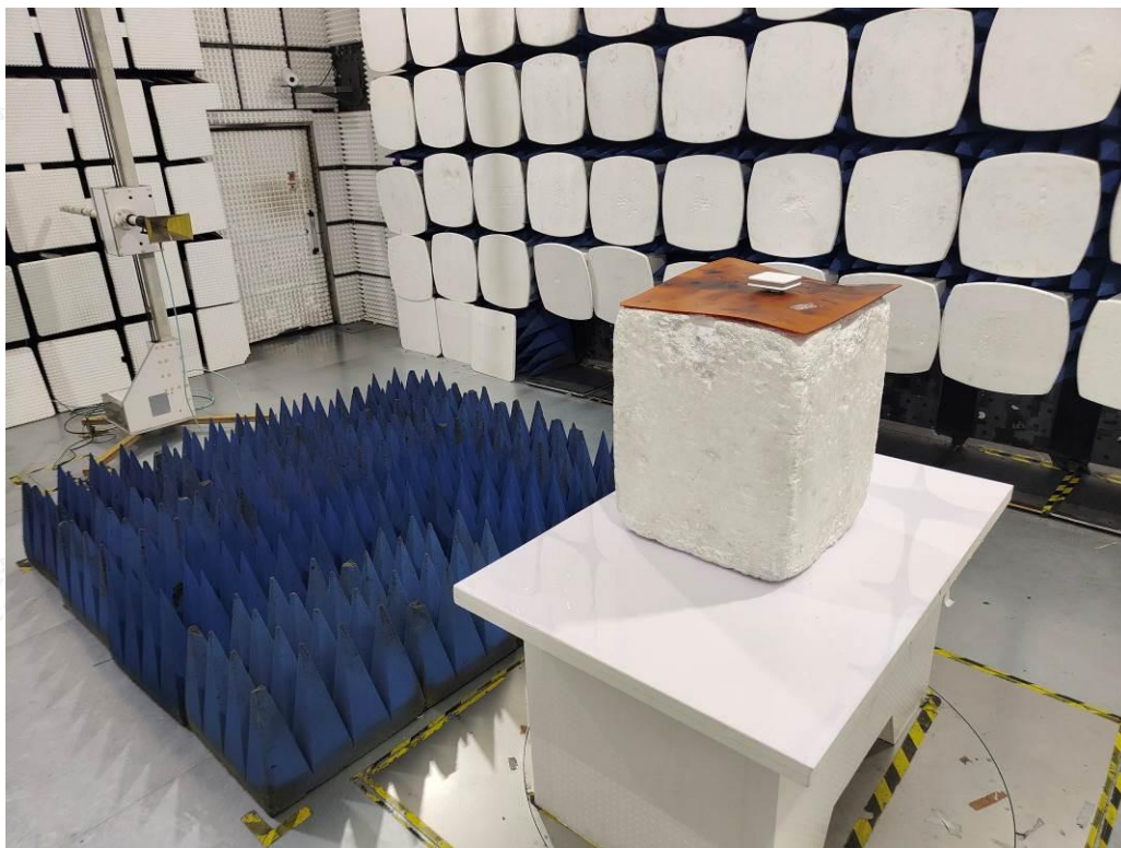
Fig. 3 (Above1GHz)
