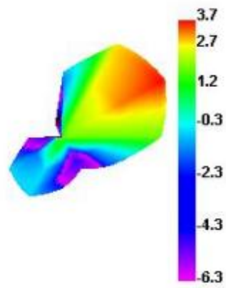
Bluetooth 37 TRP
