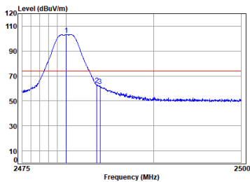
BLE_2M_TX_CH_39_Vertical-Peak
