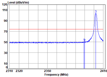
BLE_1M_TX_CH_00_Horizontal-Peak
