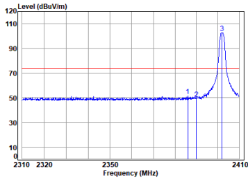
BLE_1M_TX_CH_00_Vertical-Peak
