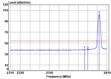
BLE_1M_TX_CH_00_Horizontal-AVG
