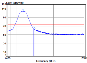
BLE_2M_TX_CH_39_Horizontal-Peak
