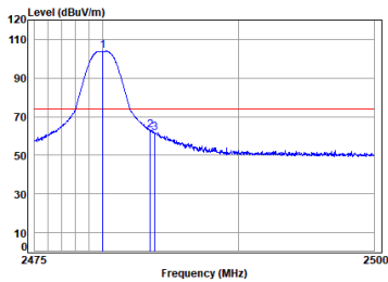
BLE_1M_TX_CH_39_Horizontal-Peak
