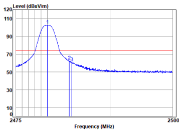
BLE_1M_TX_CH_39_Vertical-Peak
