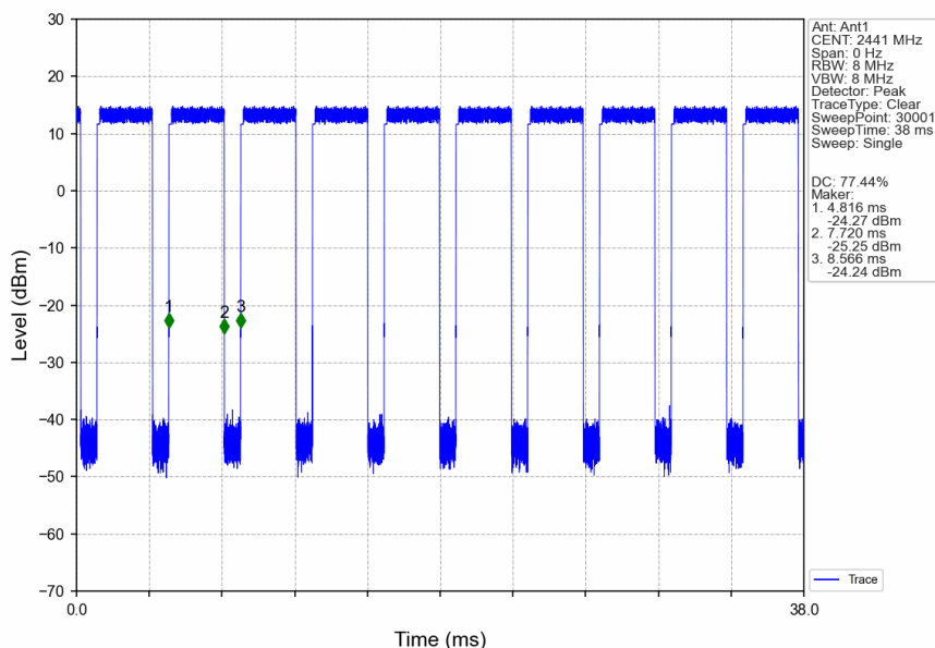
8DPSK_3DH5_MCH_2441MHz_Ant1_NTNV
