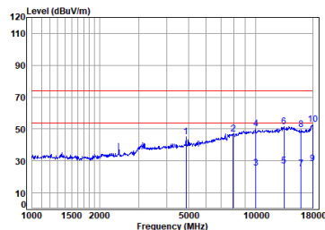
BT_DH5_TX_CH_39_Vertical
