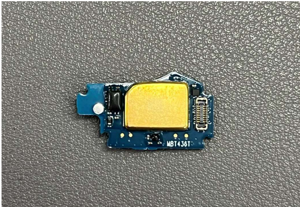
Fig. 6 PCB view 6
