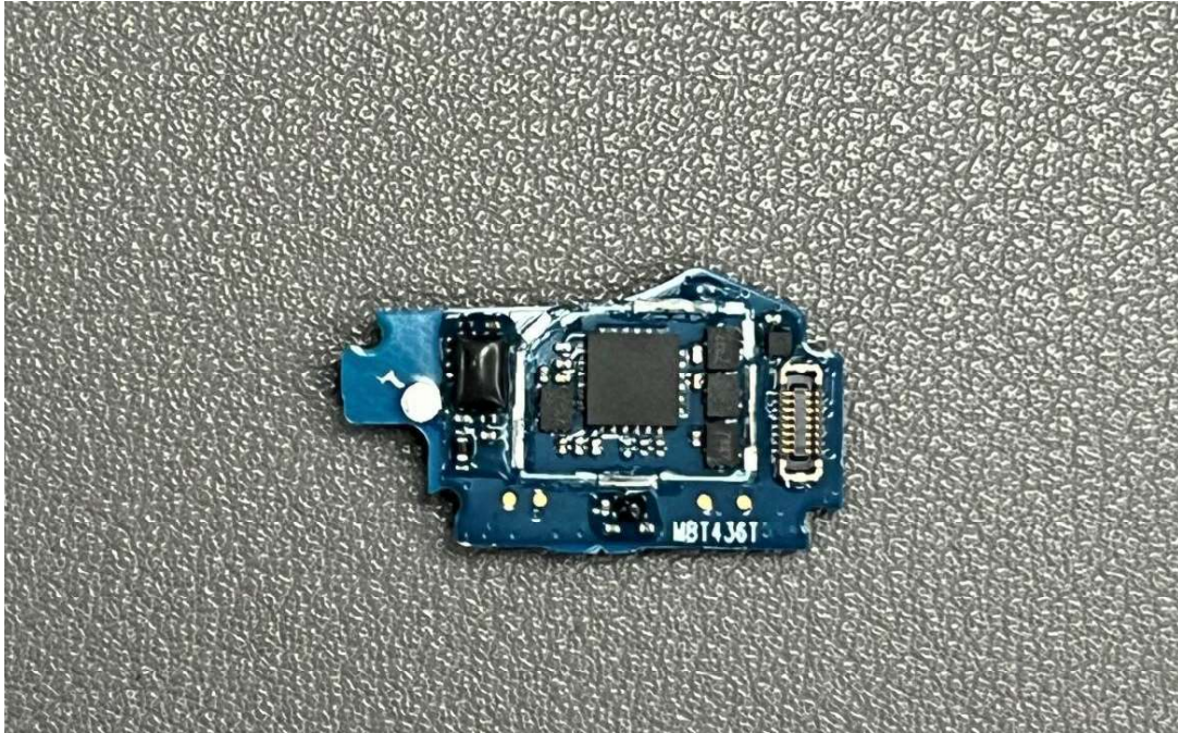
Fig. 7 PCB view 7
