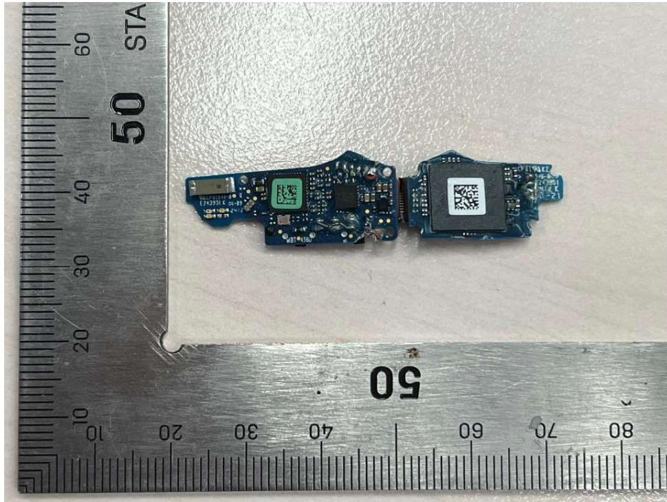
Fig. 1 PCB view 1
