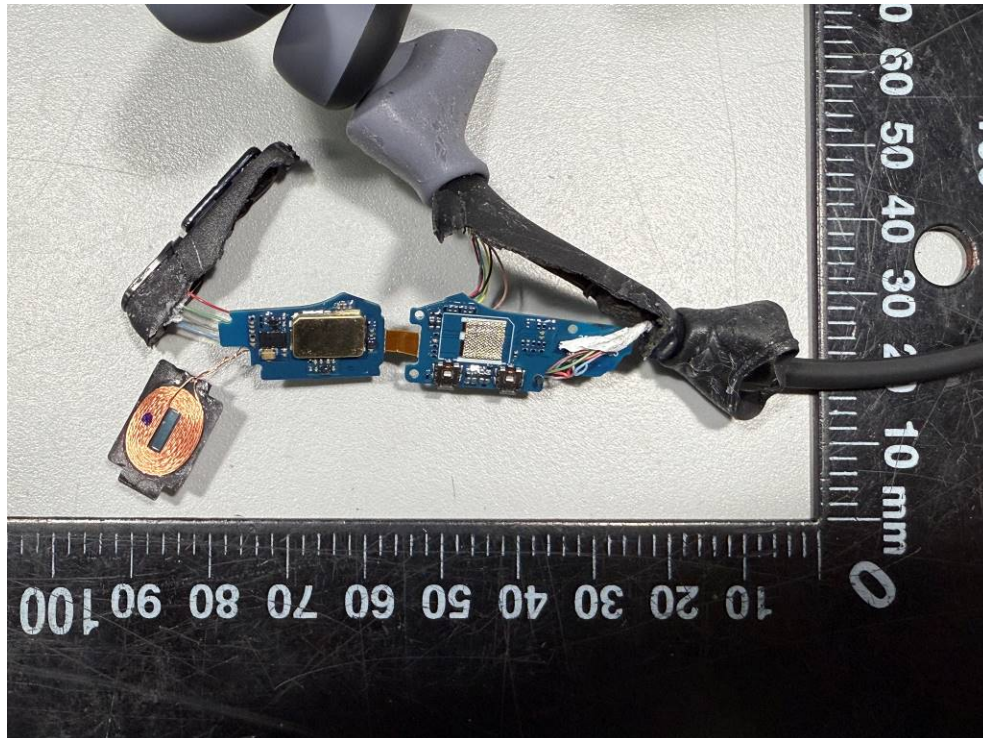
Fig. 7 PCB view 2
