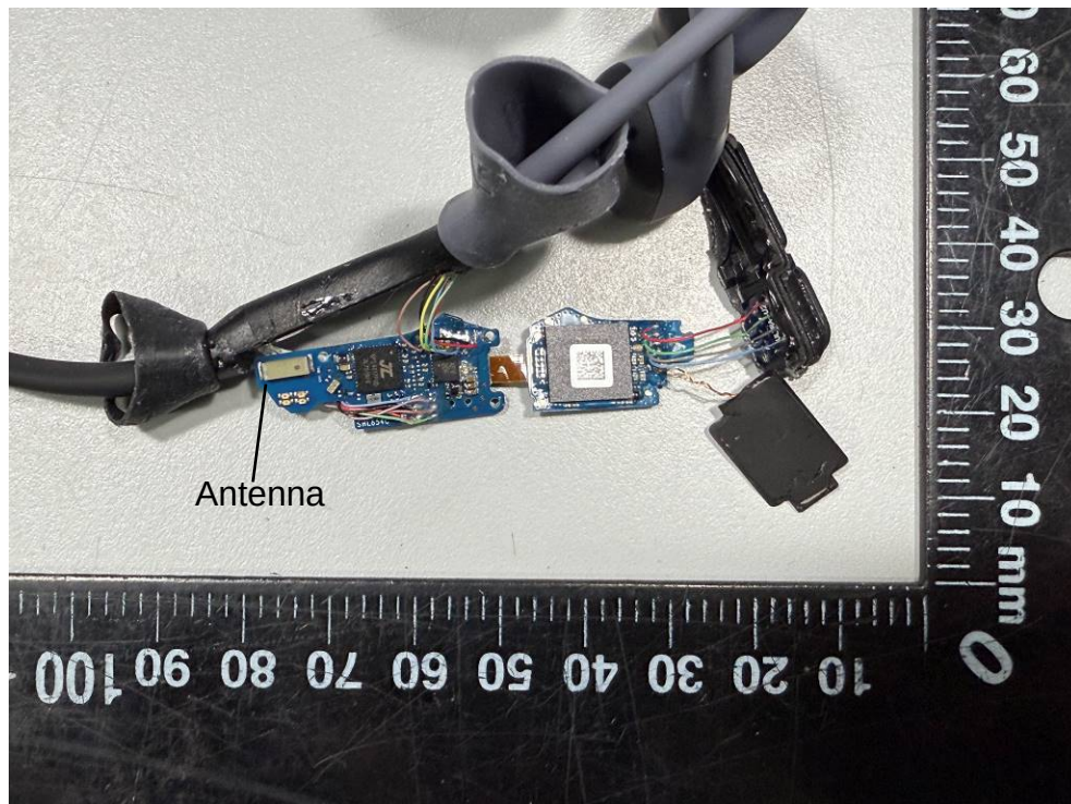
Fig. 6 PCB view 1
