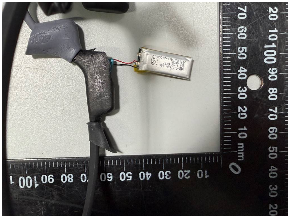
Fig. 8 Battery view
