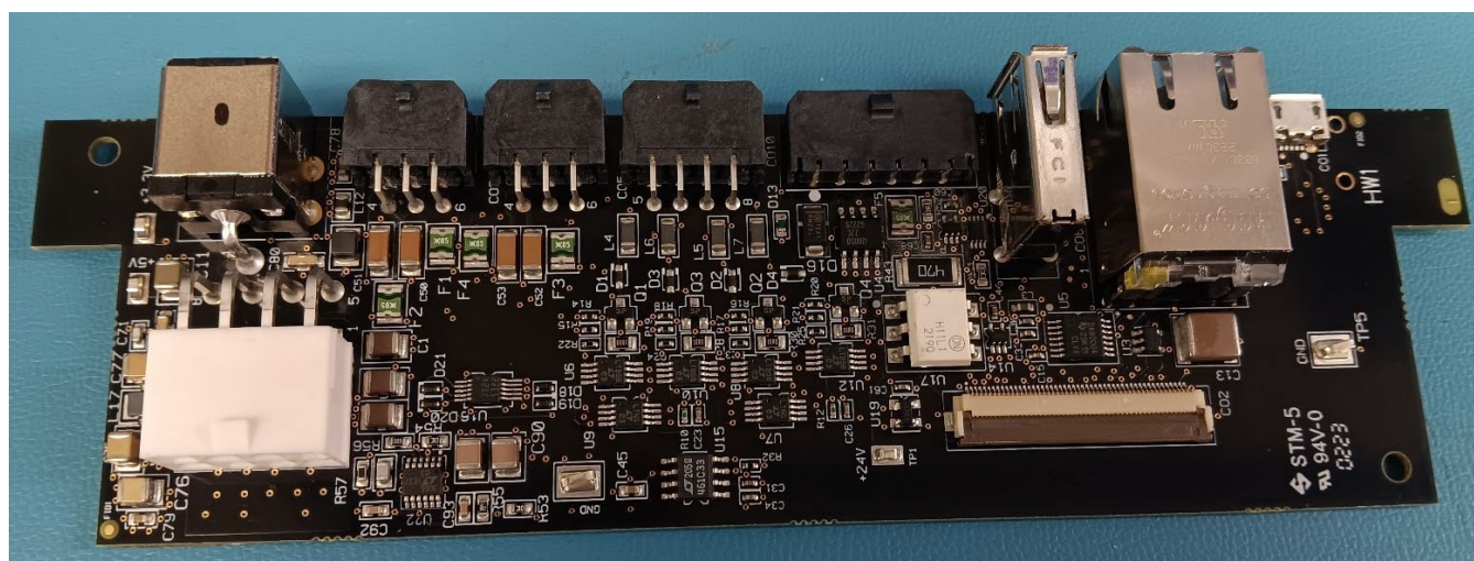
Interface-Connector Side 2
