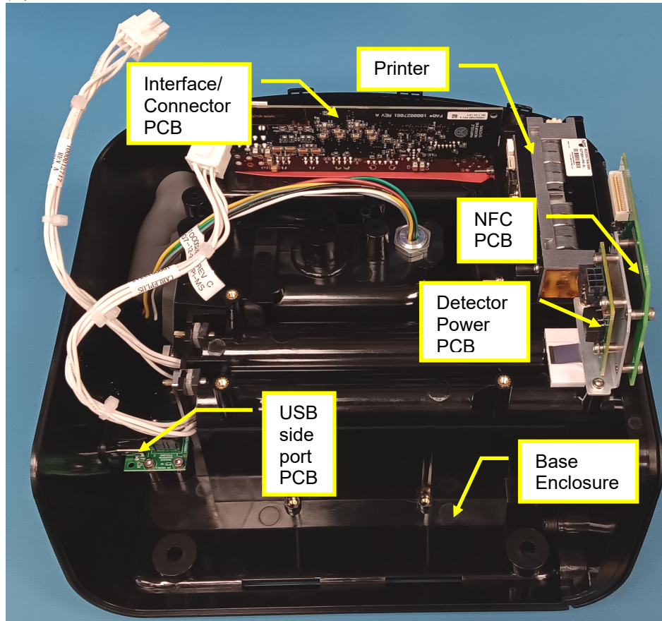
Figure 6 Printed Circuit Boards Installed in Base Enclosure
