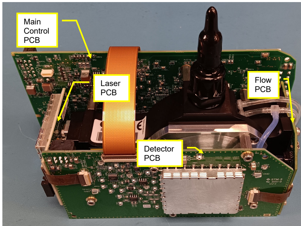
Figure 7 Printed Circuit Boards Installed on Sample Chamber
