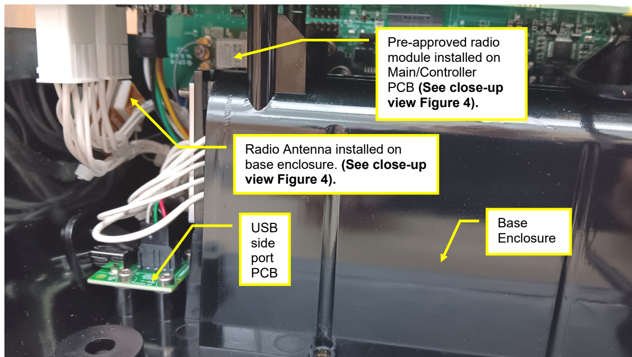
Figure 3 Close up of Figure 2 lower left side showing Pre-approved radio module and Antenna
