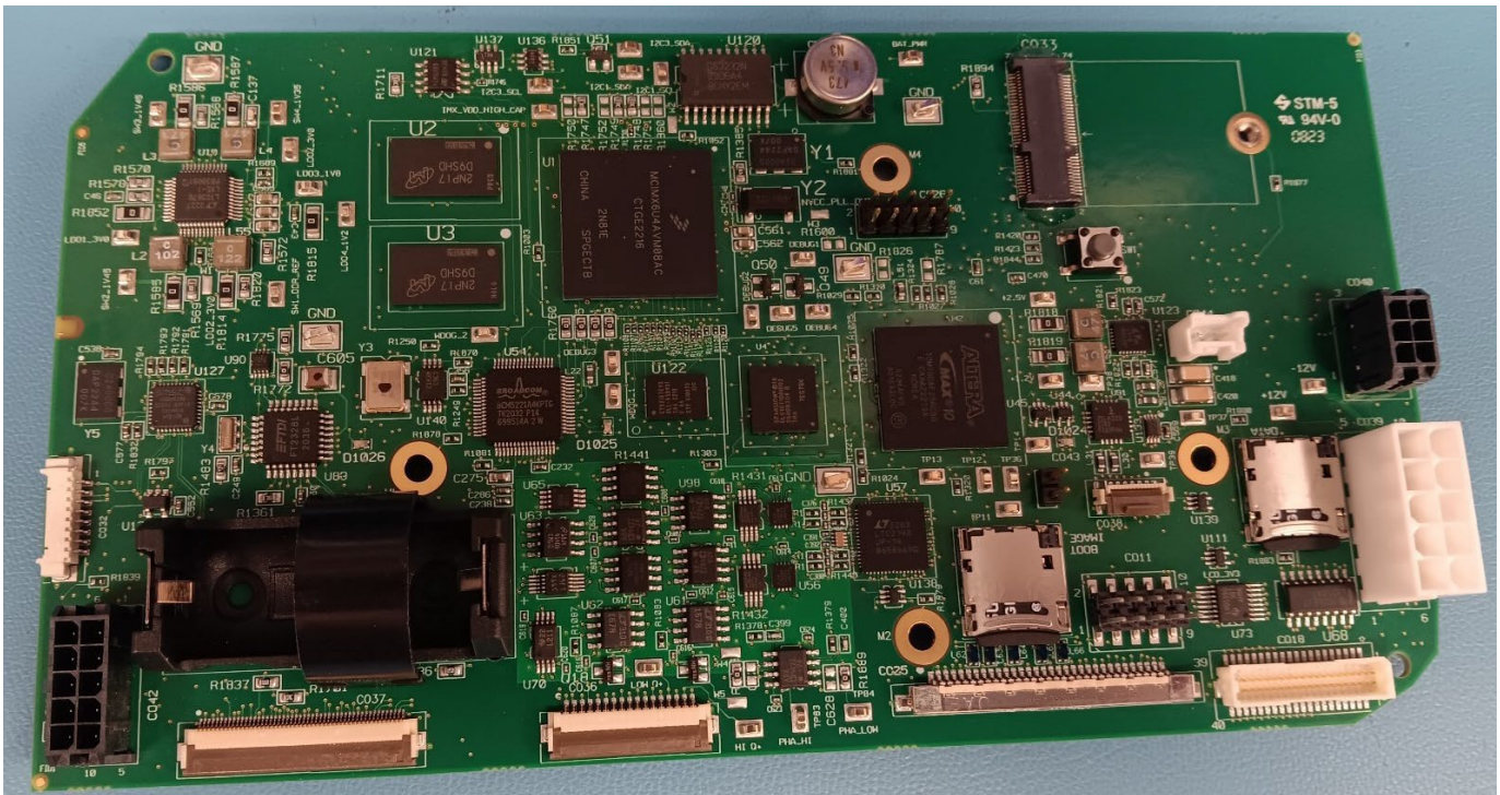
Main-Processor Side 2
