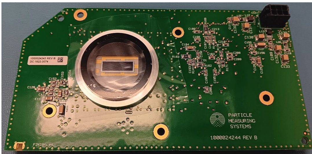
Detector Side 2
