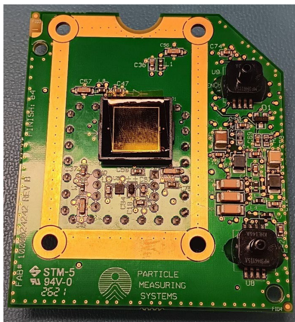
Flow Side 2
