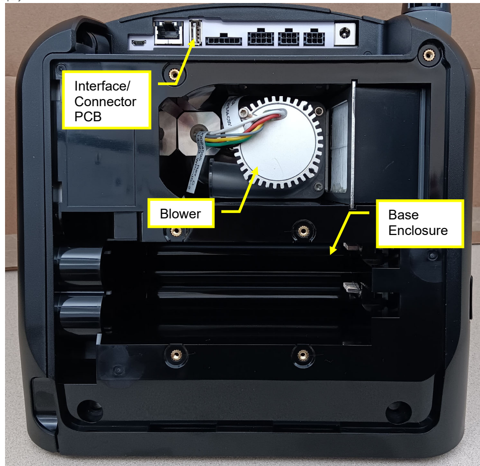
Figure 5 Blower Installed in Base Enclosure – Bottom View
