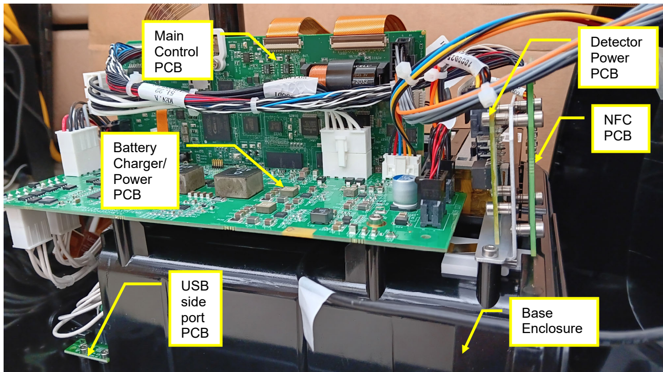
Figure 2 Front View - Base Enclosure with PCBs
