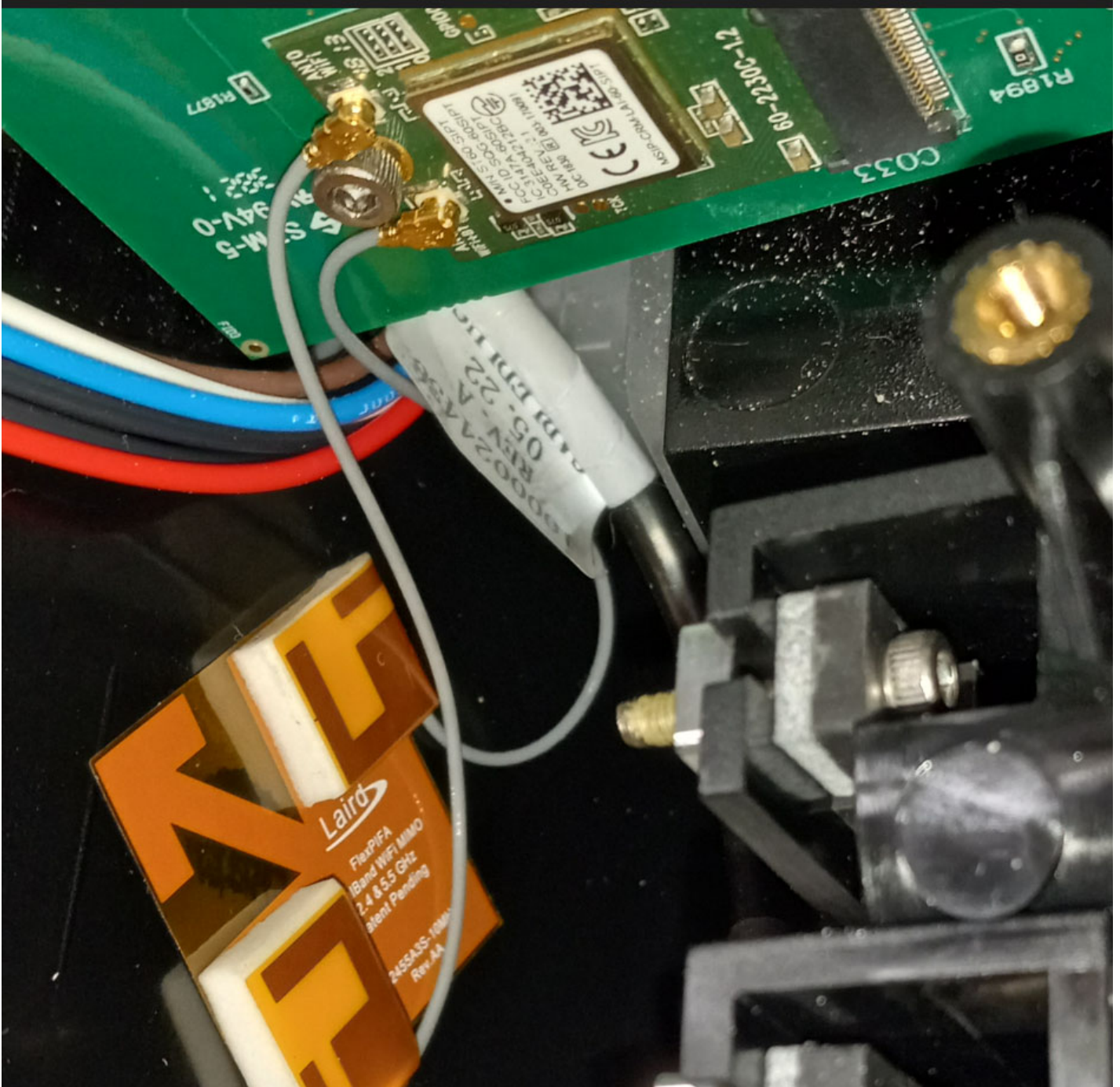
Figure 4 Close up of Figure 2 lower left side showing pre-approved radio module and Antenna
