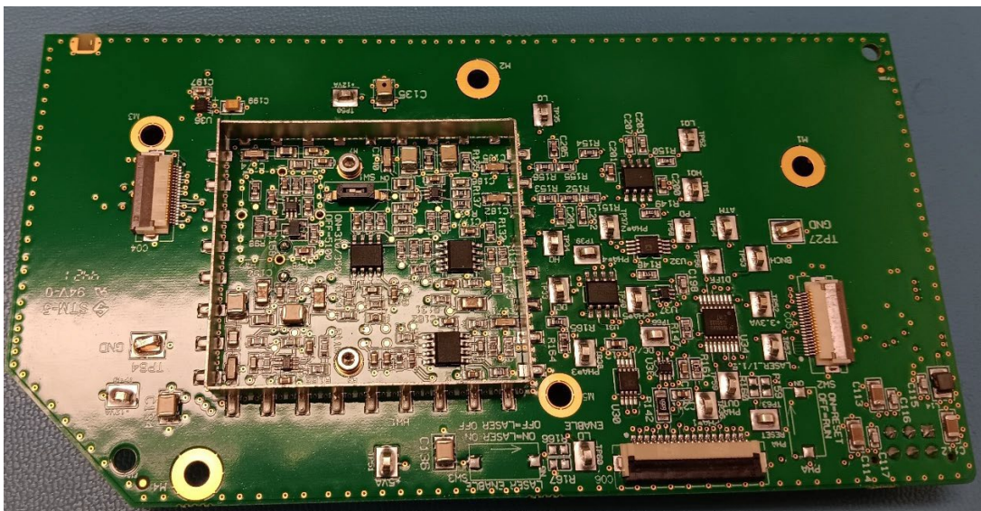
Detector Side 1
