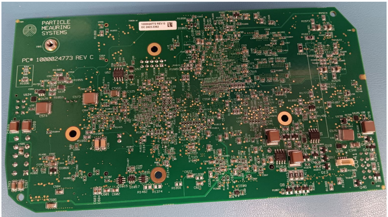
Main-Processor Side 1
