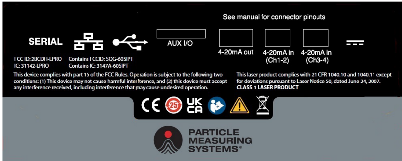
Figure 1 Label with FCC-ISED ID's and verbiage
