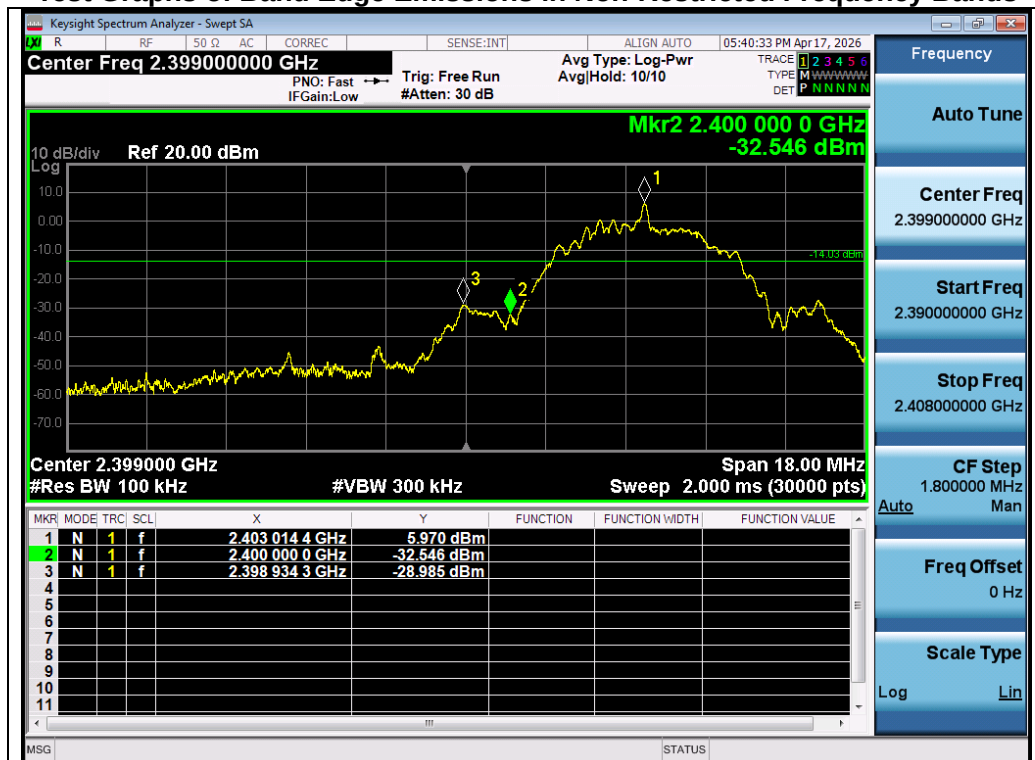
Test_Graph_2.4G_SRD_ANT1_2403_GFSK_Lower Band Edge Emissions
