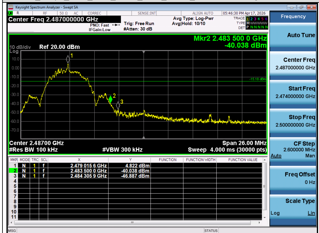
Test_Graph_2.4G_SRD_ANT1_2479_GFSK_Higher Band Edge Emissions
