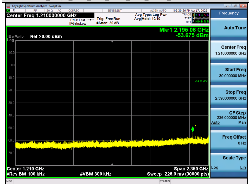
Test_Graph_2.4G_SRD_ANT1_2403_GFSK_Lower Band Emissions
