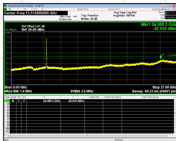
802.11ac80 on channel 155
