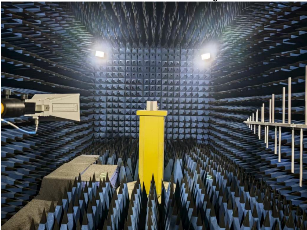
Radiated Emission and Band Edge
