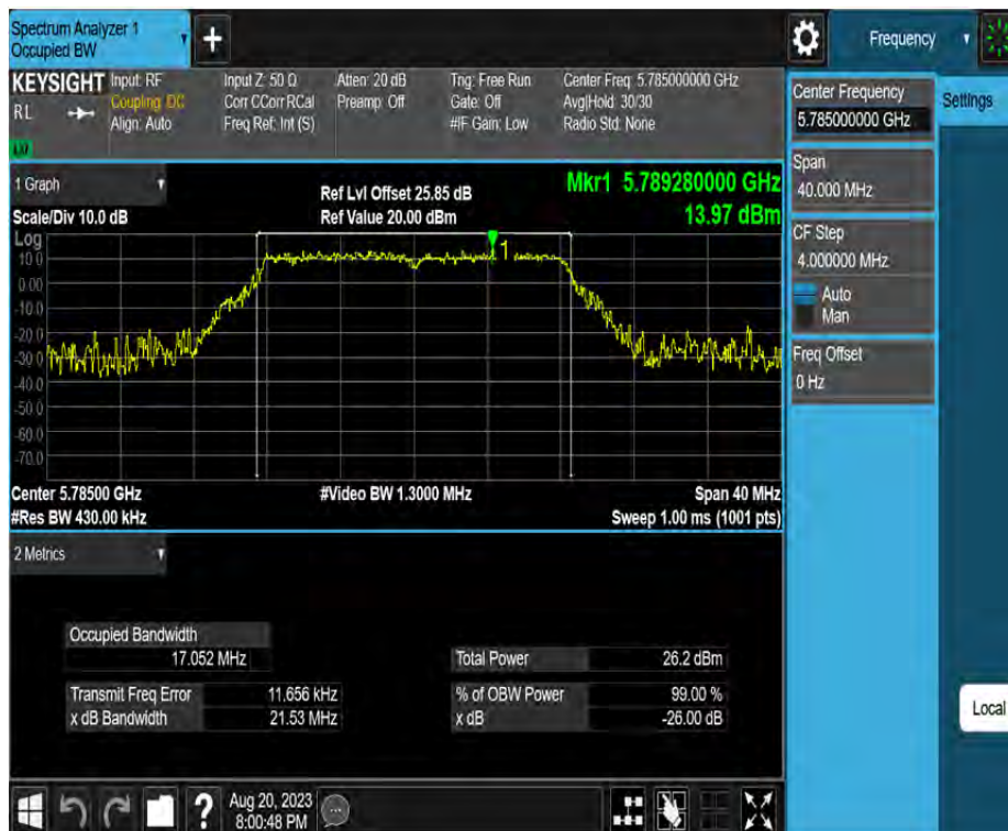
11A_Ant4_5785
