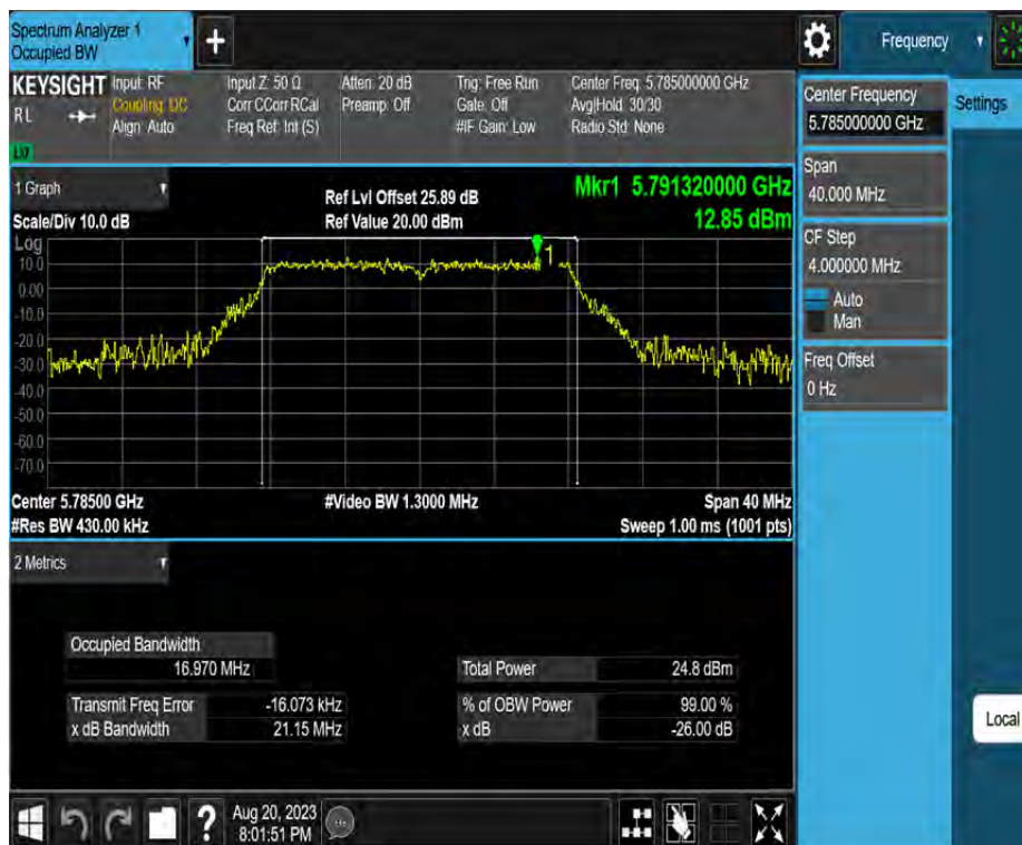
11A_Ant4_5785
