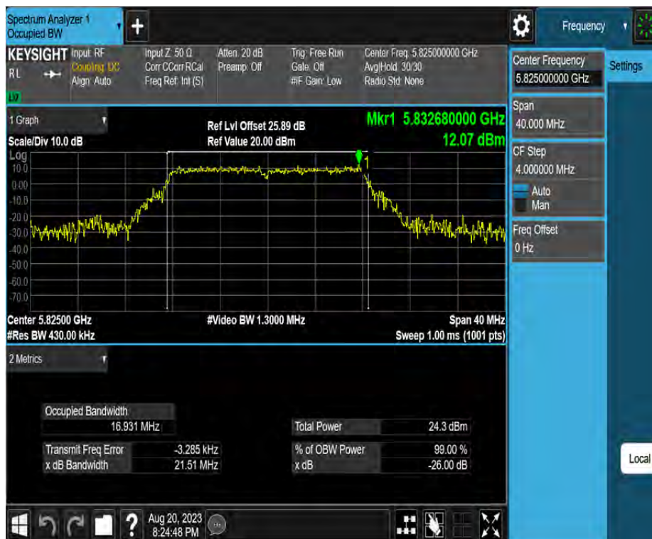
11A_Ant4_5825
