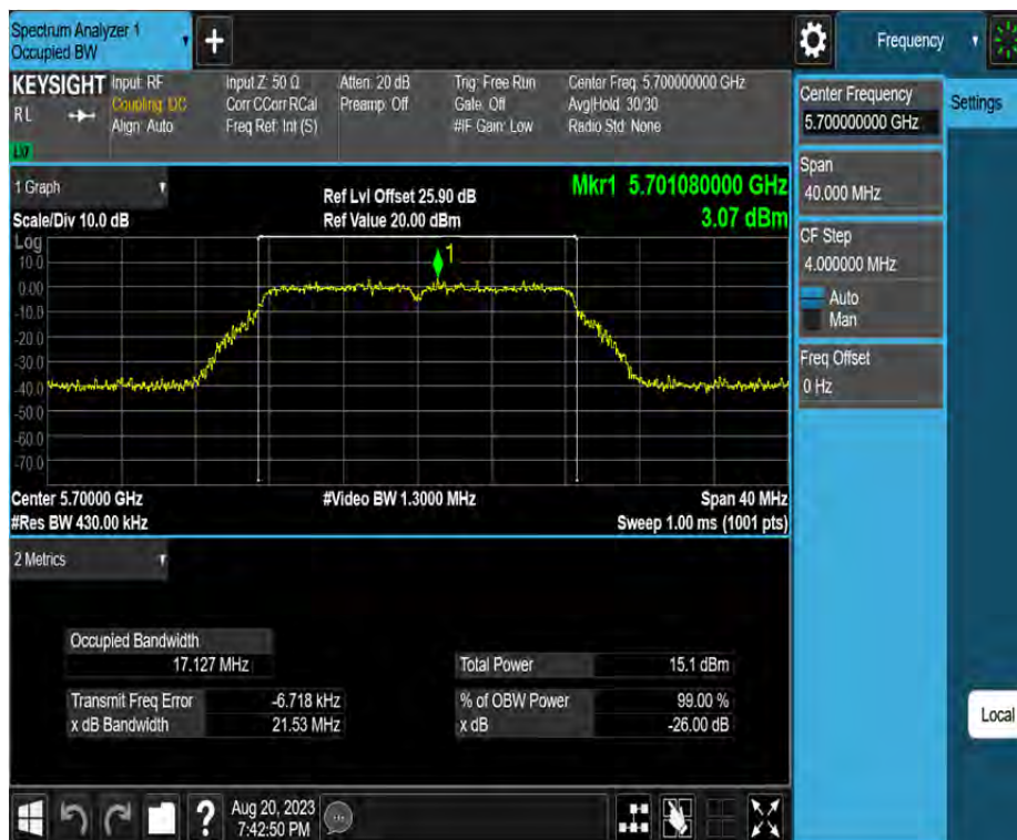
11A_Ant4_5700
