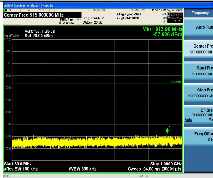
BLE_1M-Ant1-2402-30~1000-PASS
