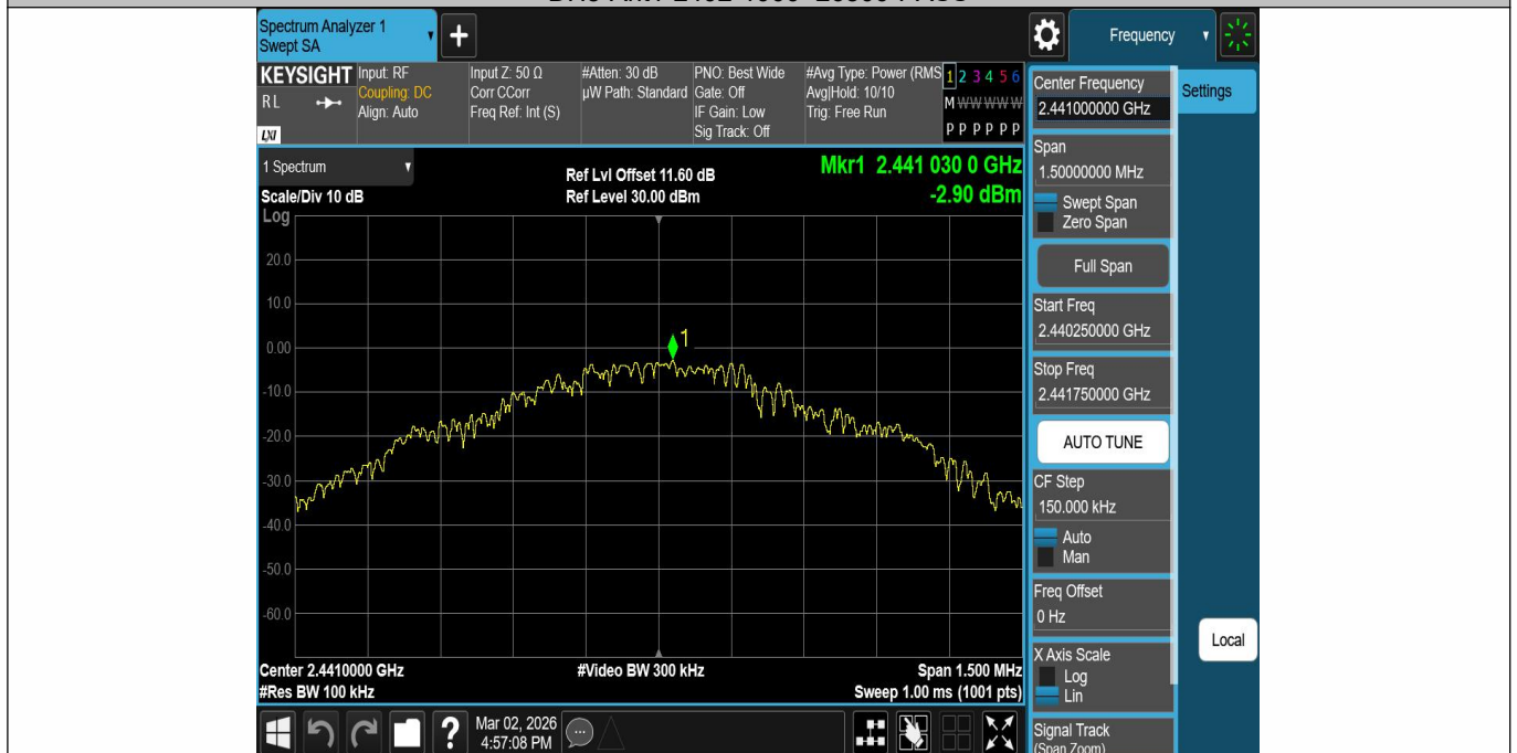
DH5-Ant1-2441-0~Reference-PASS
