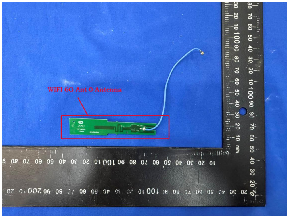
(32) EUT Photo (KCT8270HT)
