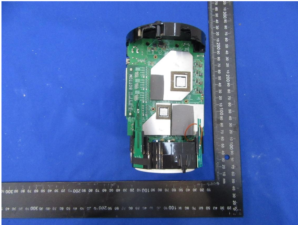
(28) EUT Photo (KCT8270HT)
