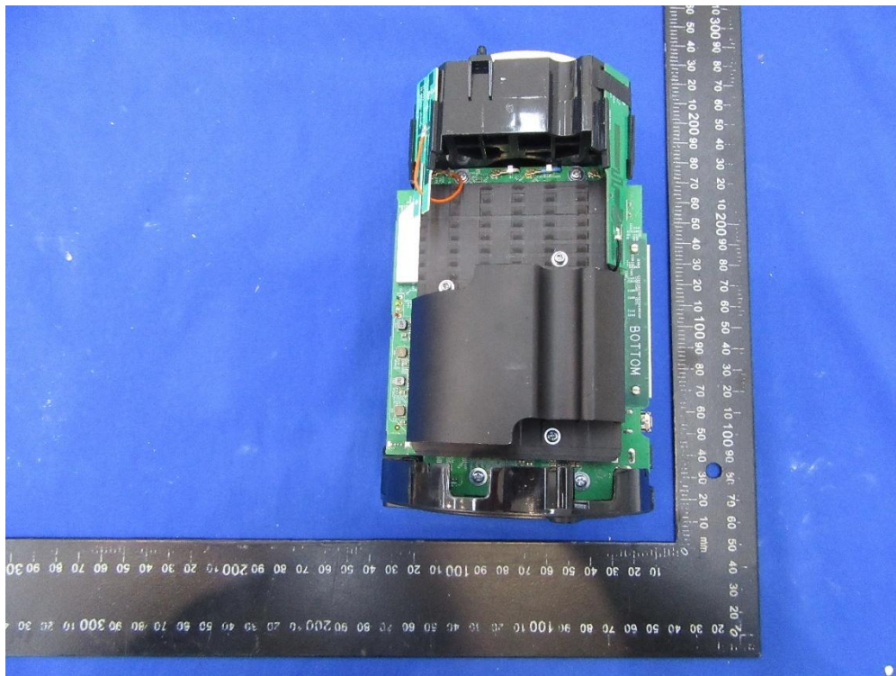
(26) EUT Photo (KCT8270HT)
