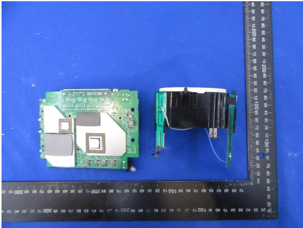
(34) EUT Photo (KCT8270HT)
