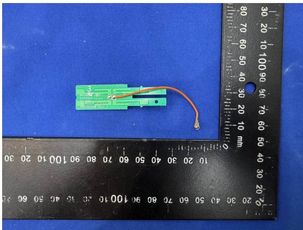
(46) EUT Photo (KCT8270HT)
