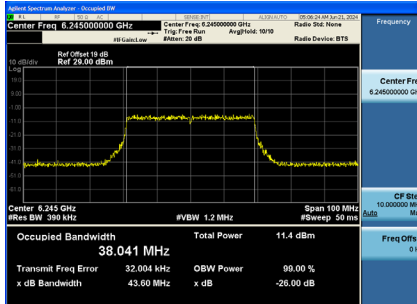
26 dB Bandwidth
