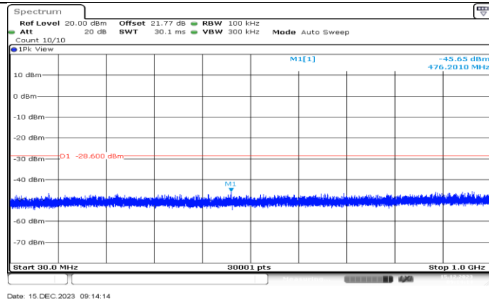
11N40MIMO Ant2 2422 30~1000
