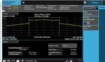
CH122 26 dB Bandwidth
