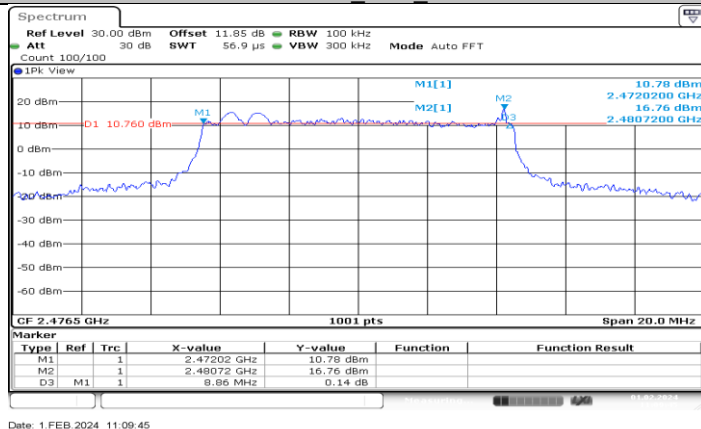
SRD 10MHz_Ant2_2476.5
