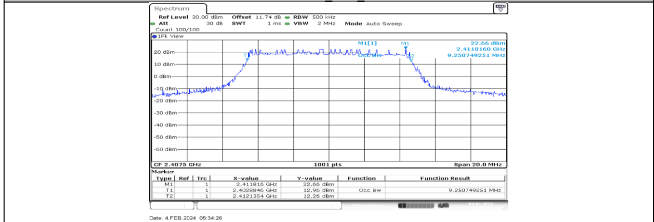
SRD 10MHz_Ant1_2407.5
