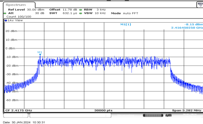
SRD 3MHz_Ant1_2417.5
