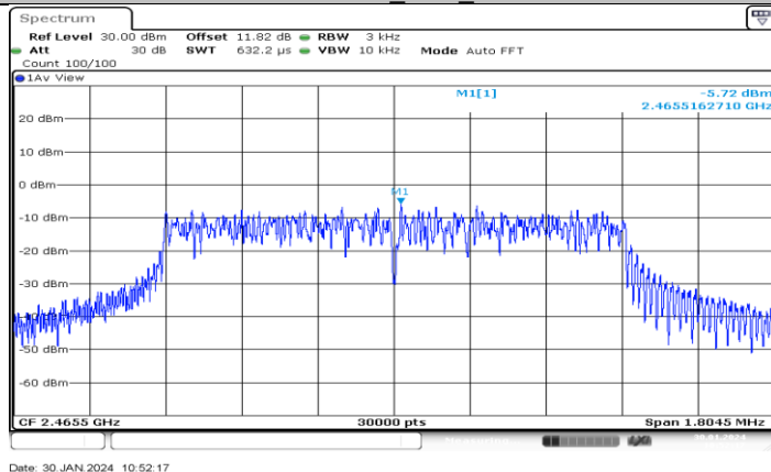
SRD 1.4MHz_Ant2_2465.5
