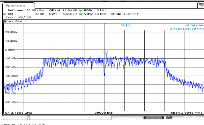
SRD 1.4MHz_Ant1_2465.5
