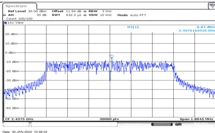
SRD 1.4MHz_Ant2_2437.5
