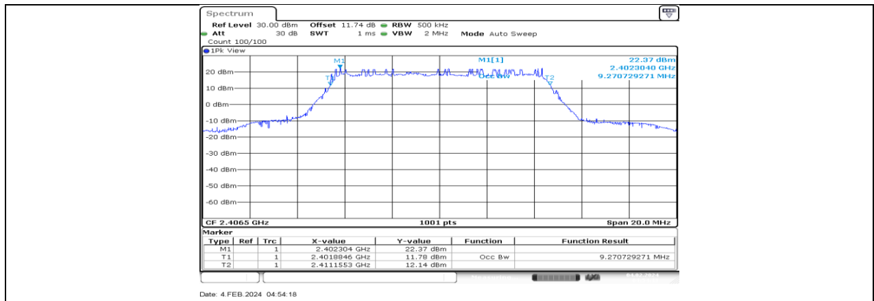
SRD 10MHz_Ant1_2406.5
