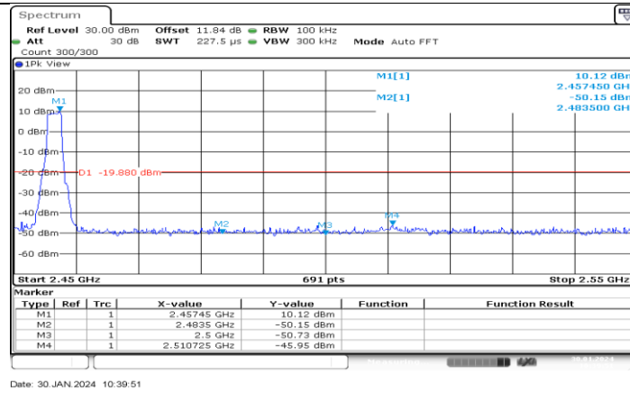
SRD 3MHz_Ant1_High_2456.5
