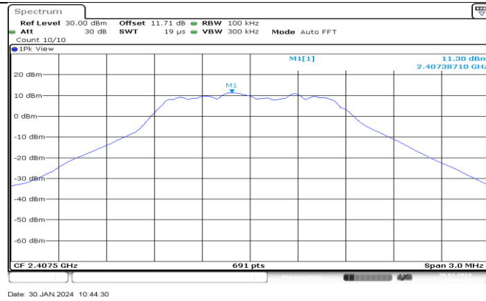
SRD 1.4MHZ_Ant2_2407.5_0~Reference
