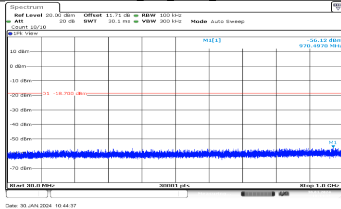
SRD 1.4MHZ_Ant2_2407.5_30~1000
