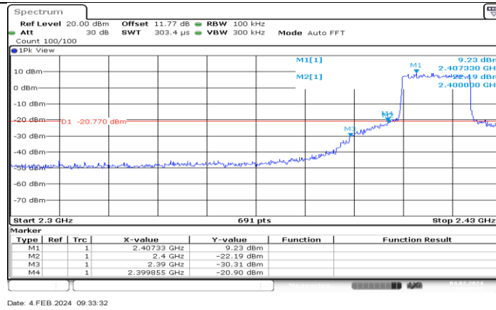
SRD 20MHz_Ant2_Low_2412.5
