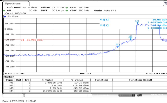
SRD 20MHz_Ant2_Low_2413.5
