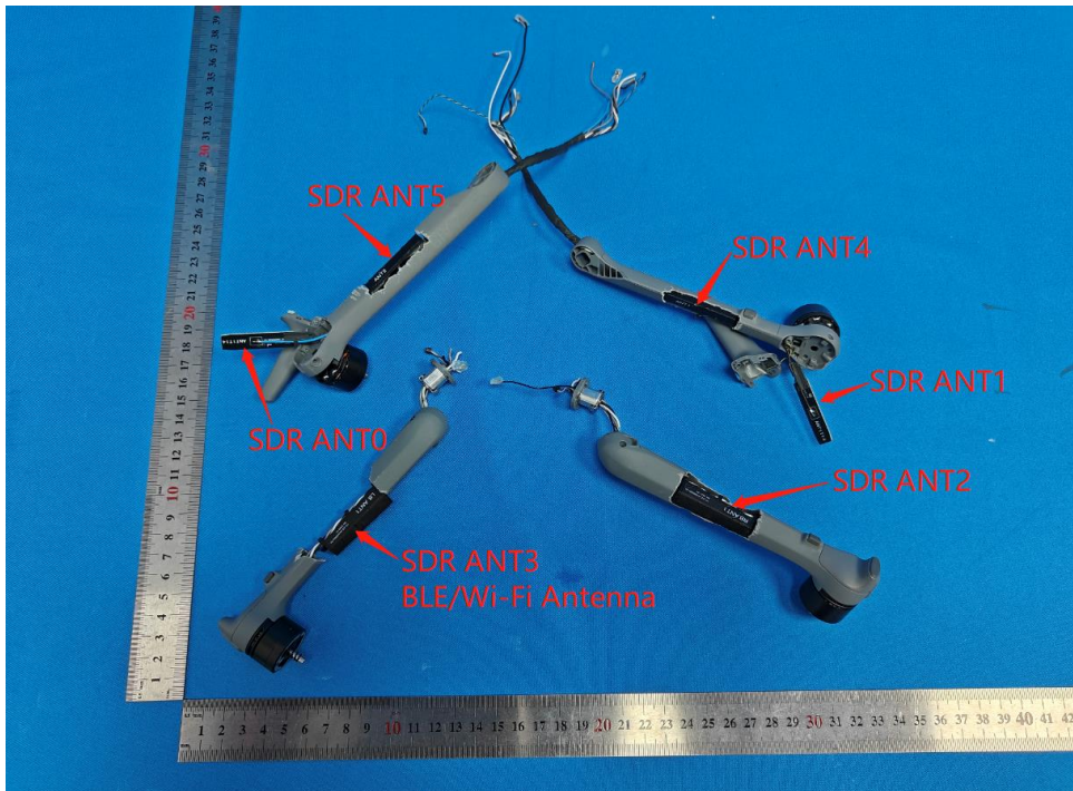
Antenna Location
