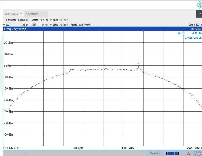
BLE_2M_Ant1_2402_0~Reference
